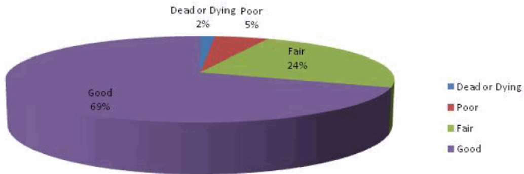
Figure 3: Foliage Condition
