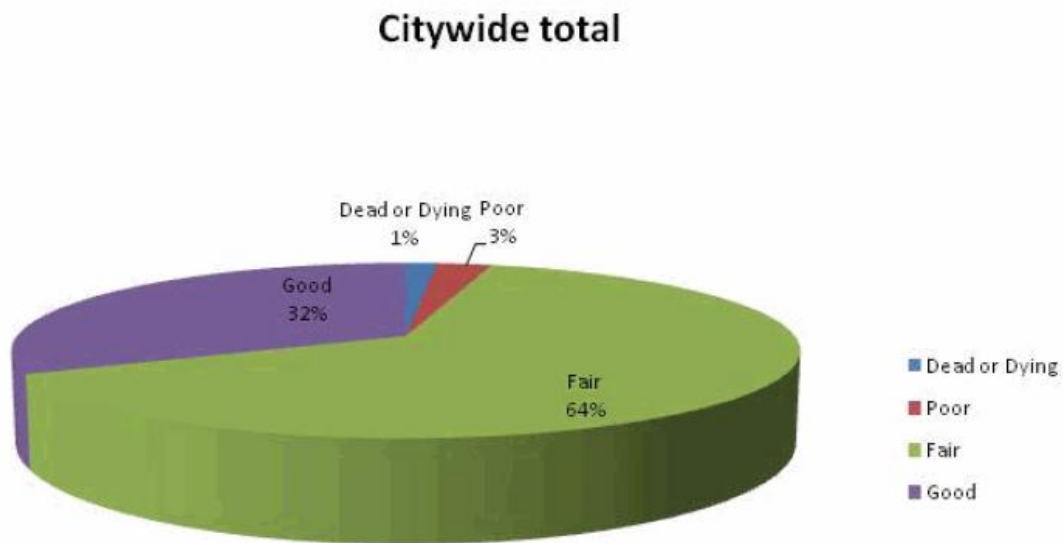
Figure 3: Foliage Condition
