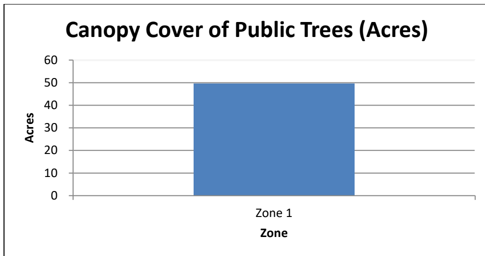
Figure 5: Canopy Cover in Acres
