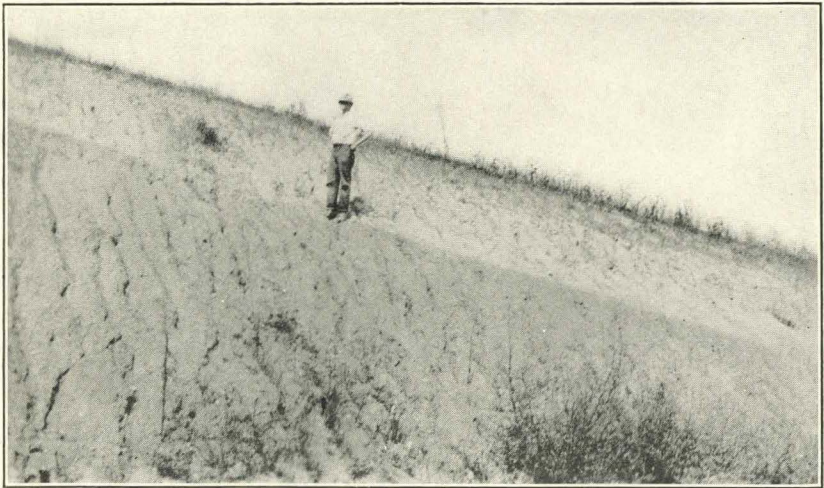
FIG. 2.—SECTION IN RAILROAD CUT EAST OF LOST NATION, SHOWING DISTINCT LINE OF DEMARCATION BETWEEN THE LOESS AND THE UNDERLYING KANSAN DRIFT, THE LOESS LAYER FOLLOWING THE CONTOUR OF THE RIDGE.
