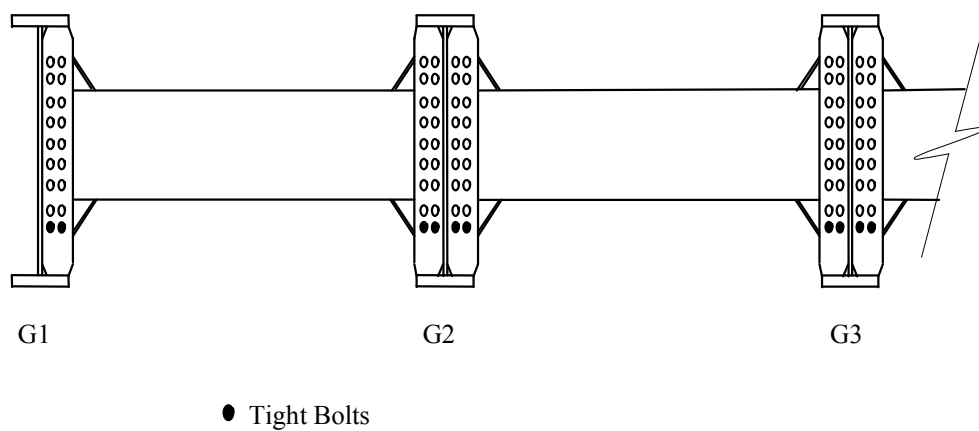
Figure 2.18. Illustration of bolt loosening condition with bottom row tight.
