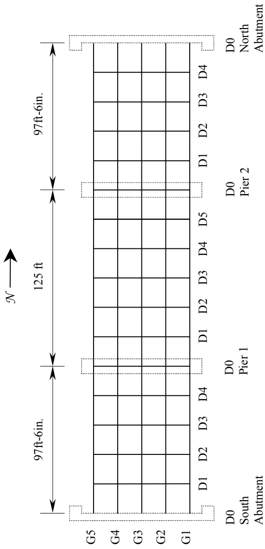
Figure 4.2. Plan view illustration of bridge superstructure.
