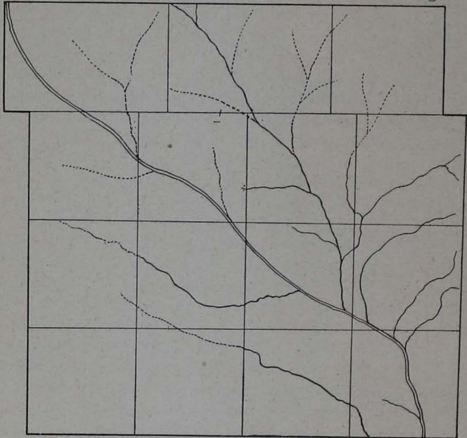
FIG. 32. Sketch map exhibiting the pre-Wisconsin drainage system, somewhat diagrammatic.
