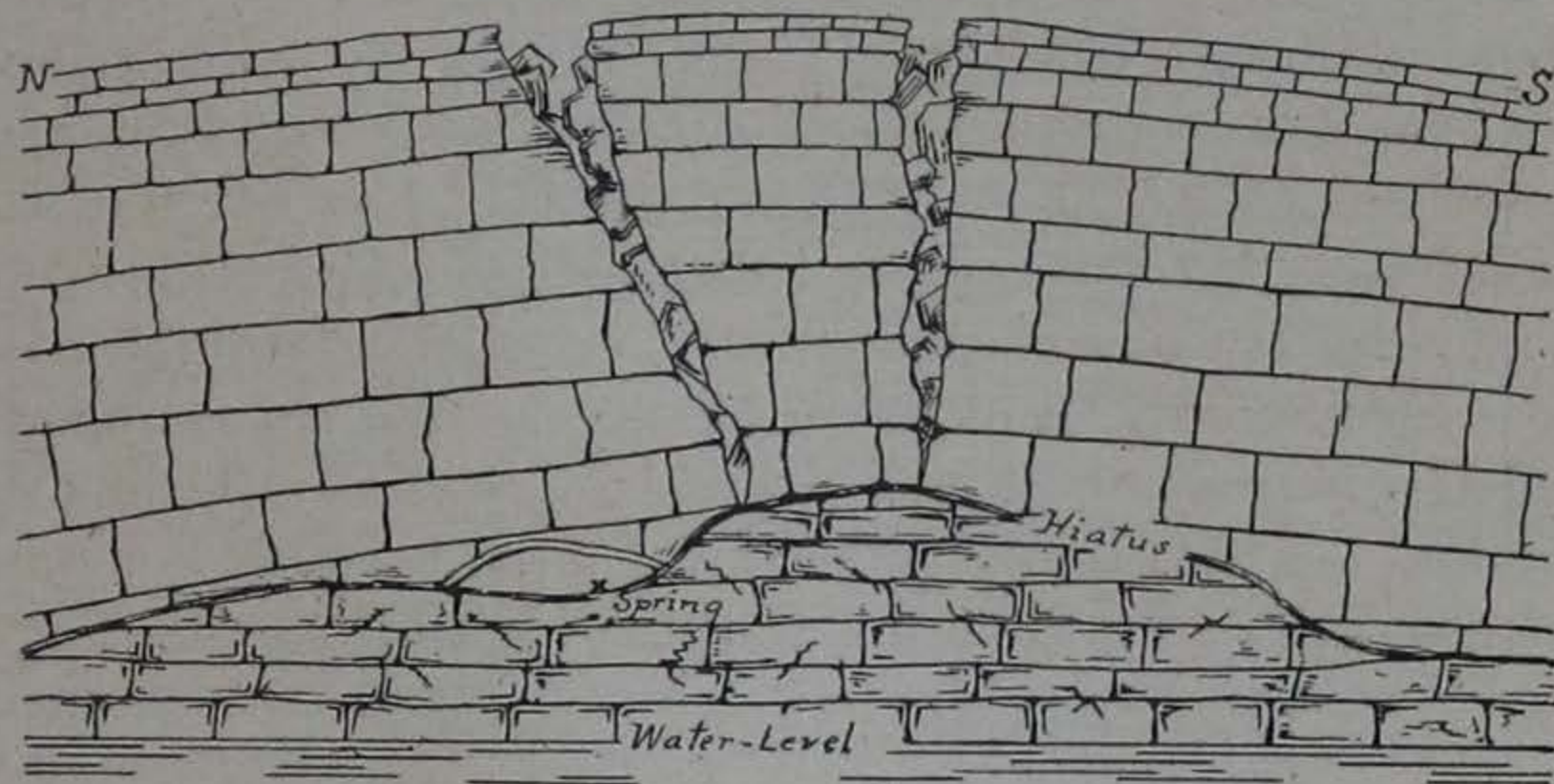
FIG. 28. Section at Ivanhoe quarry showing the local unconformity and the shattering of the upper beds.
