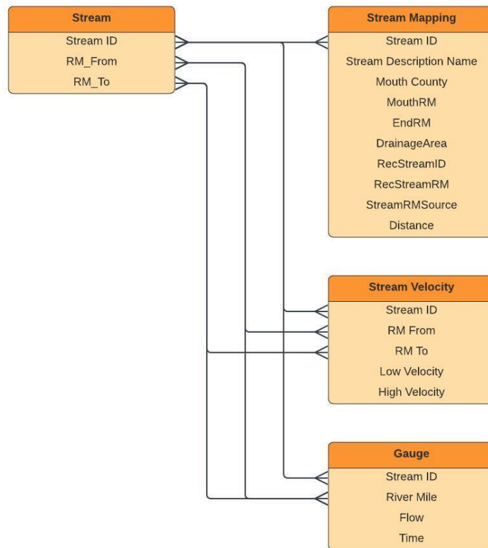
Figure 5. Entity relationship diagram of stream tables
