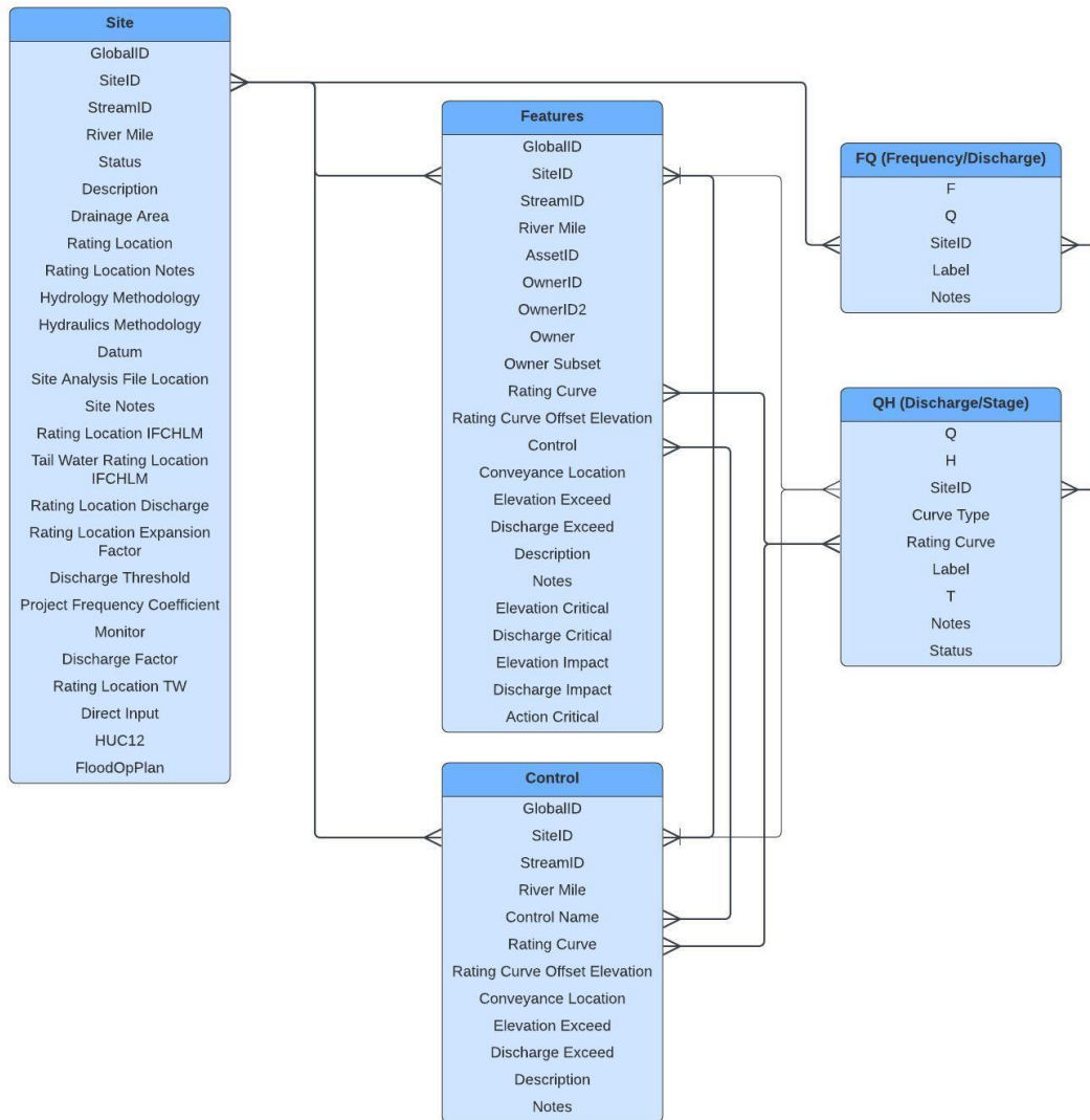
Figure 6. Entity relationship diagram of infrastructure tables
