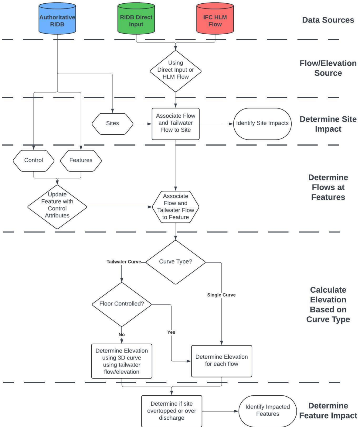
Figure 13. Hydraulic analysis flow chart
