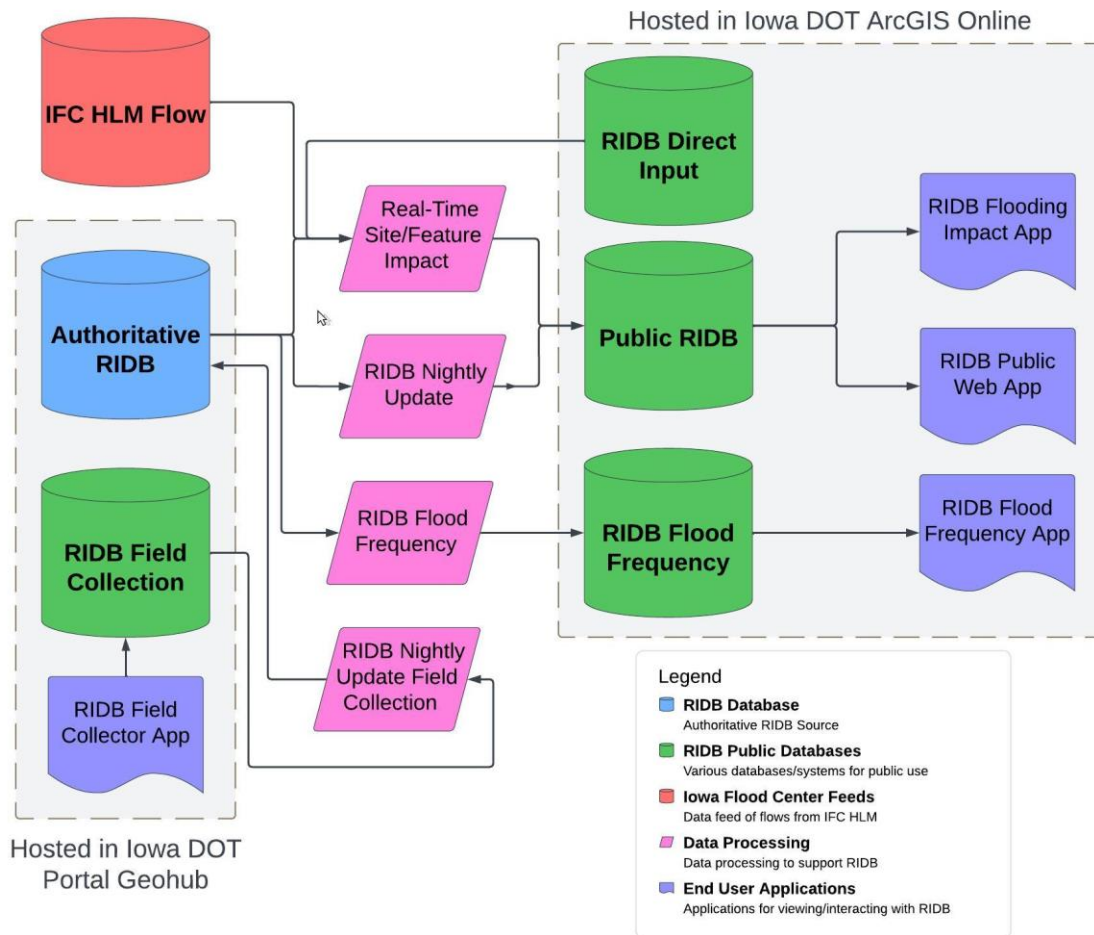
Figure 8. Overview of systems architecture for RIDB
