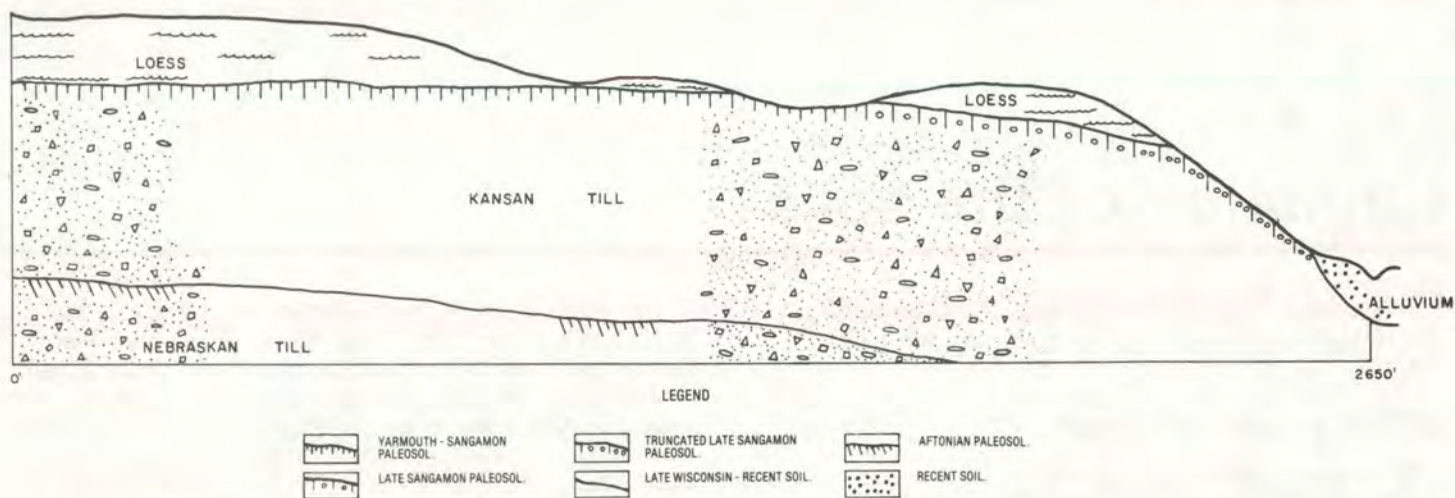
Figure 13.—Geomorphic profile traverse shows the relationship of Yarmouth Sangamon surface to the Late Sangamon pediment.
