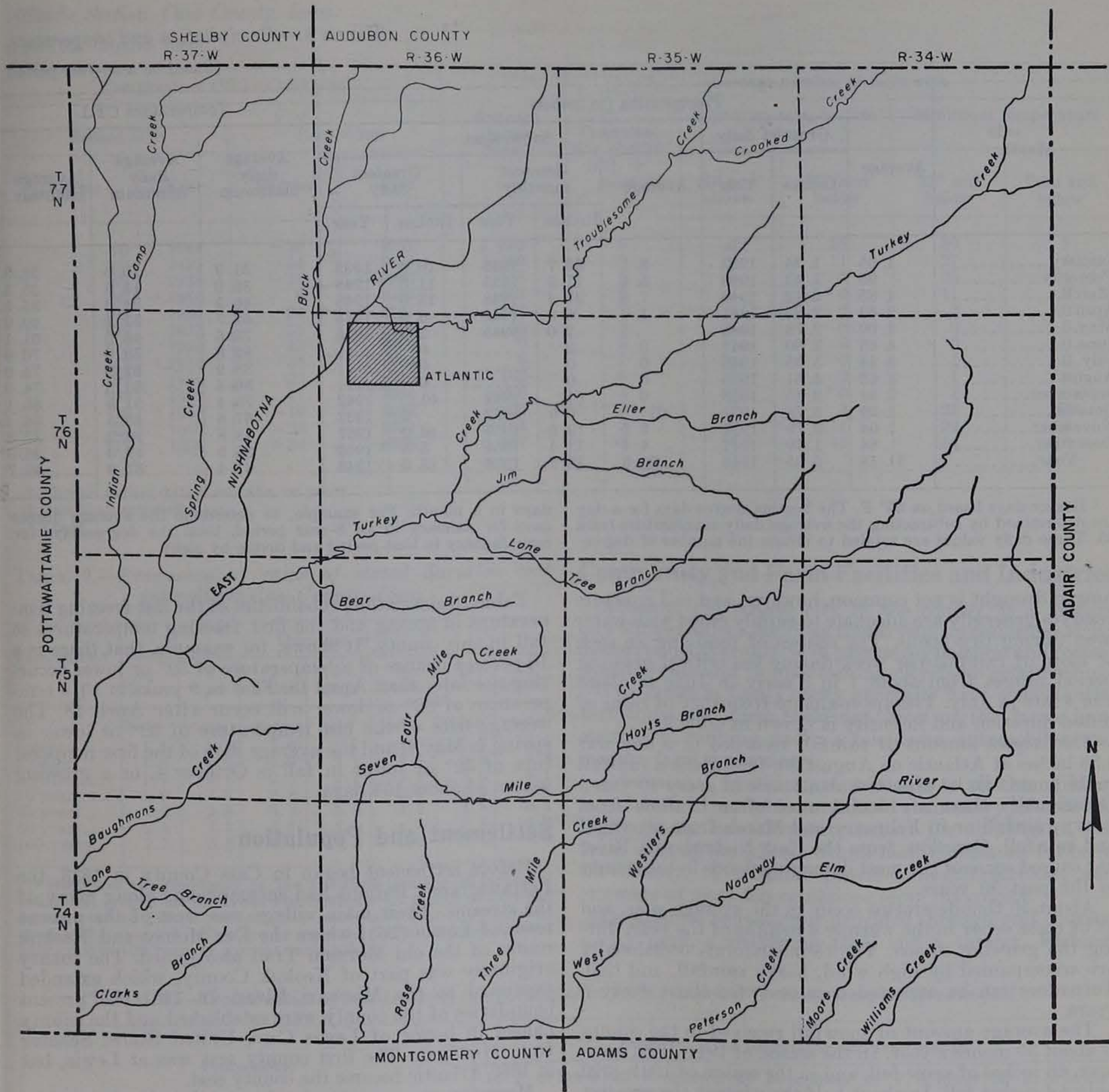
Figure 13.—Principal drainage systems in Cass County.
