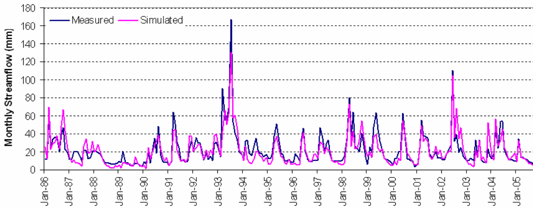
FIGURE 3. Monthly streamflow comparison at the watershed outlet
