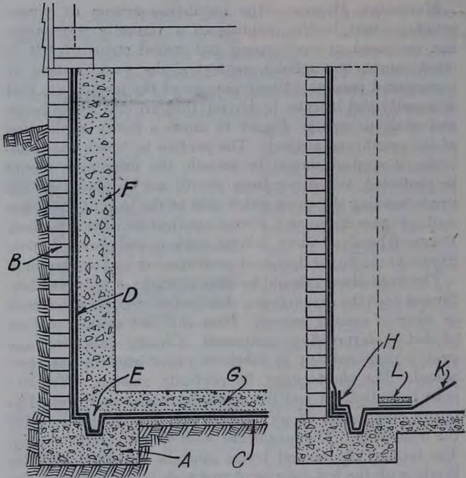
FIG. 20.—Correct Application of the Membrane Method of Waterproofing.
