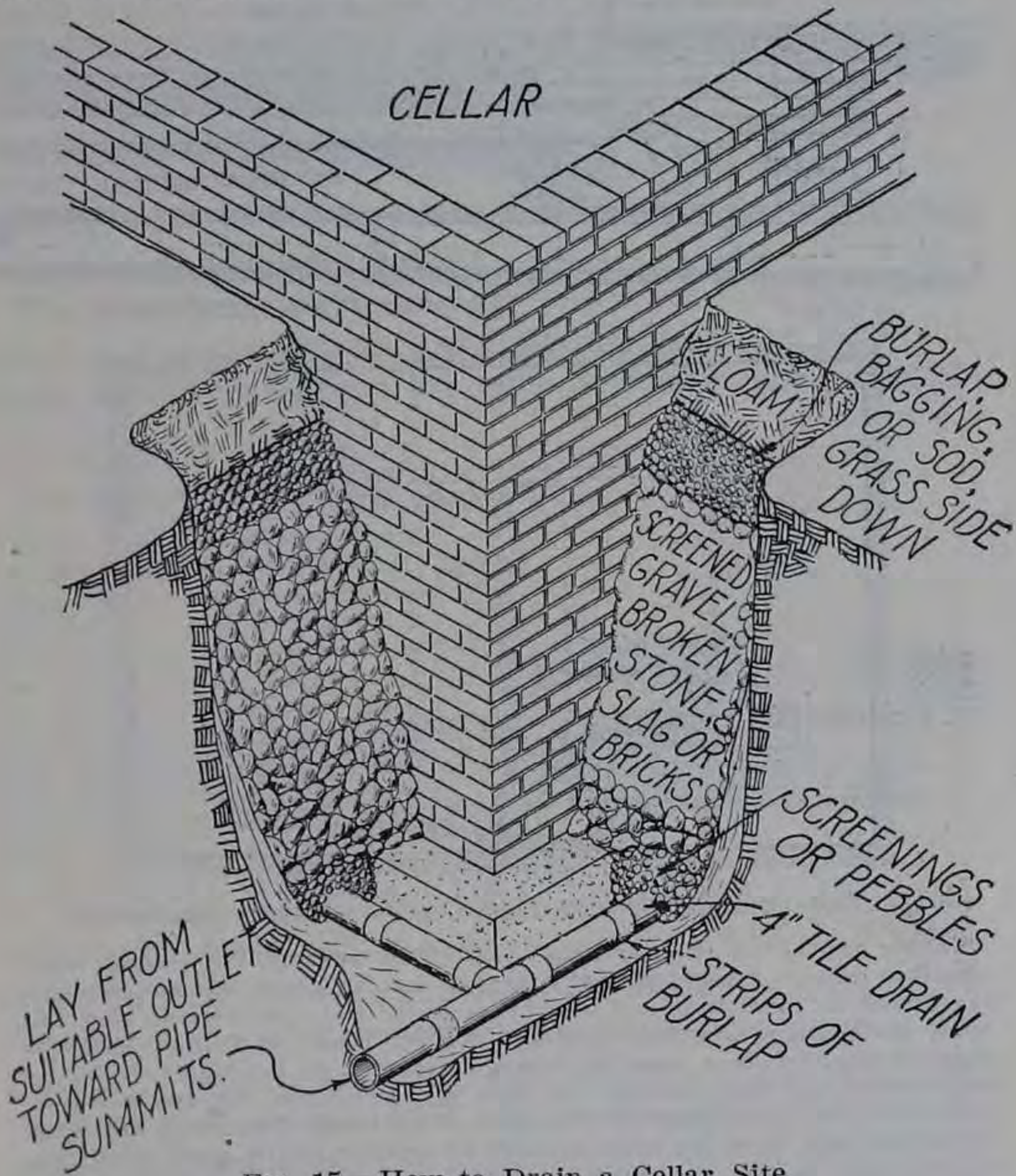
FIG. 15.—How to Drain a Cellar Site.
