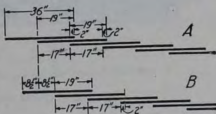
FIG. 21.—Membrane Waterproofing.
