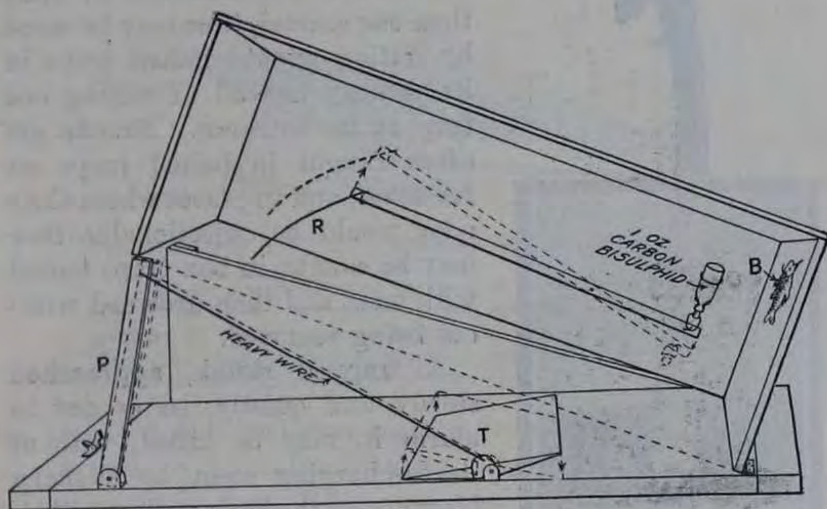
FIG. 7.—Details of Operation of Cat Trap Shown in Figure 6.
