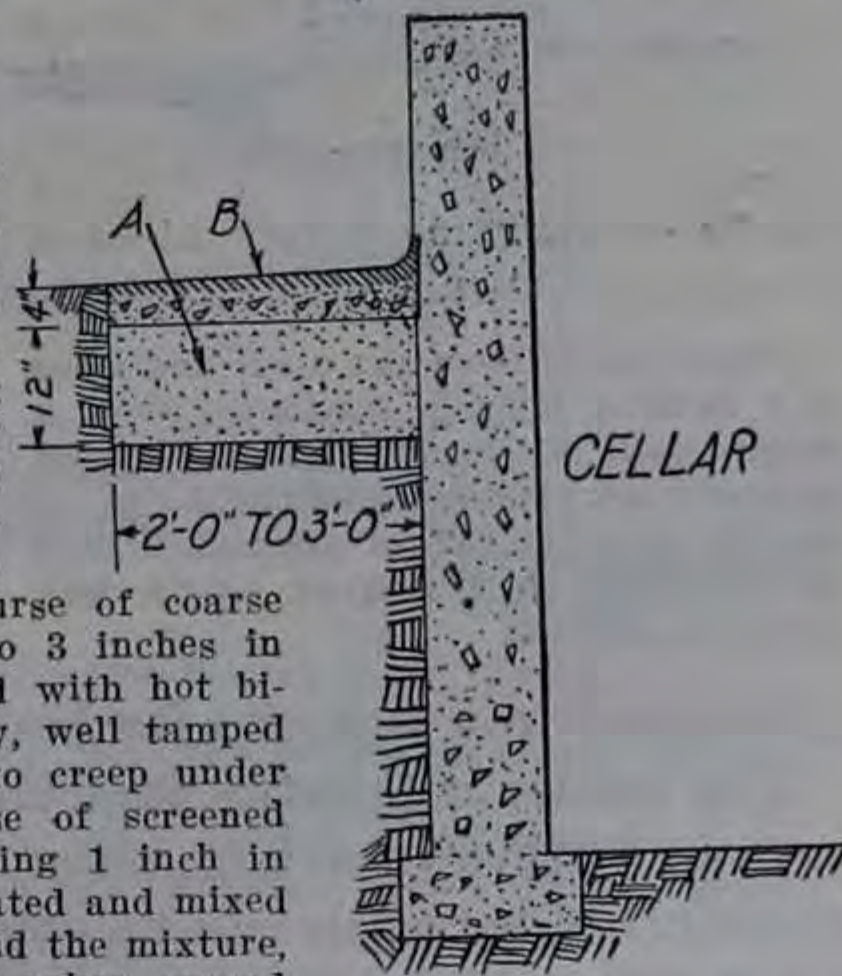
FIG. 5.—Shedding Water from Cellar Walls.
