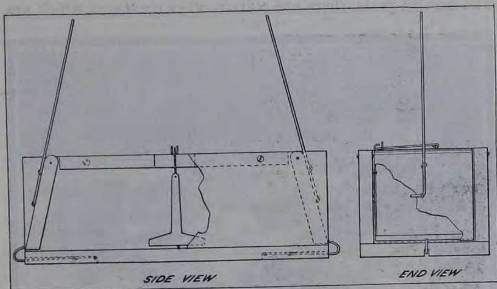
FIG. 3.—Details of Construction of Rabbit Trap Shown in Figure 2.
