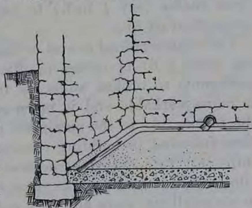
FIG. 17.—A Type of Drain that Should not be Used.
