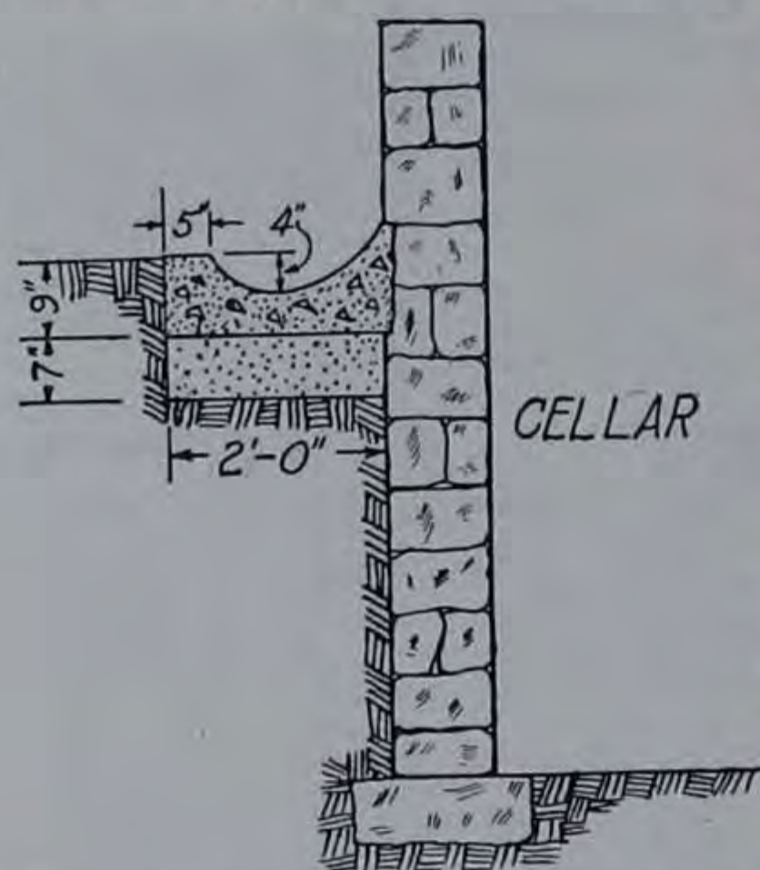
FIG. 6.—Conducting Water Along a Cellar Wall.
