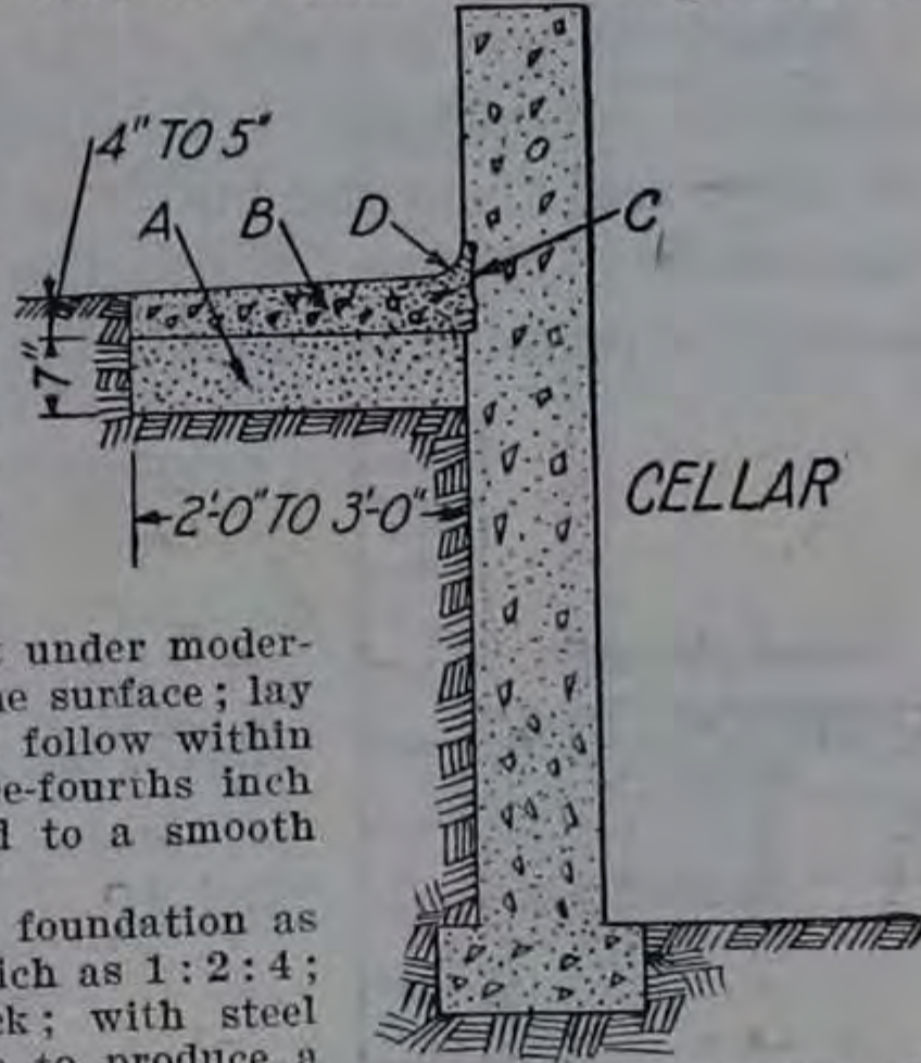
FIG. 4.—Shedding Water from Cellar Walls.
