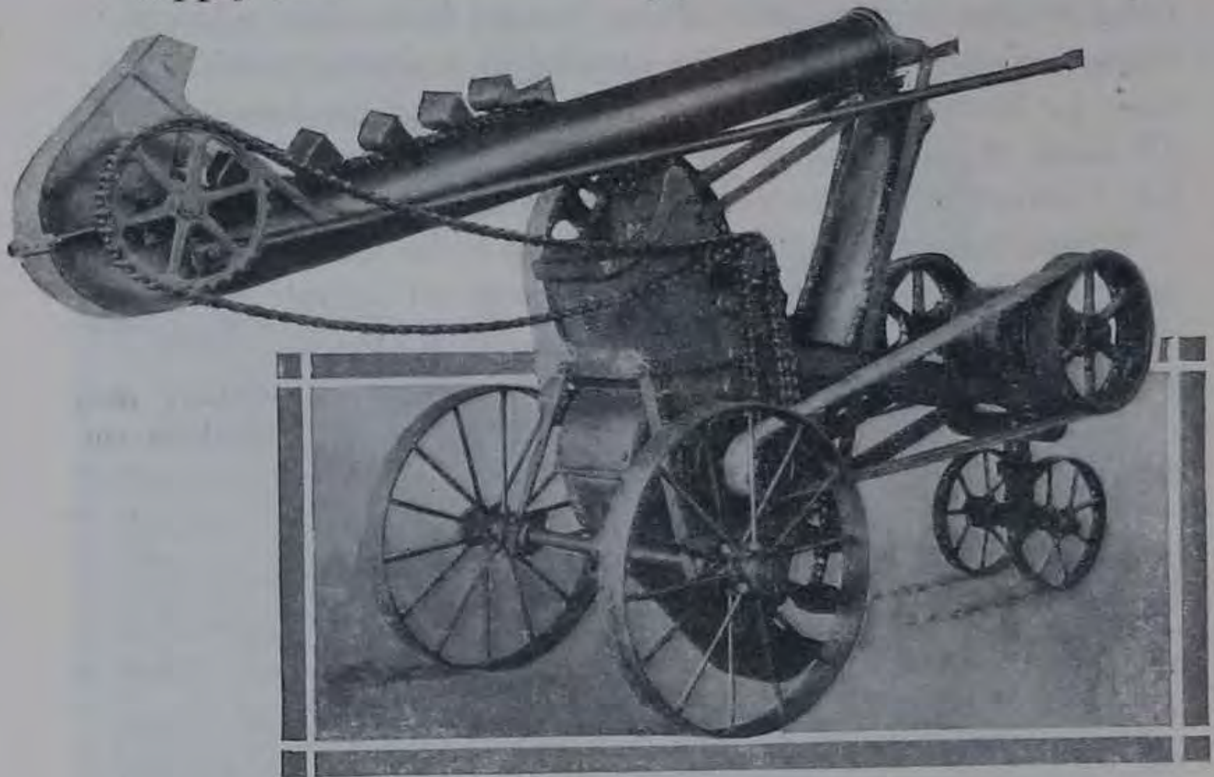
A Type of Commercial Pulverizer Showing Elevator Folded Back Ready to Move.
