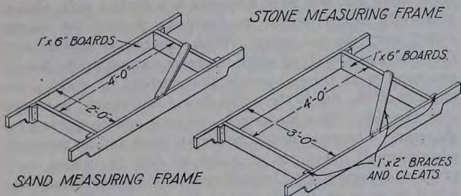
FIG. 18.—Sand and Stone Measuring Frames or Bottomless Boxes.
