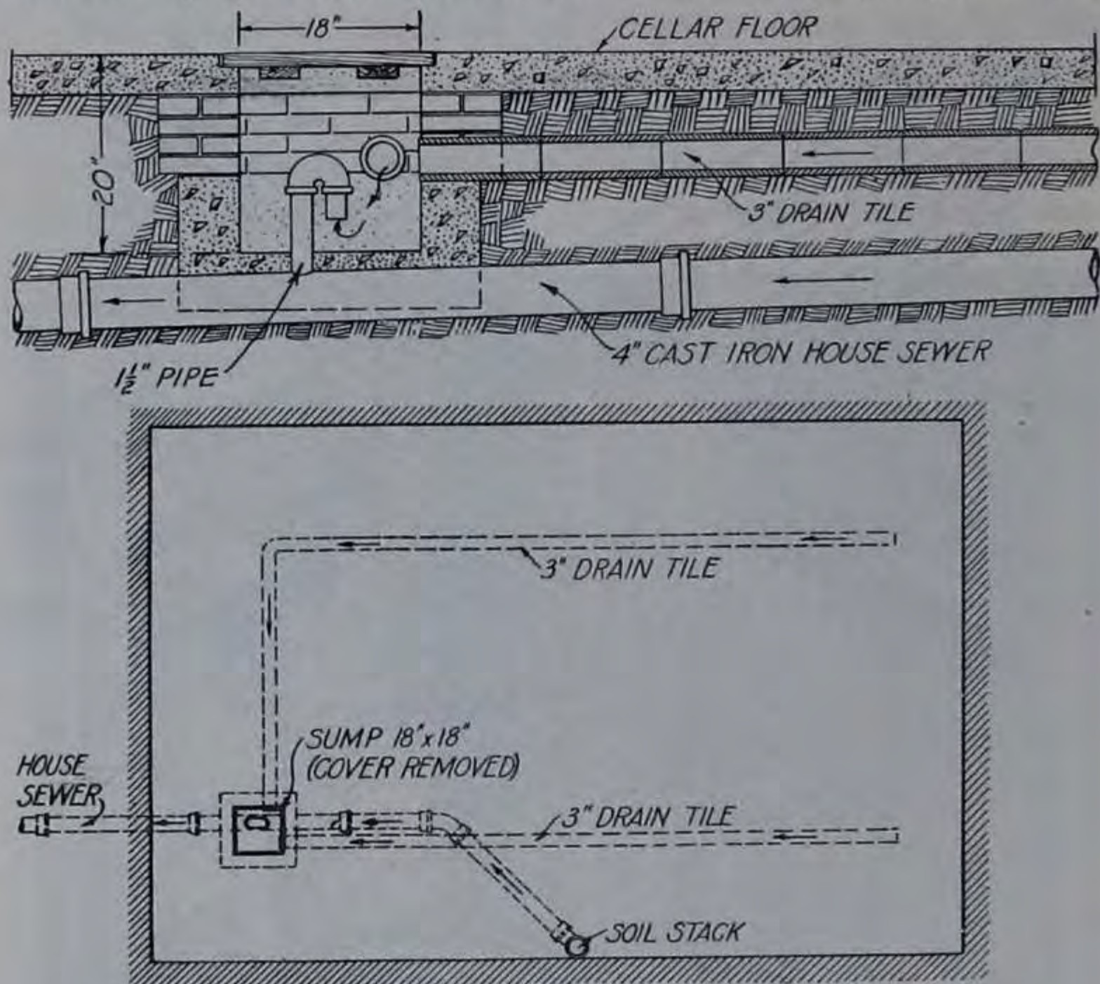
FIG. 16.—Draining through House Sewer—Rarely Advisable.
