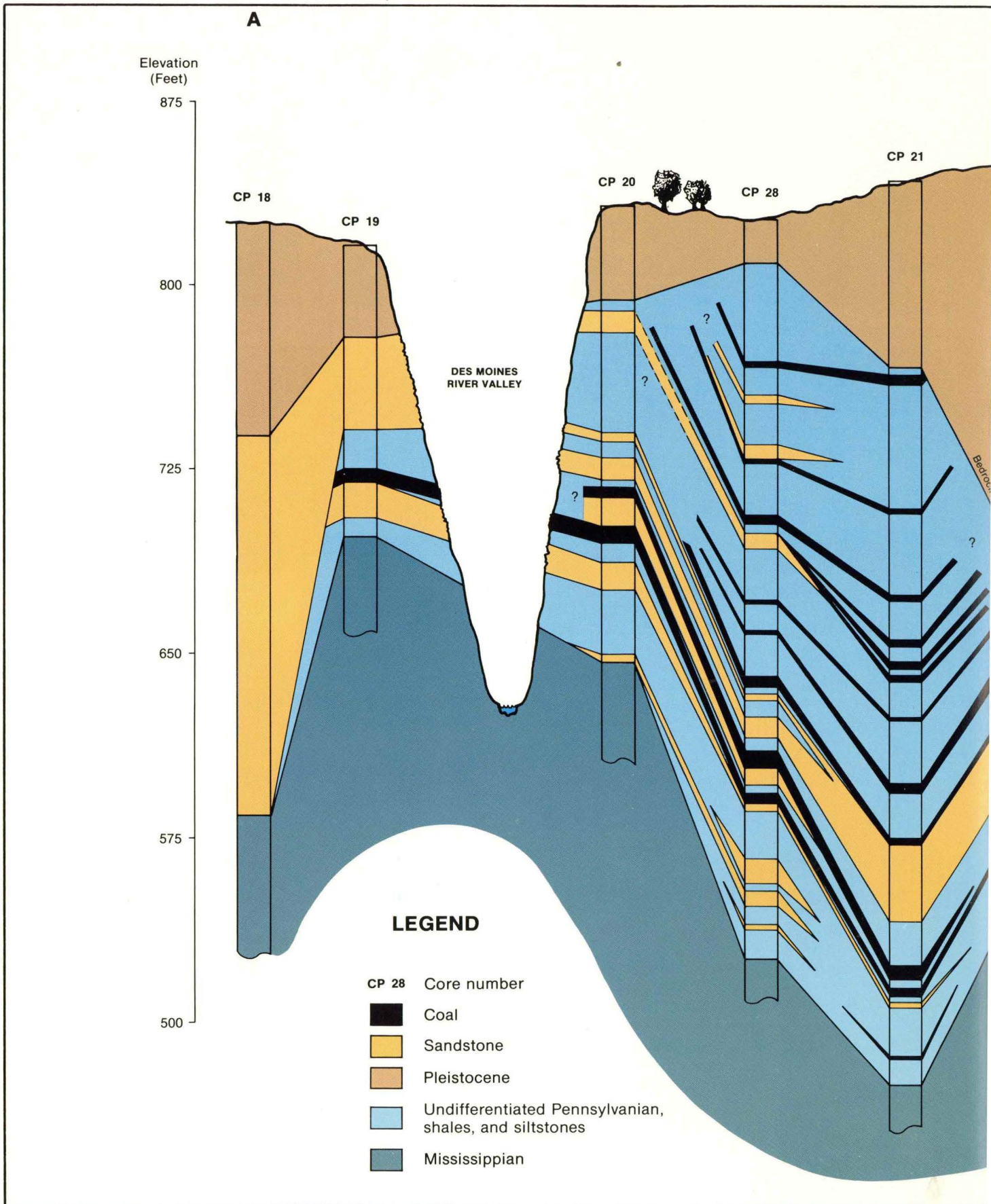
Figure 4. Cross-section A-A' illustrating a number of interrelationships common to Pennsylvanian-age rock units.
