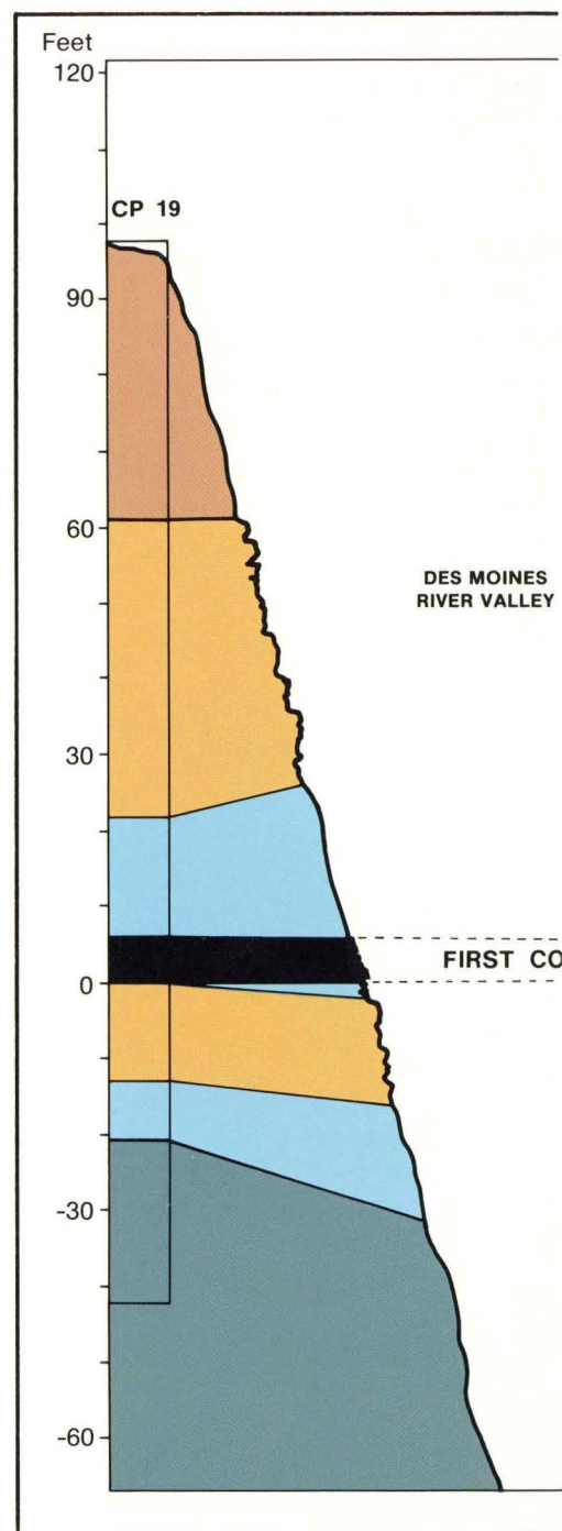
Figure 5. Expanded portion of cross-section
