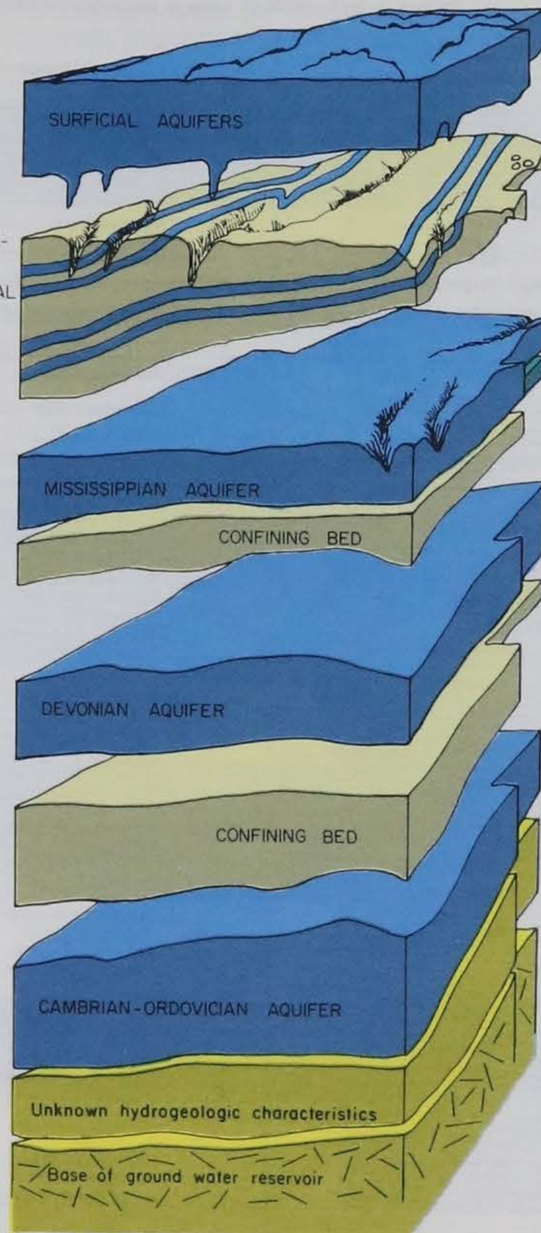
Figure 26.— The aquifers in south-central Iowa
