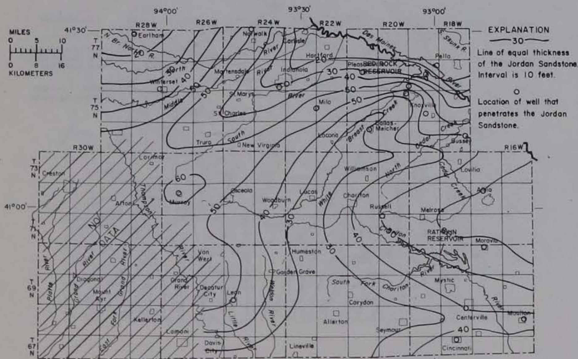
Figure 42.— Thickness of the Jordan Sandstone
