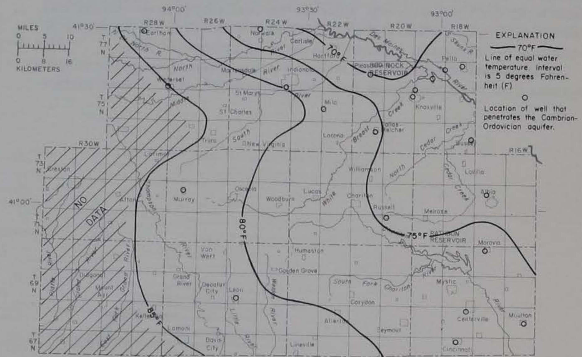
Figure 57.—Temperature of water in the Cambrian-Ordovician aquifer
