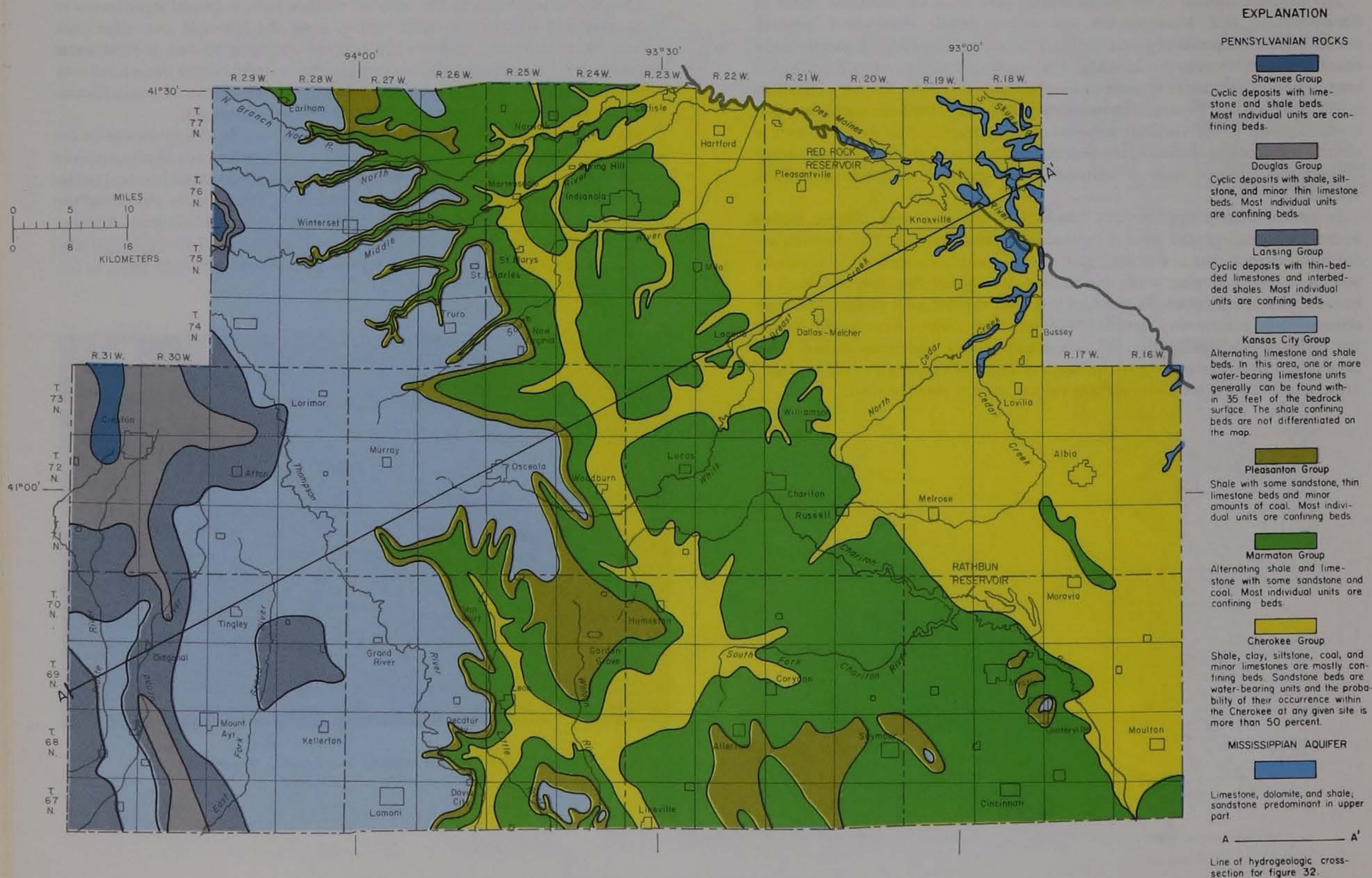
Figure 31.— Bedrock hydrogeologic map
