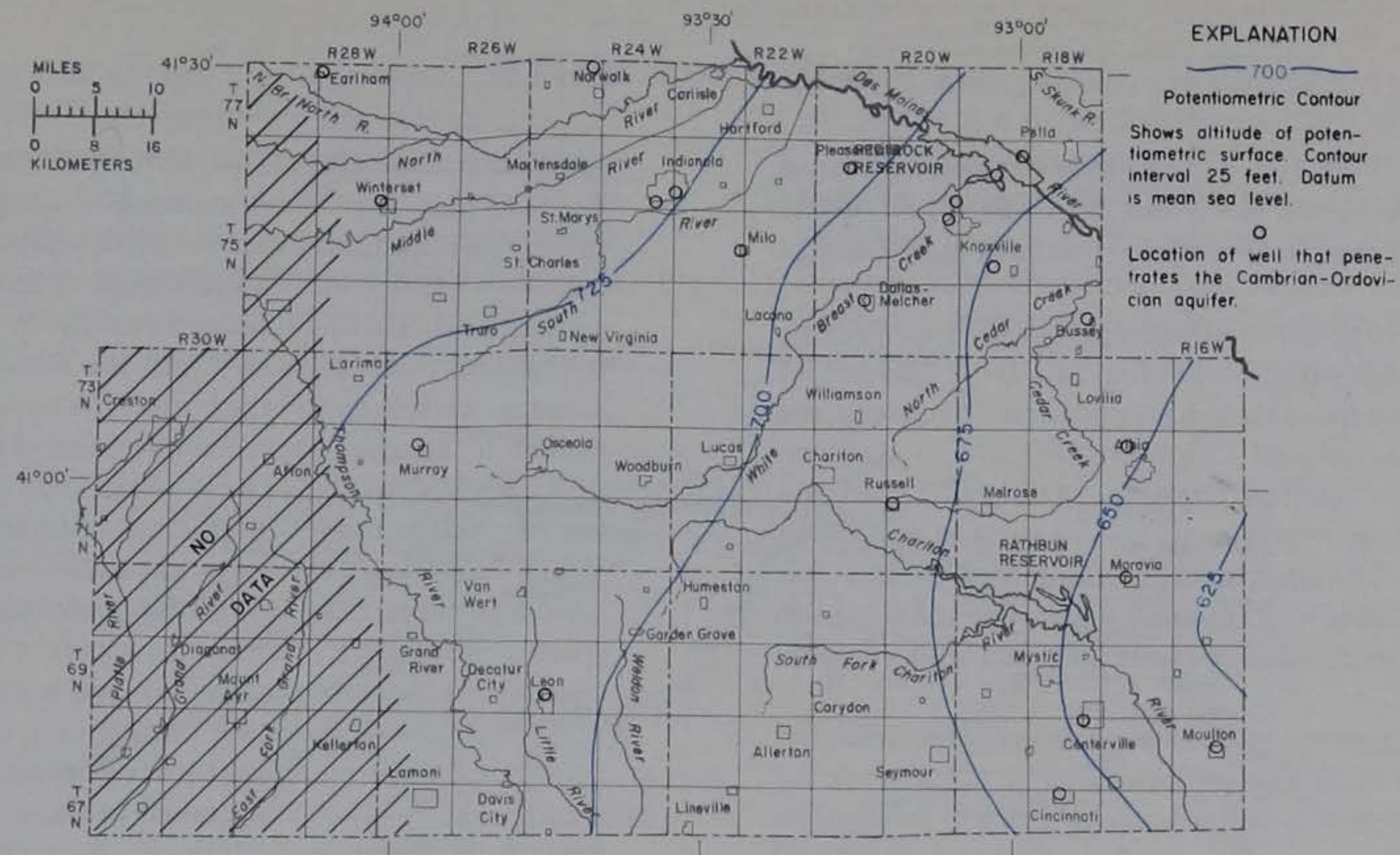
Figure 48.— Predevelopment potentiometric surface of the Cambrian-Ordovician aquifer
