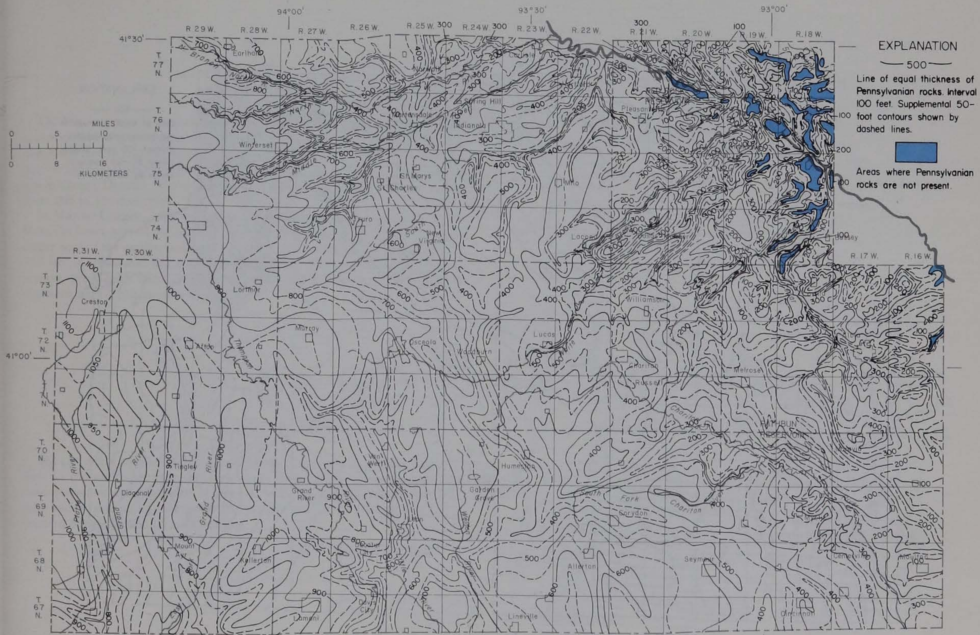
Figure 38.— Thickness of the Pennsylvania rocks
