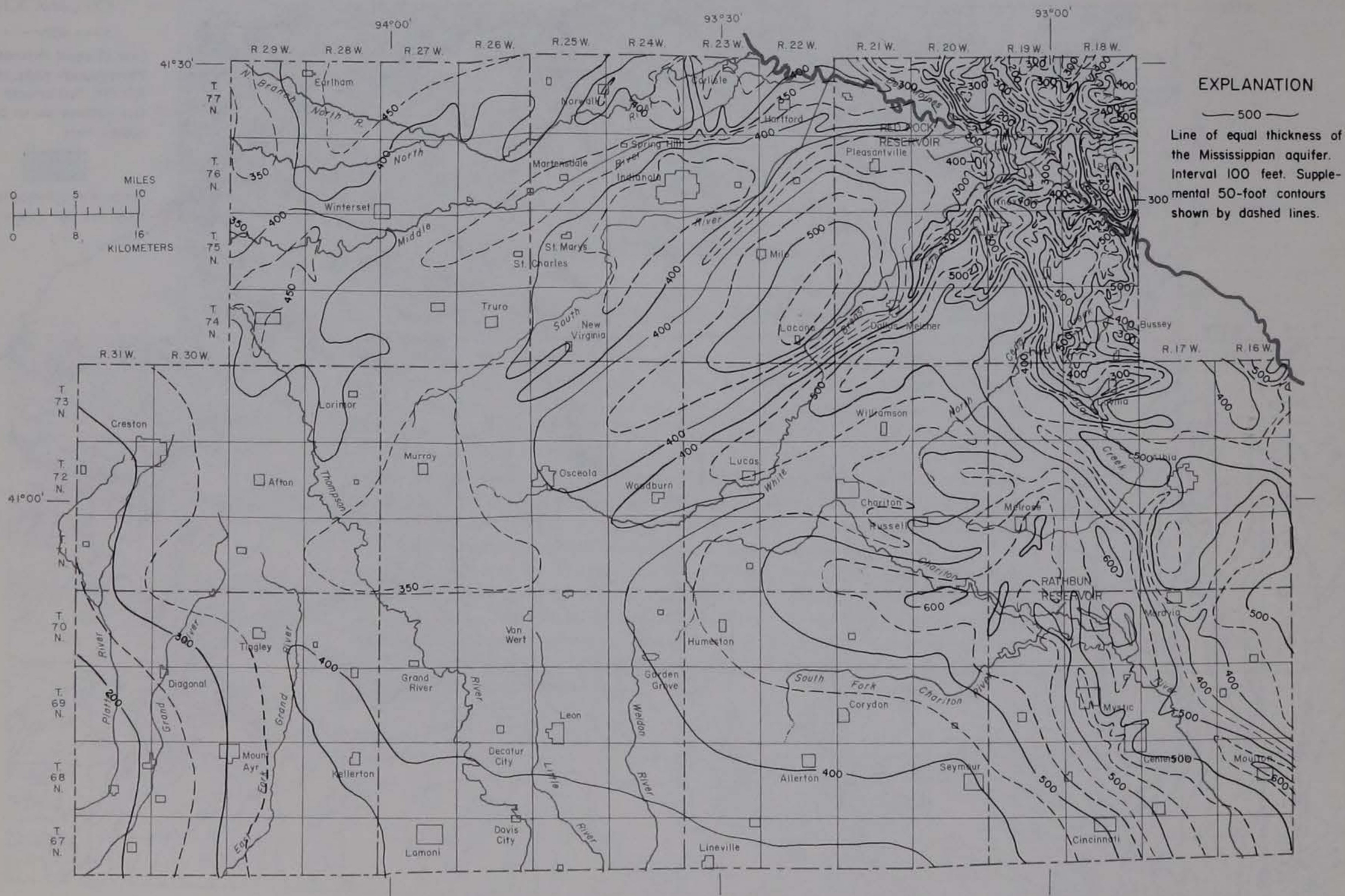
Figure 39.— Thickness of the Mississippian aquifer
