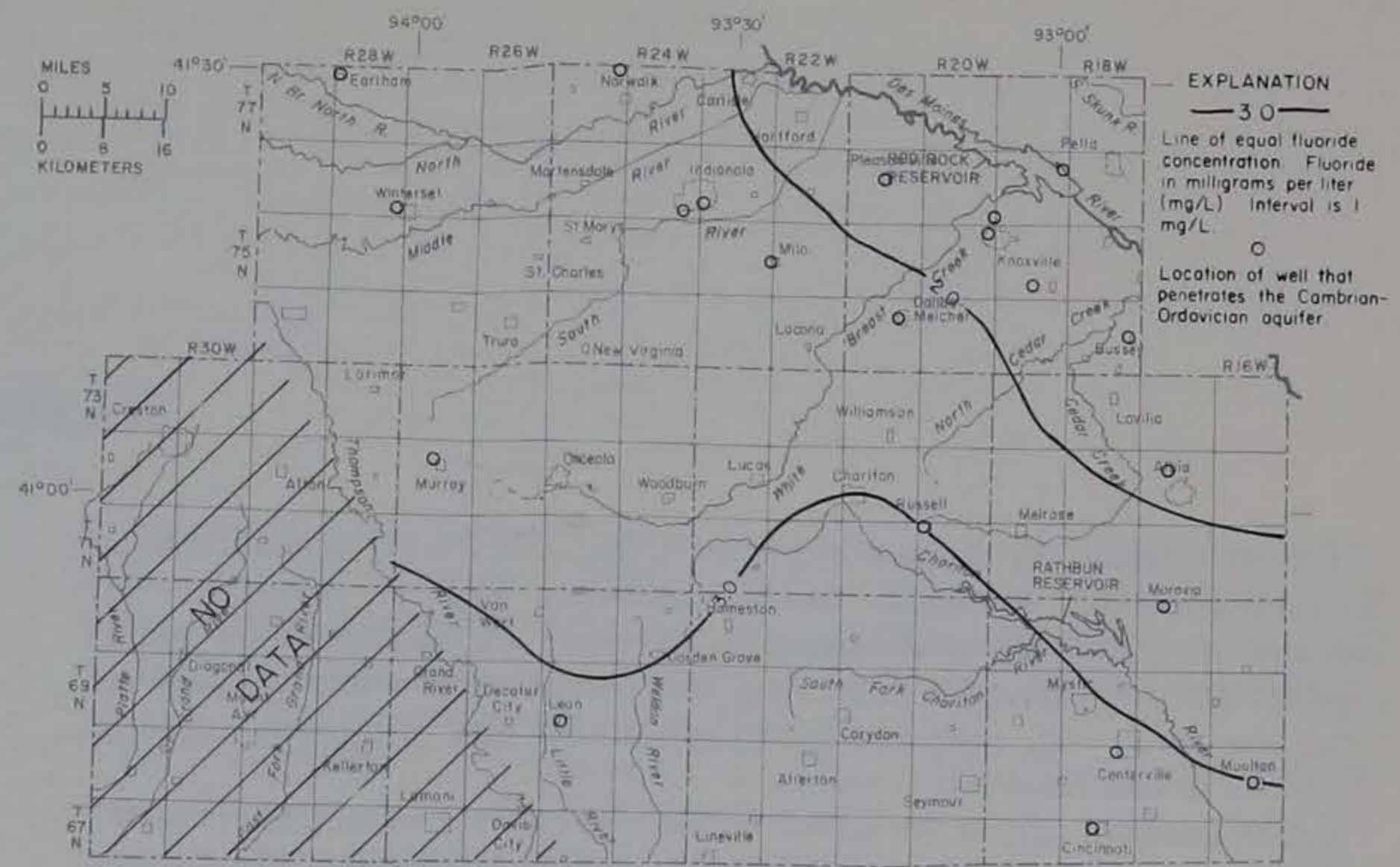
Figure 56.—Fluoride concentrations in water from the Cambrian-Ordovician aquifer
