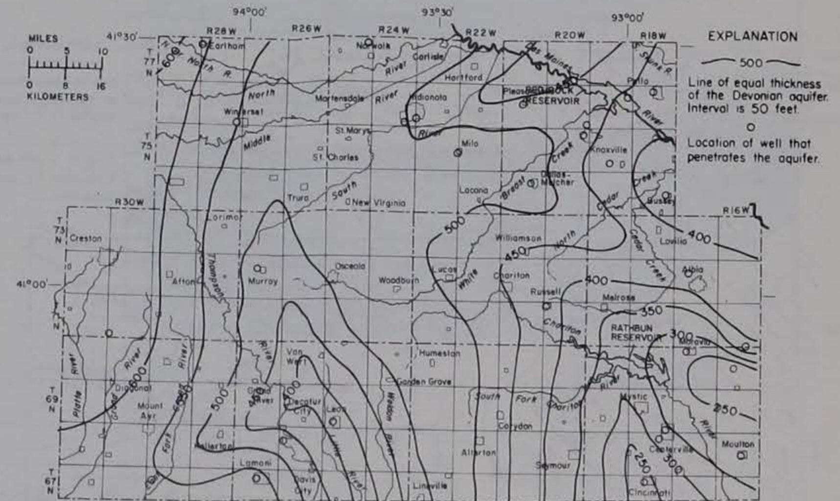
Figure 40.— Thickness of the Devonian aquifer
