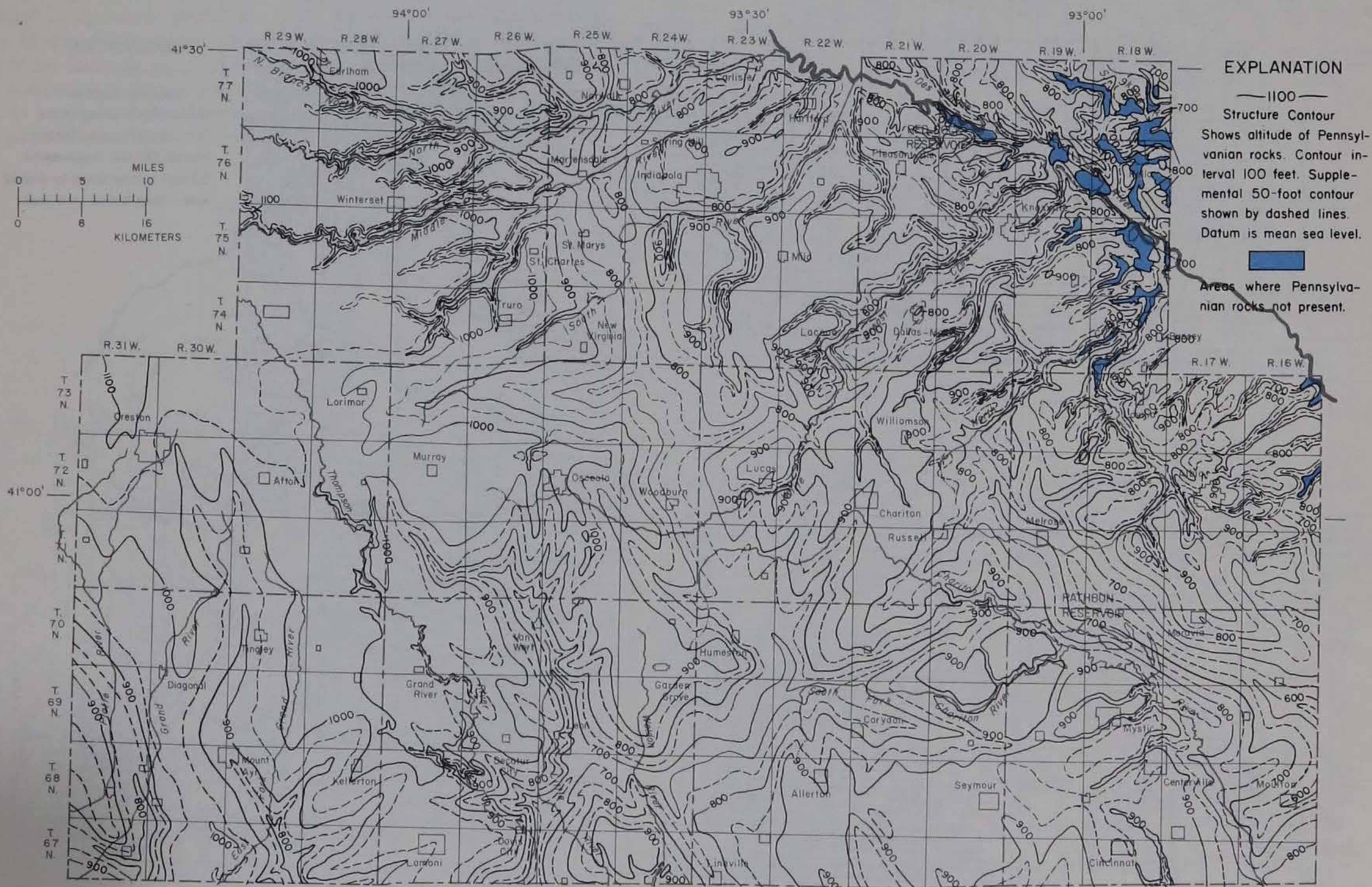
Figure 33.— Altitude of the top of the Pennsylvanian rocks
