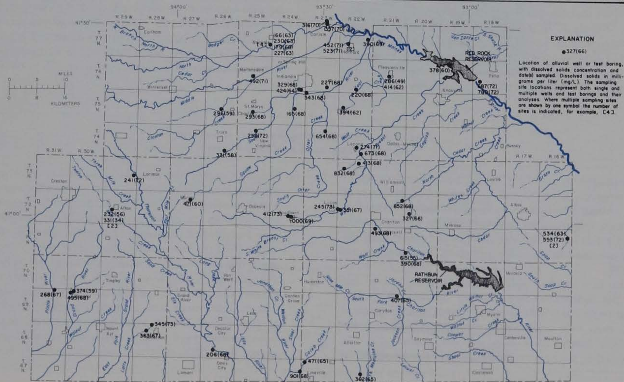
Figure 53.— Dissolved-solids concentrations in water from the alluvial aquifer
