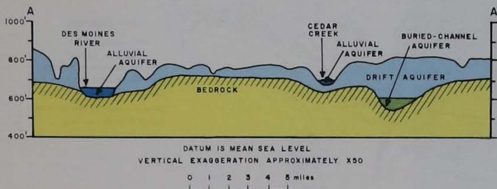
Figure 25.—Generalized hydrogeologic cross section of surficial aquifers
