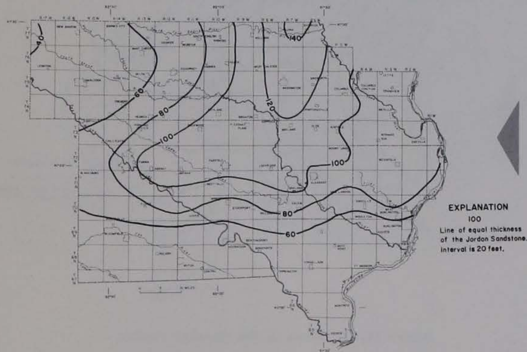
Figure 36.—Thickness of the Jordan Sandstone
