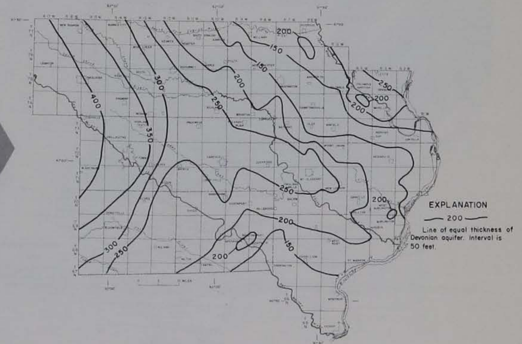
Figure 34.—Thickness of the Devonian aquifer
