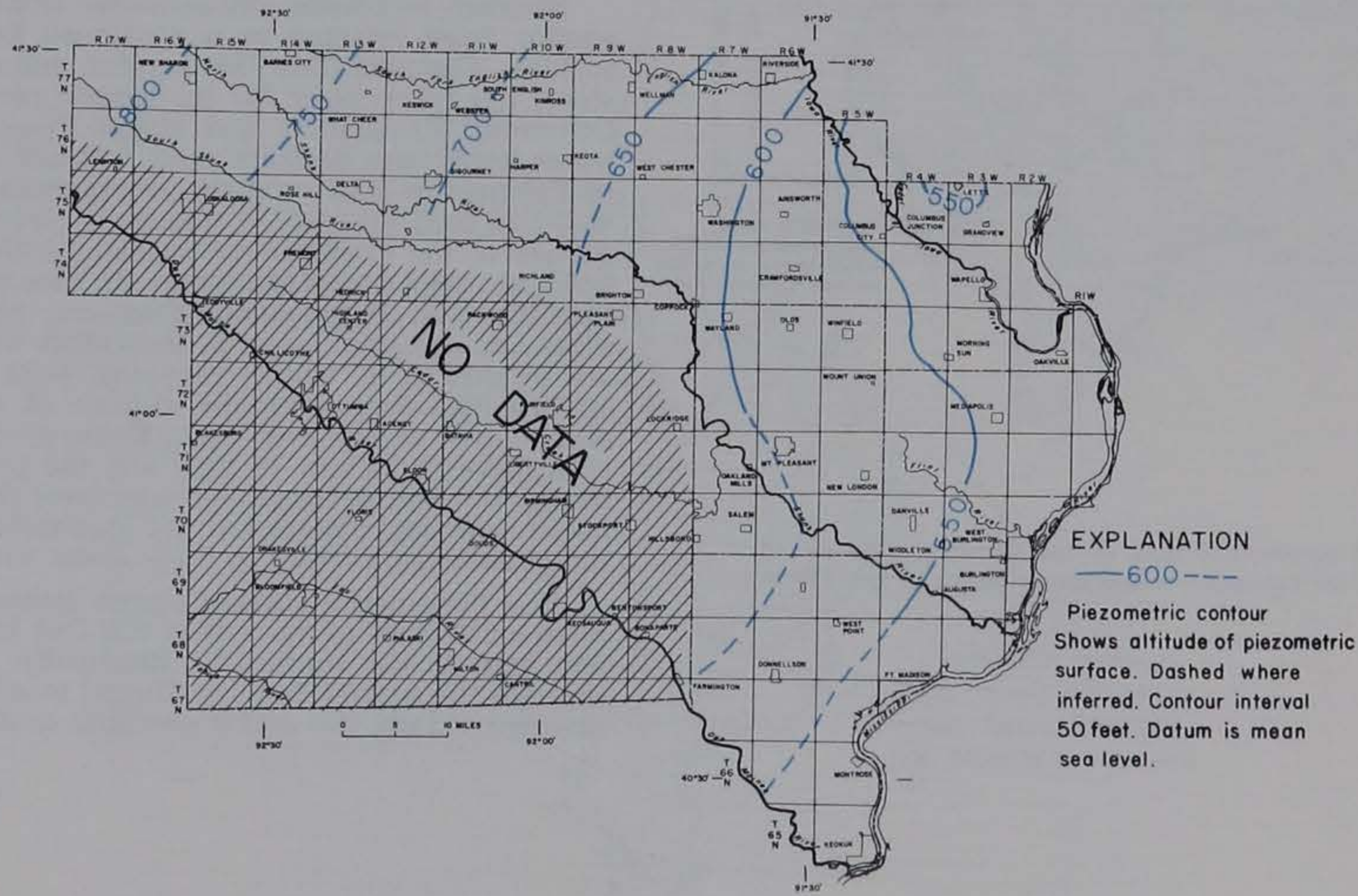
Figure 42.—Piezometric surface of the Devonian aquifer
