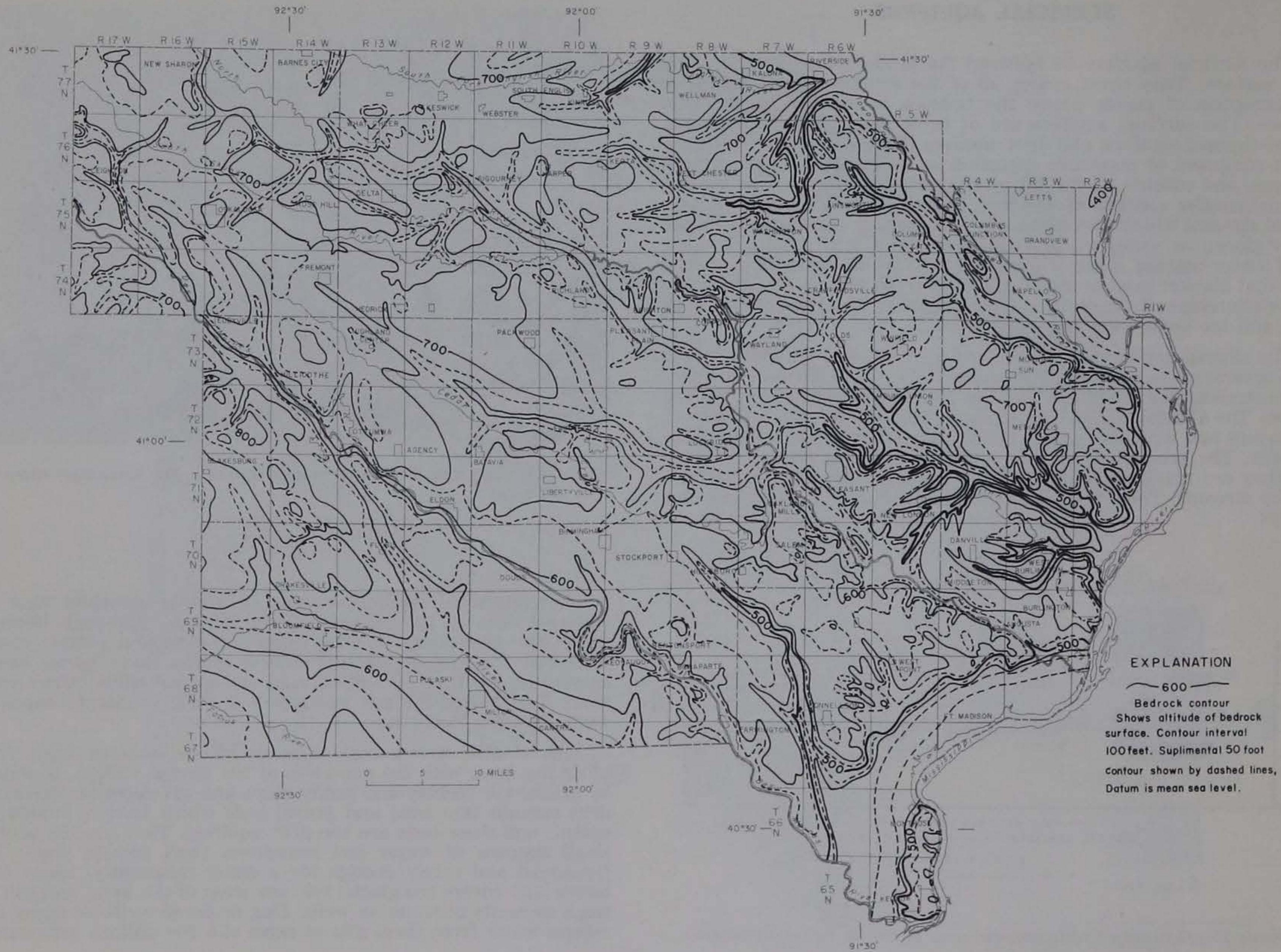
Figure 26.—Bedrock topographic map
