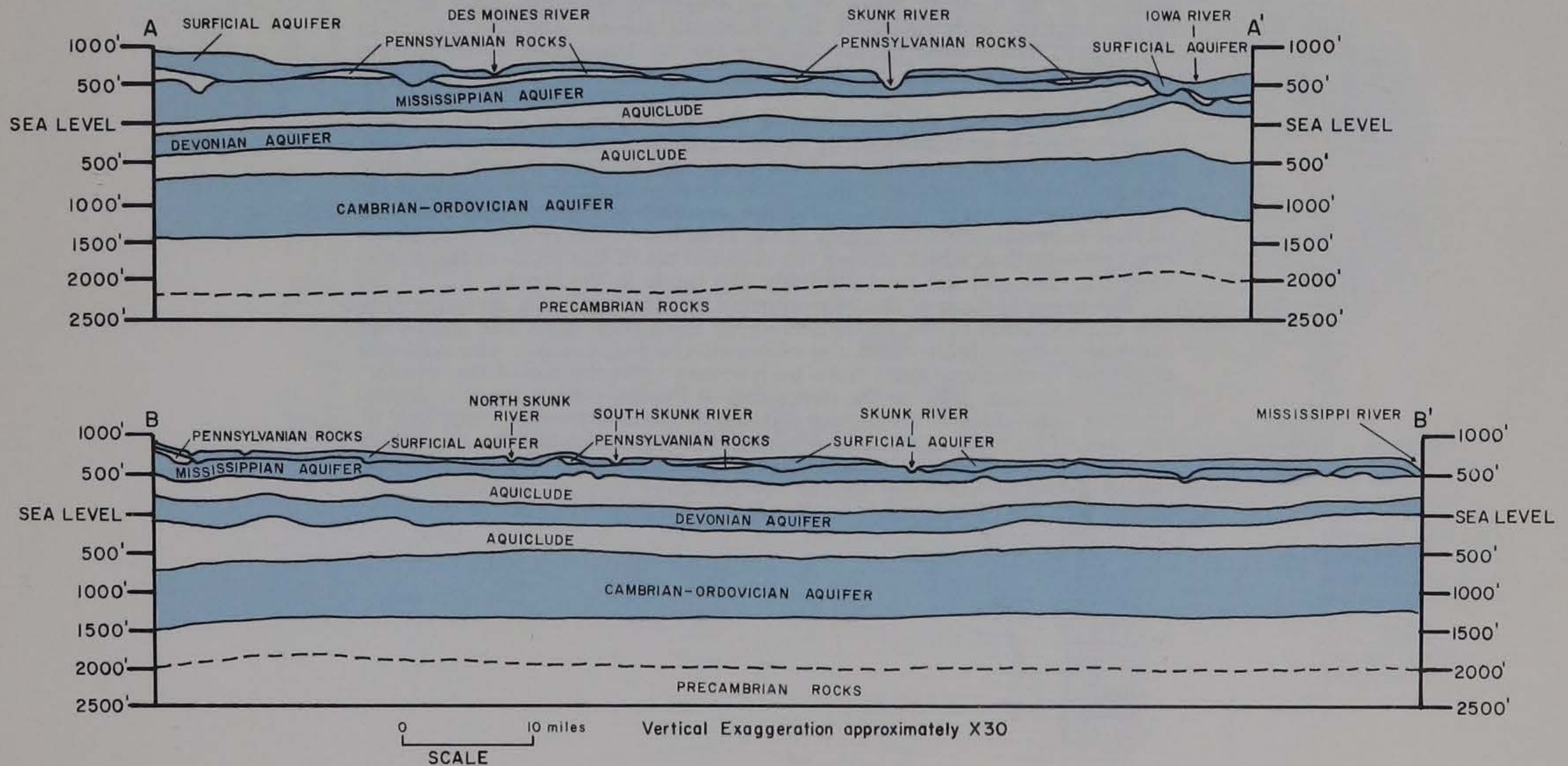
Figure 28.—Hydrogeologic cross sections
