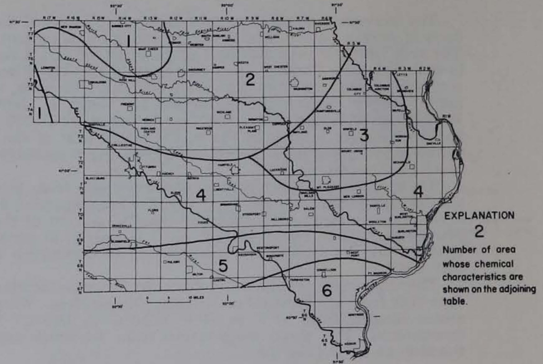
Figure 59.—Water-quality areas of the Cambrian-Ordovician aquifer
