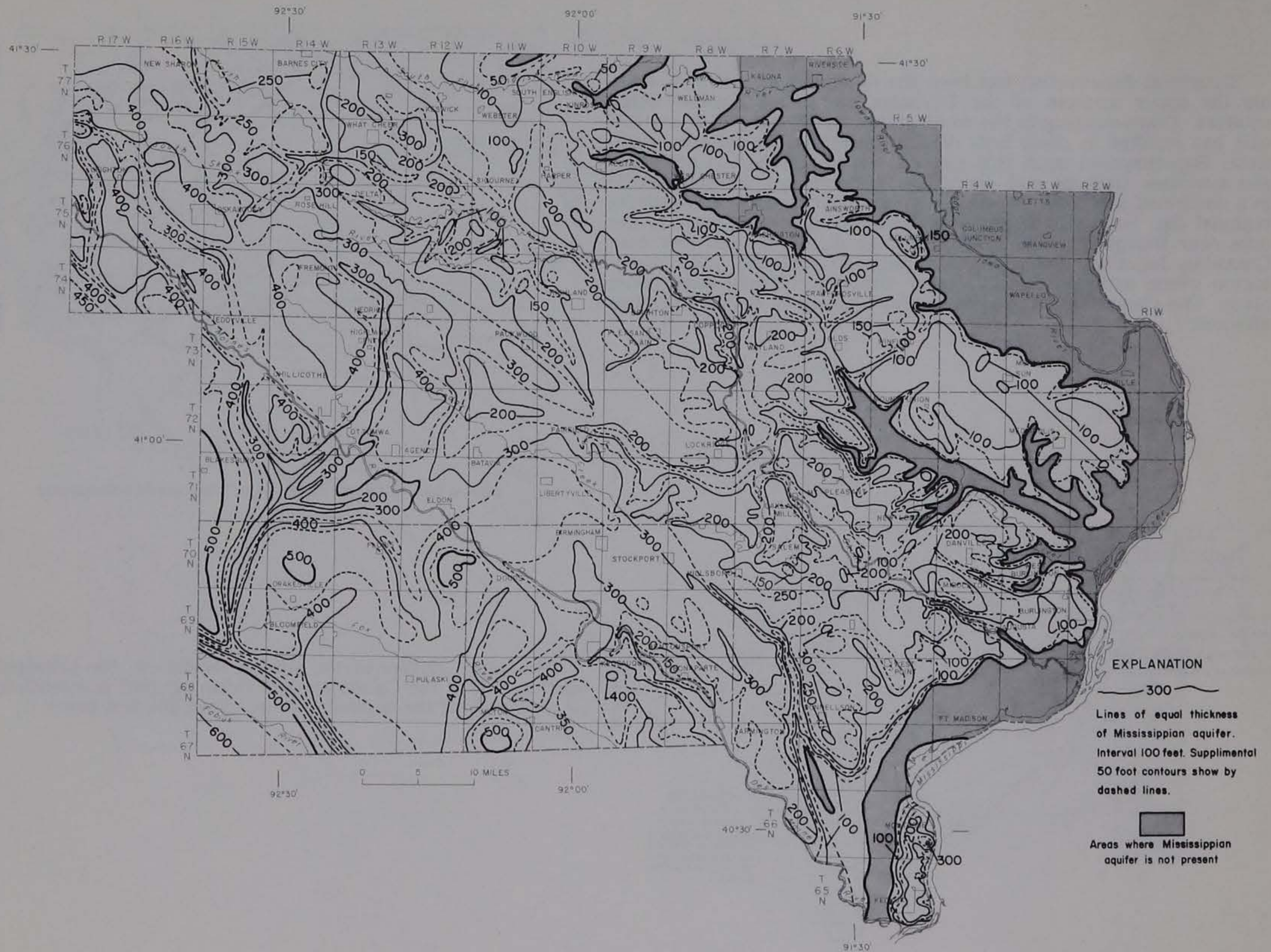
Fig. 33.—Thickness of the Mississippian aquifer
