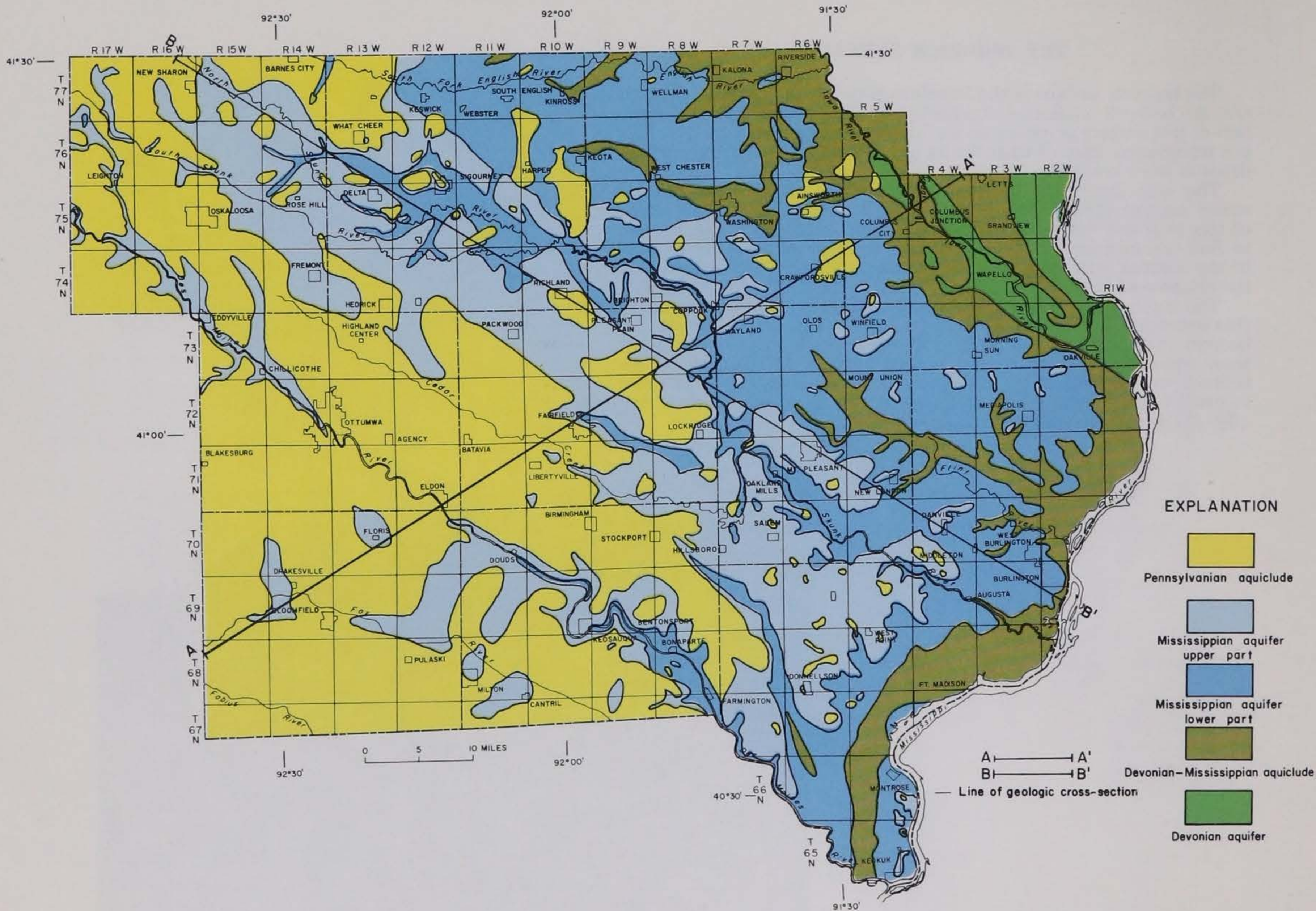
Figure 27.—Bedrock hydrogeologic map
