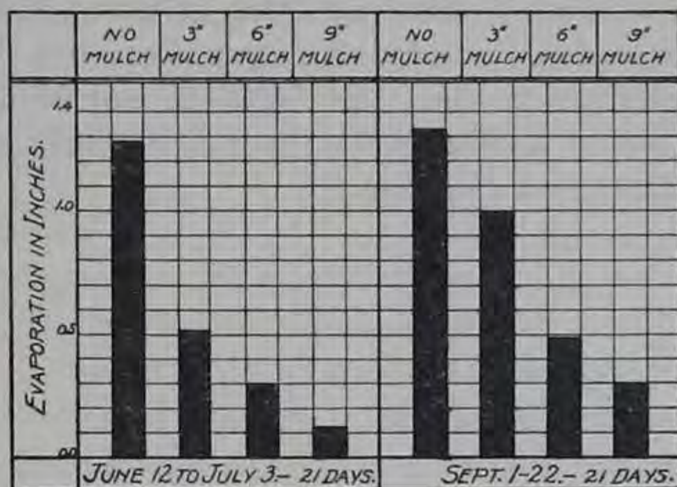
FIG. 27.—Evaporation at Reno, Nev., 1908.
