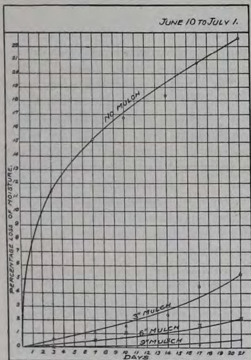
FIG. 24.—Curves showing daily rate of evaporation, Davis, Cal.
