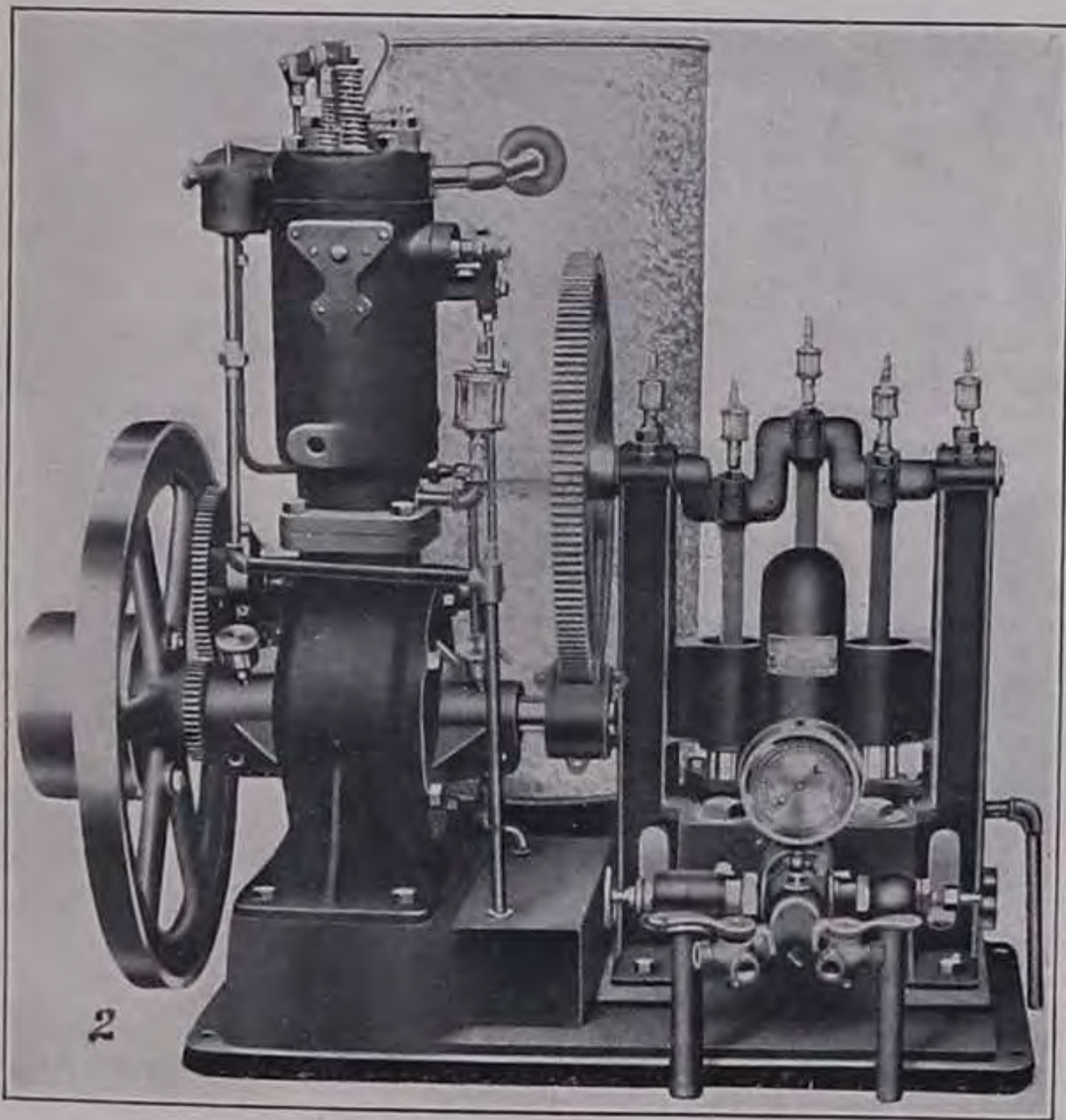
TYPES OF SPRAYING APPARATUS: GASOLINE-POWER OUTFITS.
