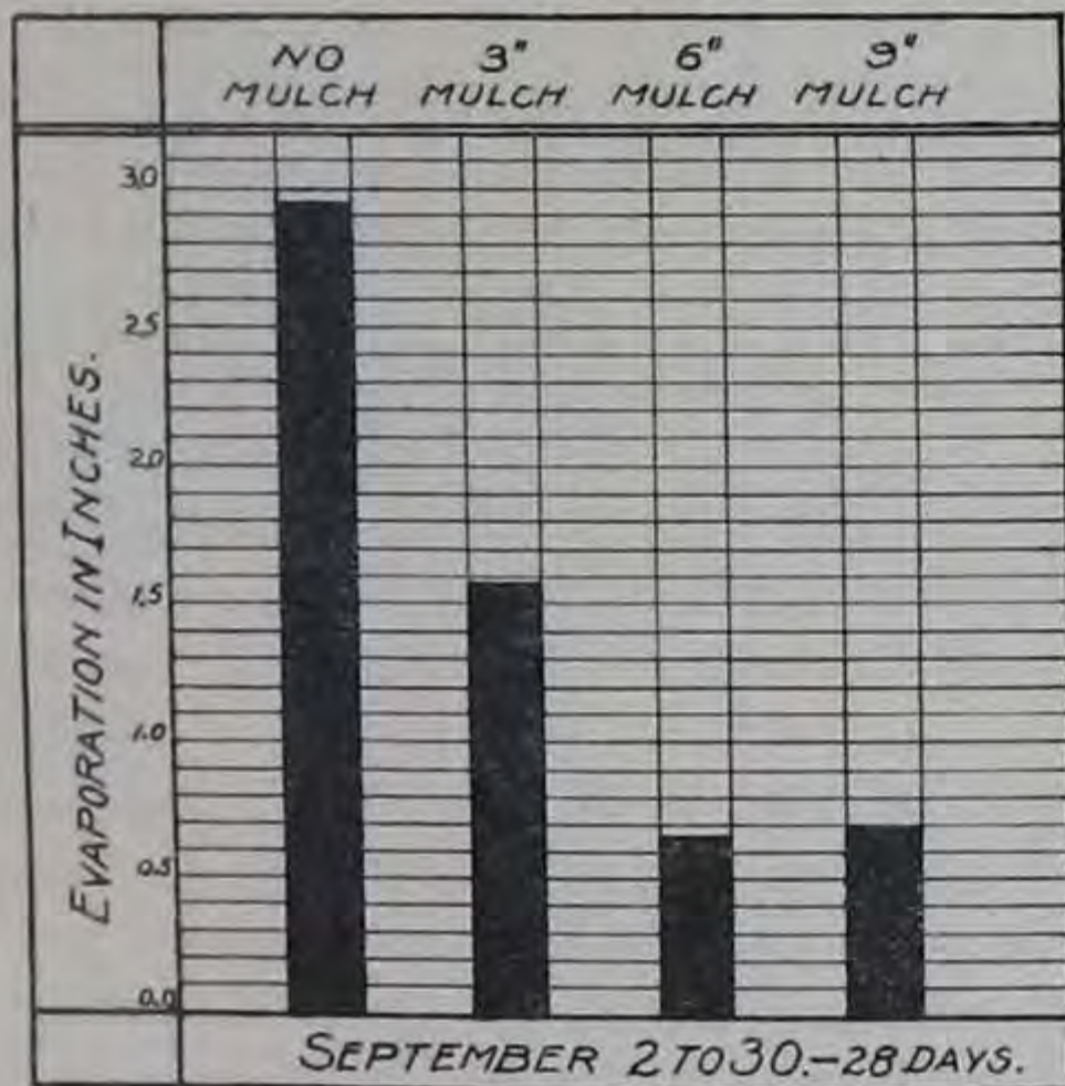
FIG. 28.—Evaporation at Bozeman, Mont., 1908.
