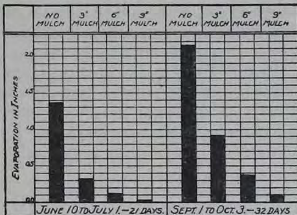
FIG. 23.—Evaporation at Davis, Cal., 1908.
