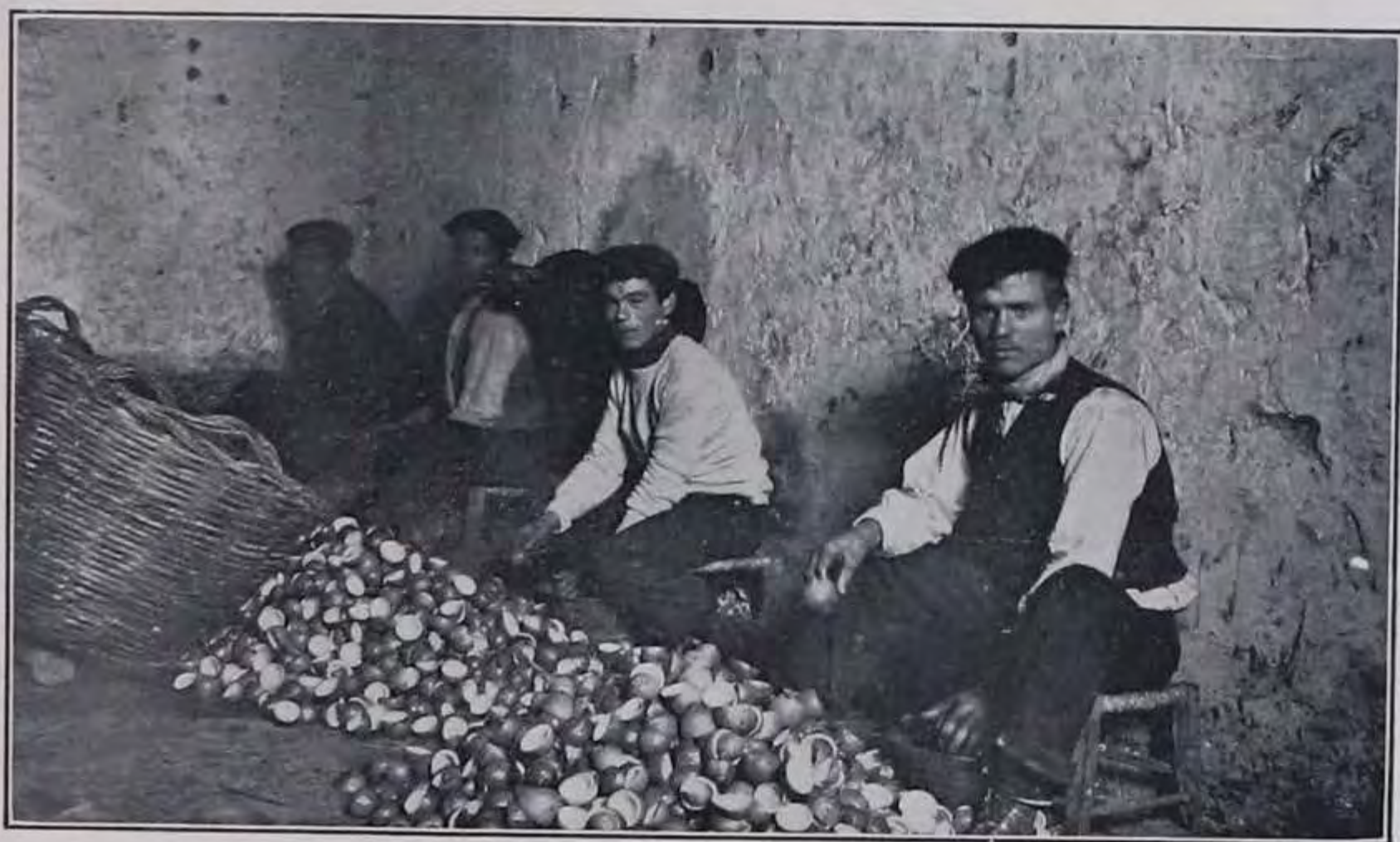
FIG. 2.—EXPRESSING LEMON OIL, TWO-PIECE METHOD, MESSINA SICILY.
