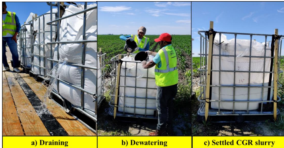
Figure 51. Dewatering process for CGR slurry at the demonstration site in Washington County: (a) draining water from bags, (b) manual dewatering, and (c) settled CGR slurry
