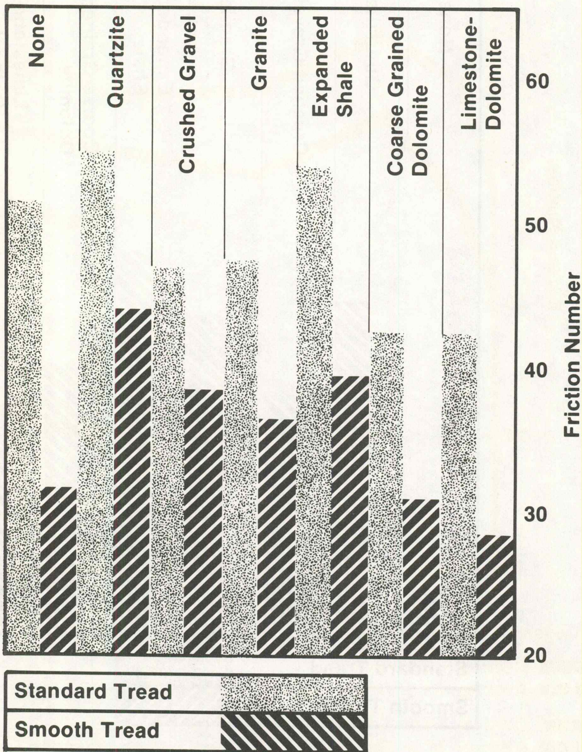
Figure 3: Friction Number of Sprinkle Treatments on the Asphalt Sand Surface Course Four Years After Construction
