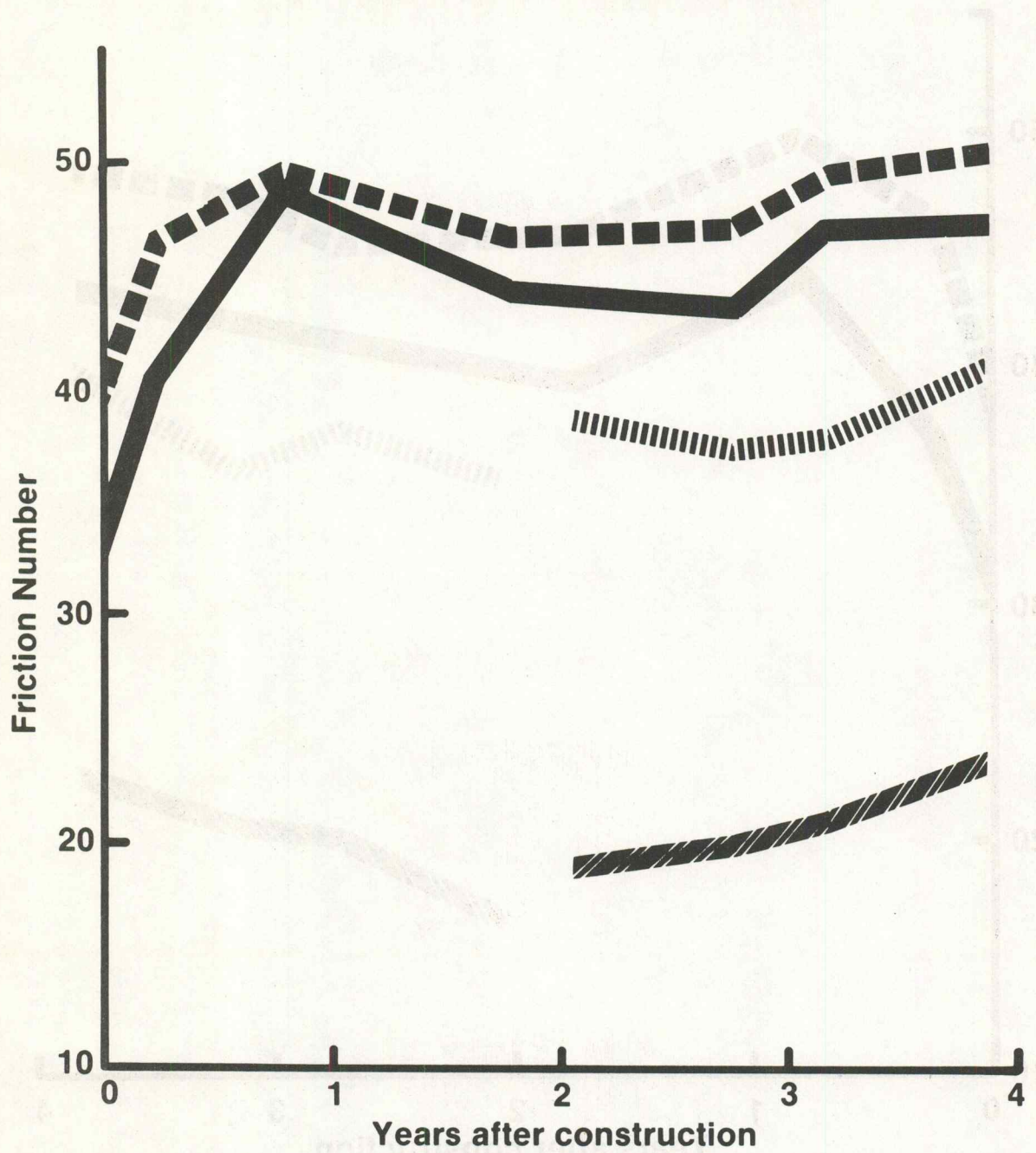
Figure 5: Comparison of Friction Numbers for Sprinkle Treated Sections and Control Sections on Type B \frac{3}{8} " (10 MM) Mix
