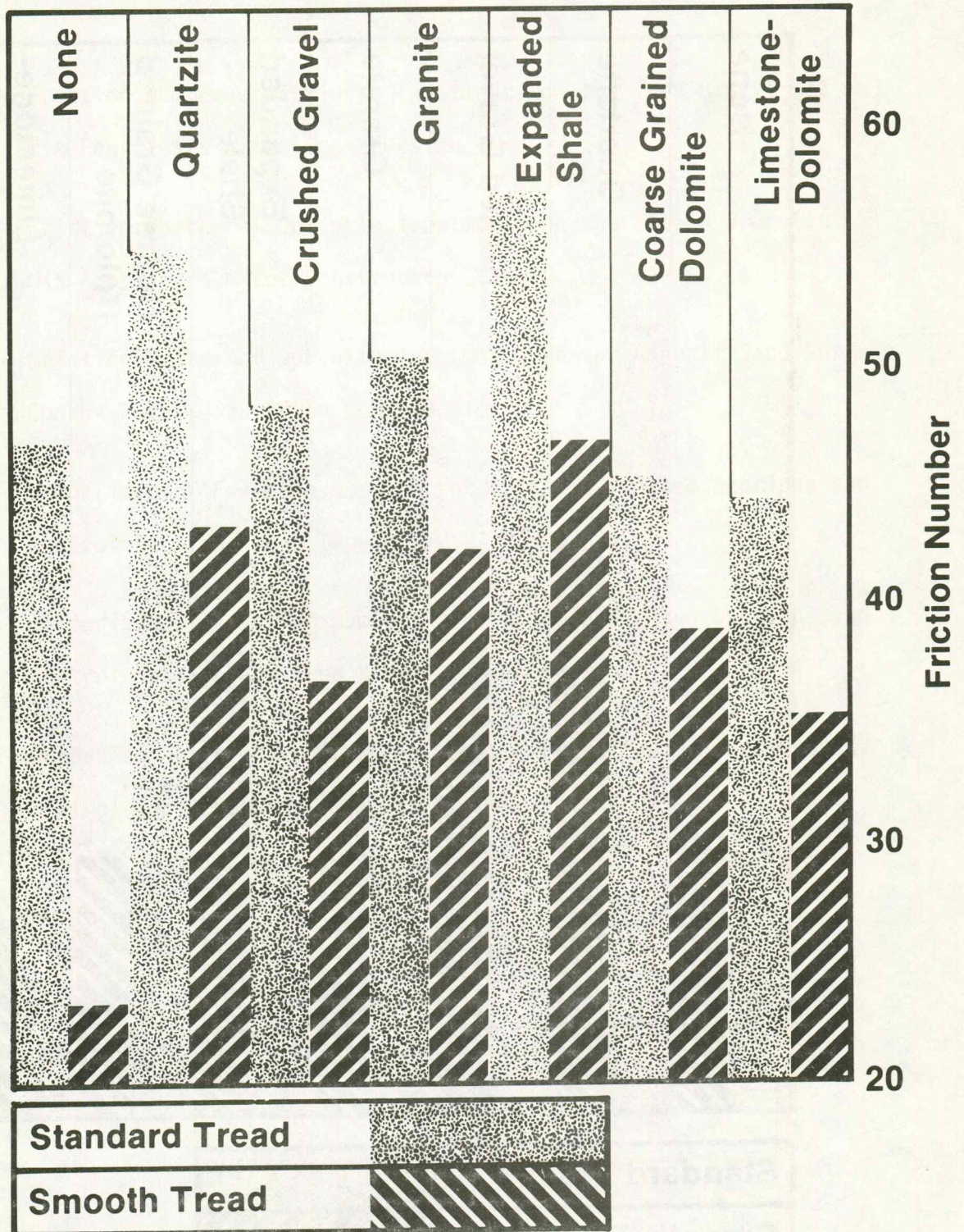
Figure 2: Friction Number of Sprinkle Treatments on the Type B \frac{3}{8} " (10 MM) Mix Four Years After Construction
