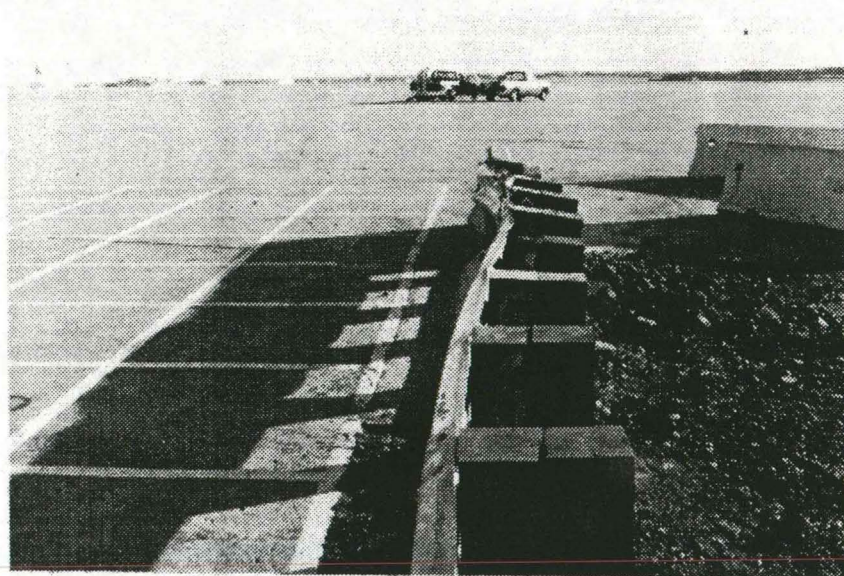
FIGURE 26. PHOTOGRAPHS OF DAMAGE TO APPROACH GUARDRAIL TRANSITION SECTION.
