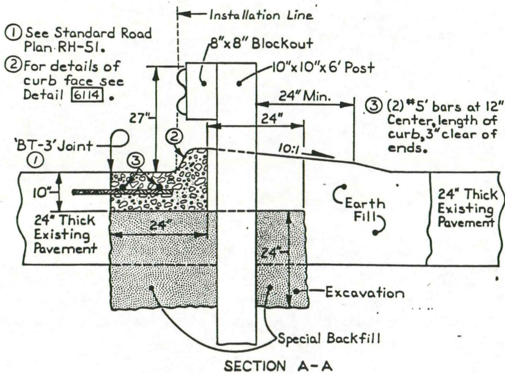
FIGURE 12. DETAIL OF POST EMBEDMENT AND W-BEAM ATTACHMENT.
