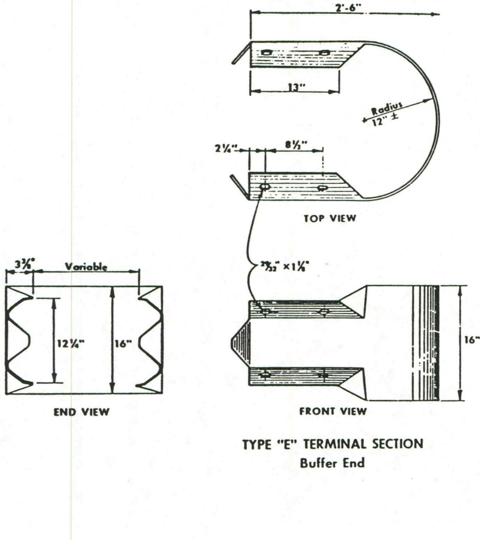
FIGURE 9. SKETCH OF FORMED STEEL TERMINAL SECTIONS.
