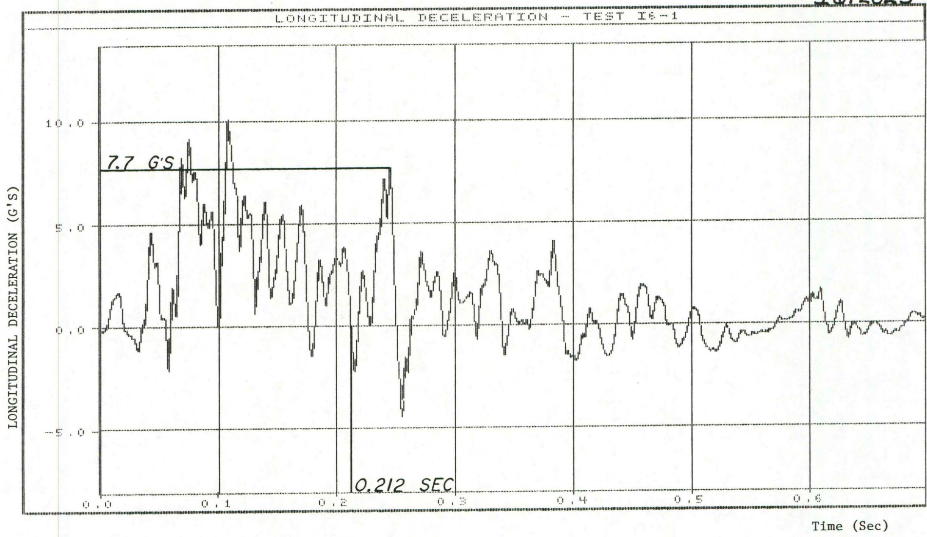
FIGURE C-1. GRAPH OF LONGITUDINAL DECELERATION, TEST I6-1.
