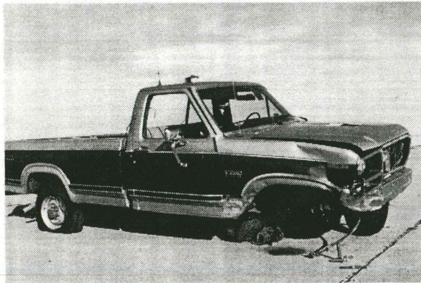
FIGURE 22. PHOTOGRAPHS OF VEHICLE DAMAGE.
