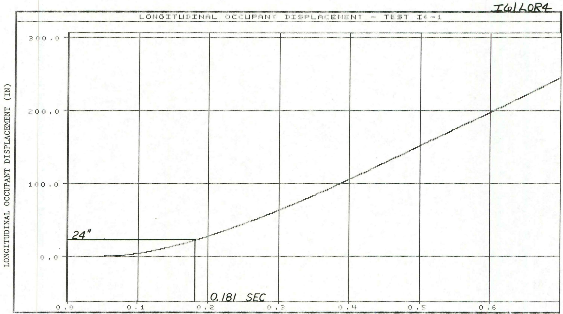
FIGURE C-6. GRAPH OF LONGITUDINAL OCCUPANT DISPLACEMENT, TEST I6-1.
