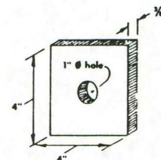
DETAIL OF GALVANIZED STEEL WASHER
