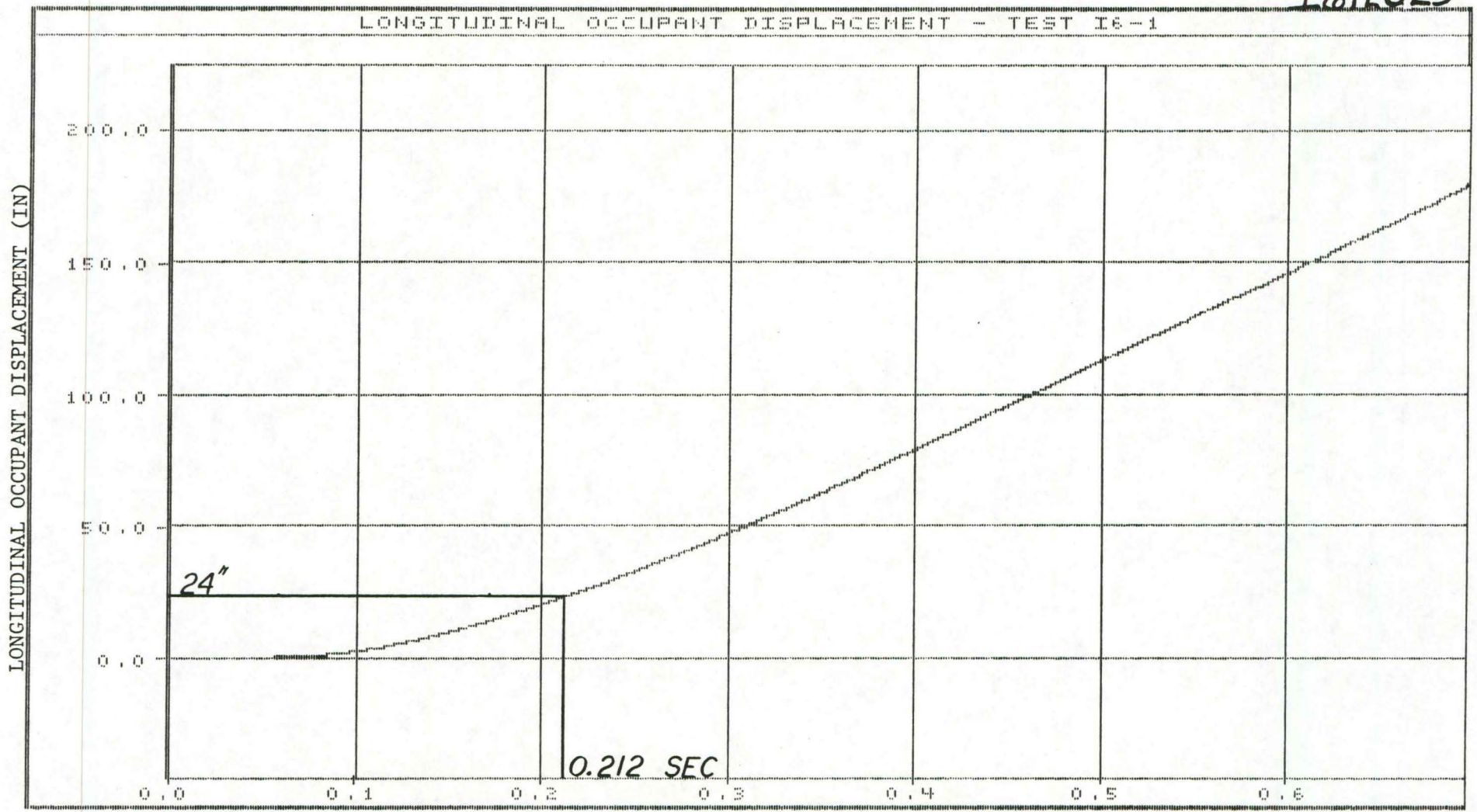
FIGURE C-5. GRAPH OF LONGITUDINAL OCCUPANT DISPLACEMENT, TEST I6-1.
