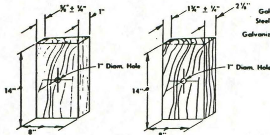
SPACER BLOCK DETAILS
