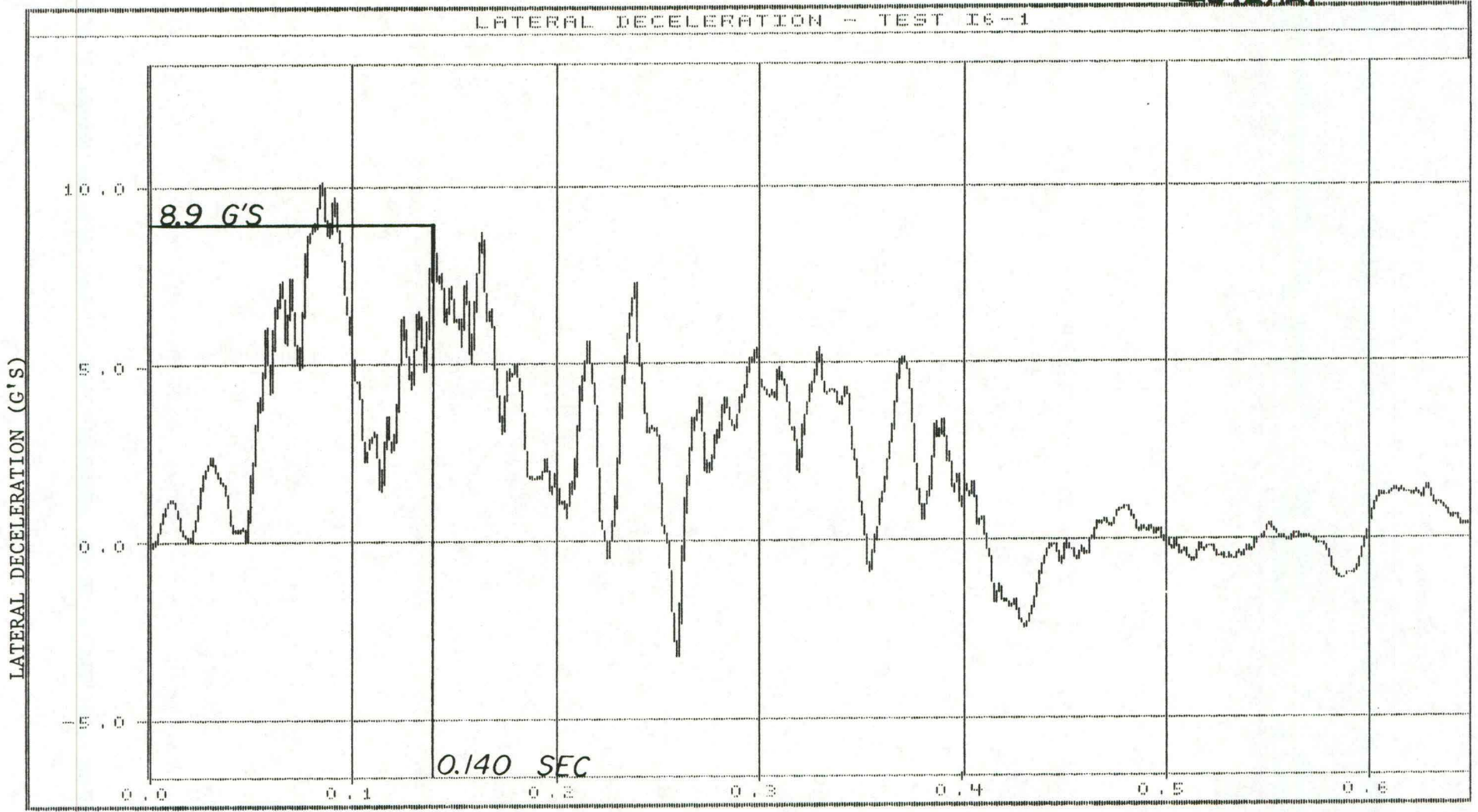
FIGURE C-7. GRAPH OF LATERAL DECELERATION, TEST I6-1.
