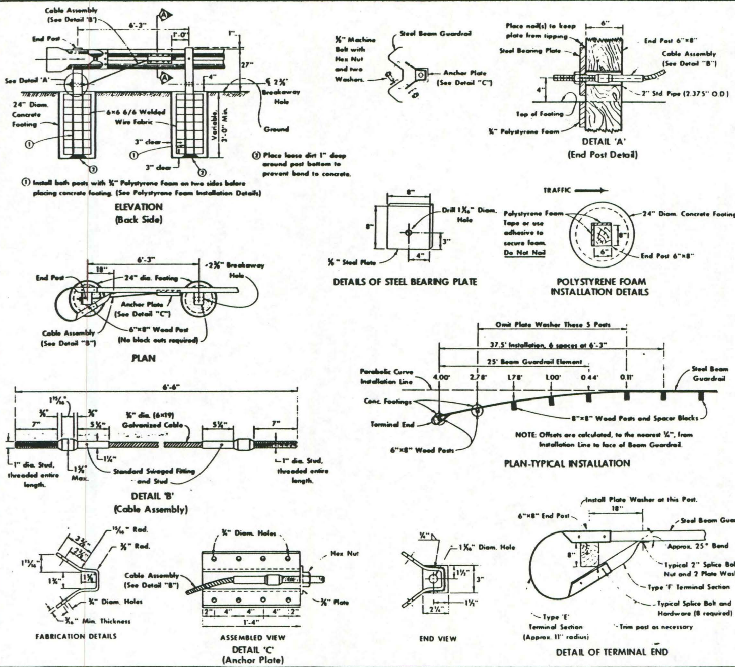
FIGURE 8. SKETCH OF BREAKAWAY END ANCHORAGE.
