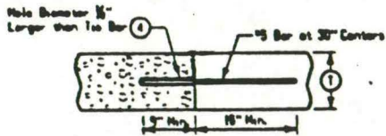
'BT-3' ABUTTING PAVEMENT JOINT, RIGID TIE (FORMERLY 'BD' JOINT)
