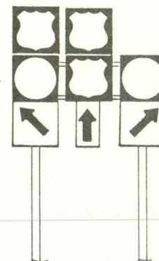
4" X 6" Posts 72" Auxiliary Bar 1 Two Post Bracket
