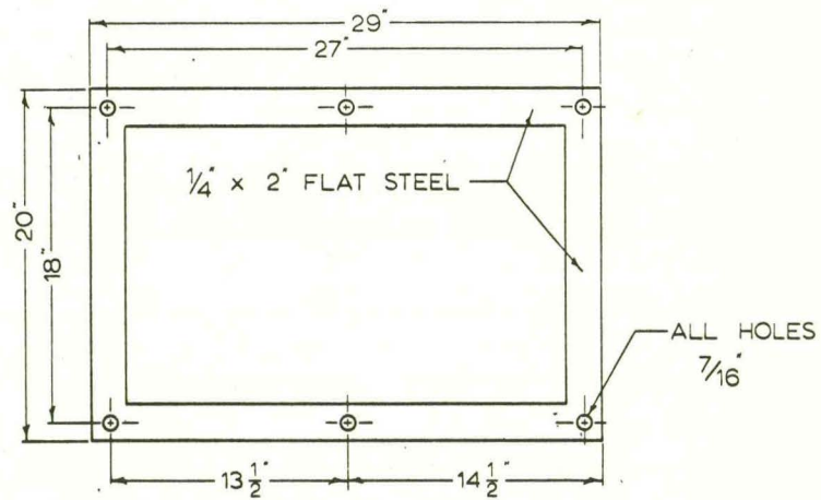
ONE POST SIGN MOUNTING BRACKET
