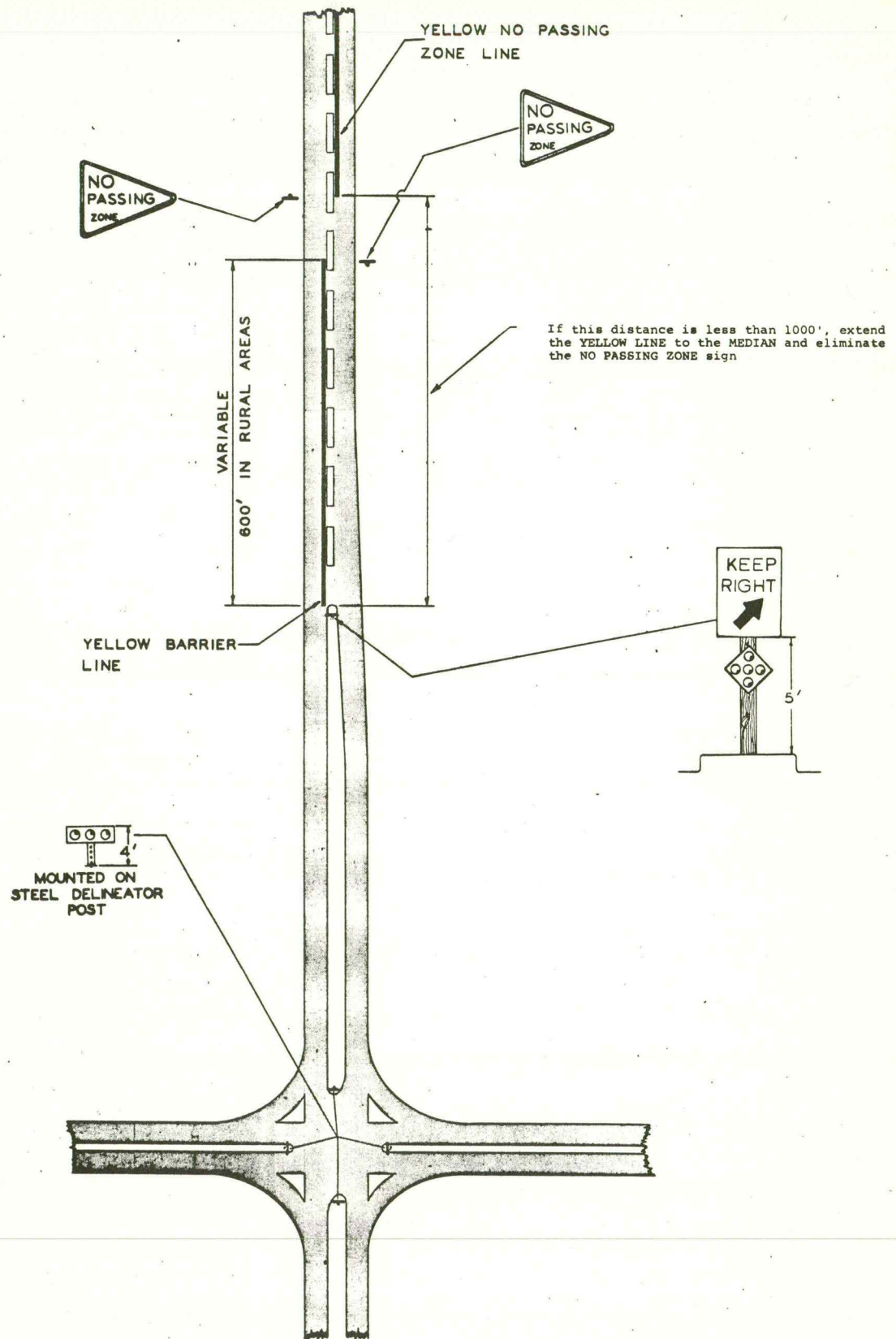
Figure xiv TYPICAL APPLICATION OF BARRIER LINE AT CHANNELIZED INTERSECTION
