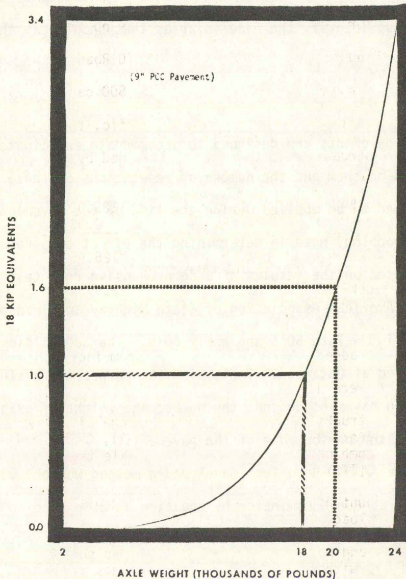
RELATIONSHIP BETWEEN AXLE WEIGHT AND 18 KIP EQUIVALENTS
