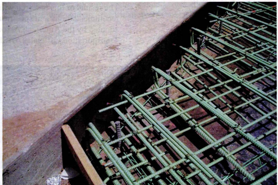
Installation of an improved bridge-to-pavement connection detail
