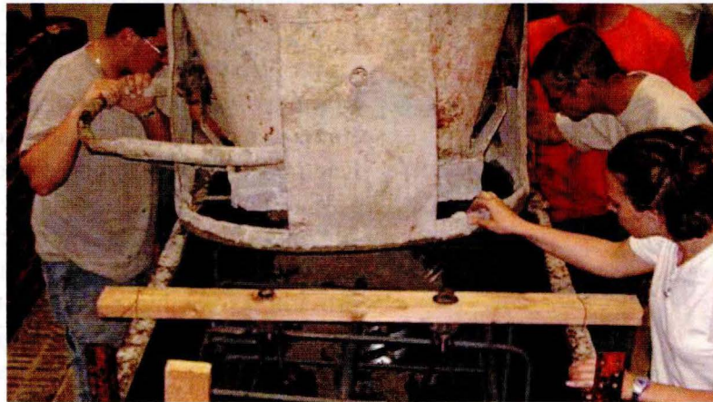
Concrete being placed in the first series of abutment specimen
