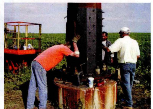
A bolted reinforcing jacket was placed on a tower in the I-35 & US 18 Interchange near Clear Lake
