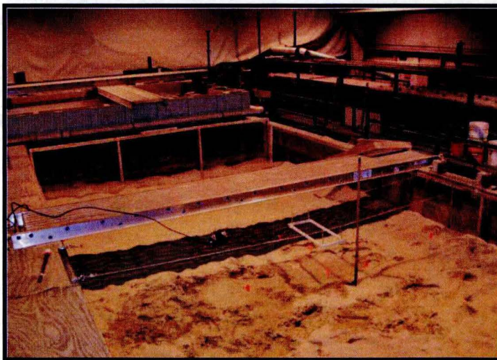
The water/sediment re-circulating flume for the RFID tests (antenna is at the center of the flume)
