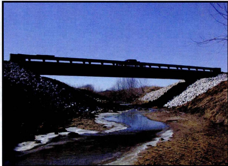
A UHPC prestressed bridge constructed on Little Soap Road in Wapello County, Iowa
