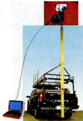
MLSPIV unit with mast deployed and ancillary equipment
