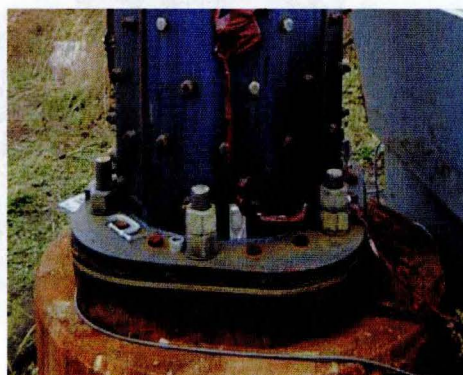
Bolted Reinforcing Jacket
