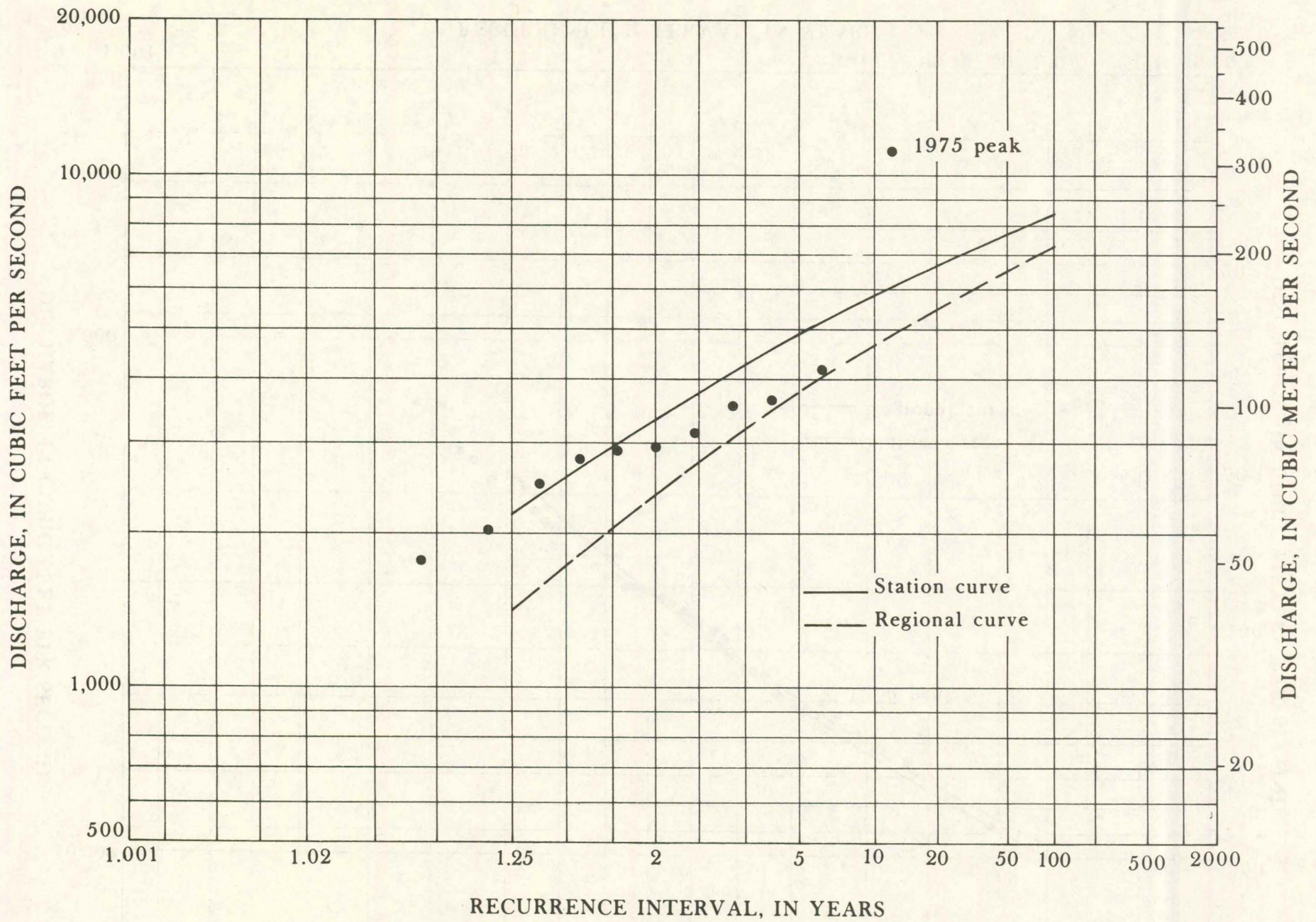
Figure 17. Flood frequency curves for gaging station 05470500 Squaw Creek at Ames, Iowa.
