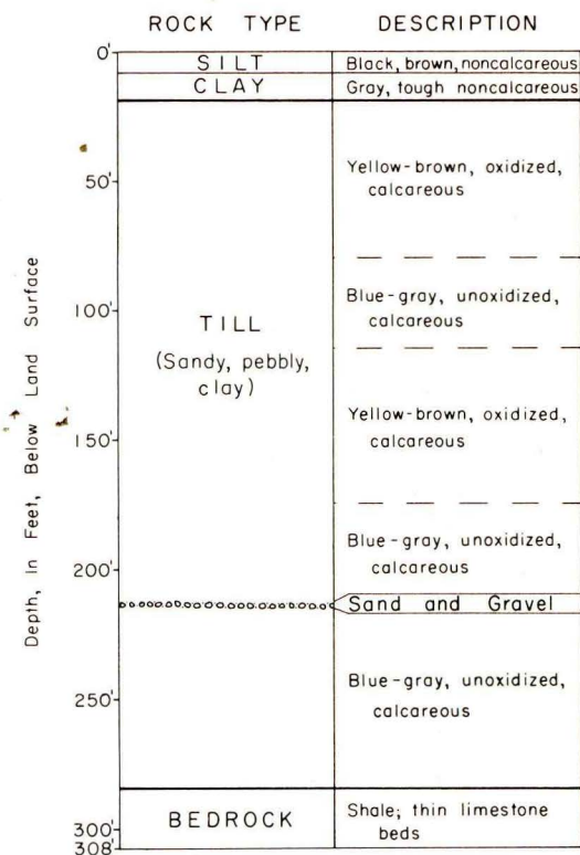
Log of test hole D-51, which is generally representative of the composition of the glacial drift in the county.
