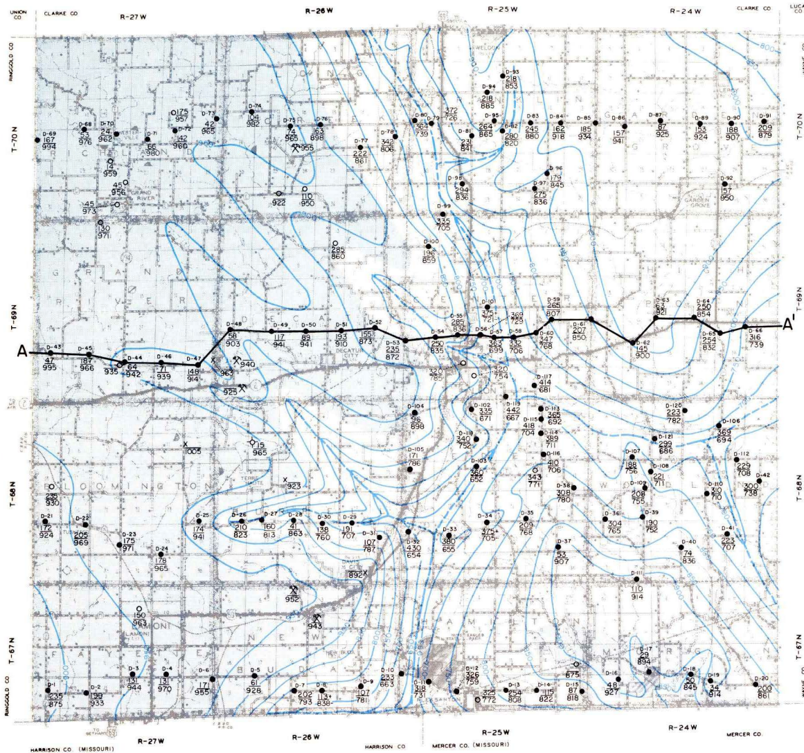
Bedrock topography and geology.
