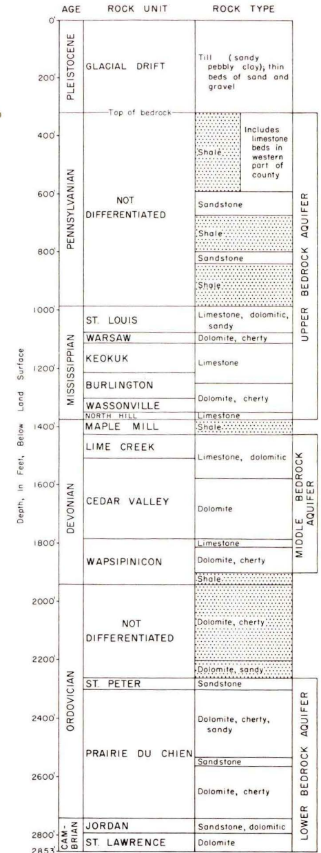
Rock units that underlie the county. Data is based on log of Leon well No. 4
