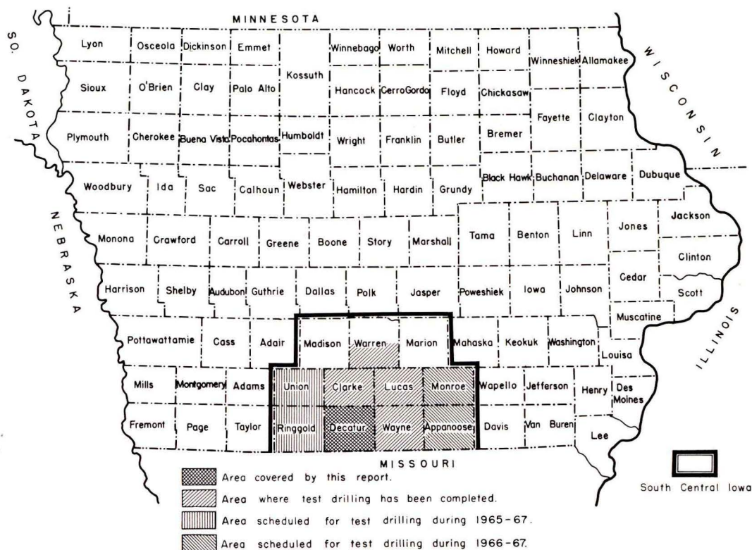
Progress of ground-water investigation in south-central Iowa.
