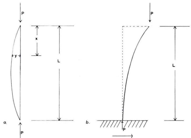
Fig. A-5. Diagram of a slender column under axial loading.
