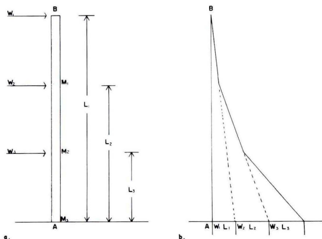
Fig. A-3. Diagram of cantilever beam with several concentrated loads.
