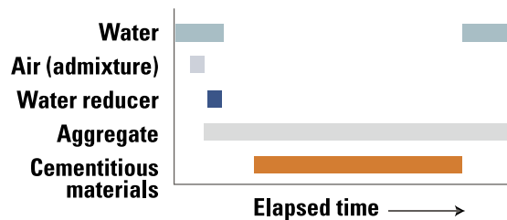
Figure 8-9. Typical sequence of adding material in a truck mixer
