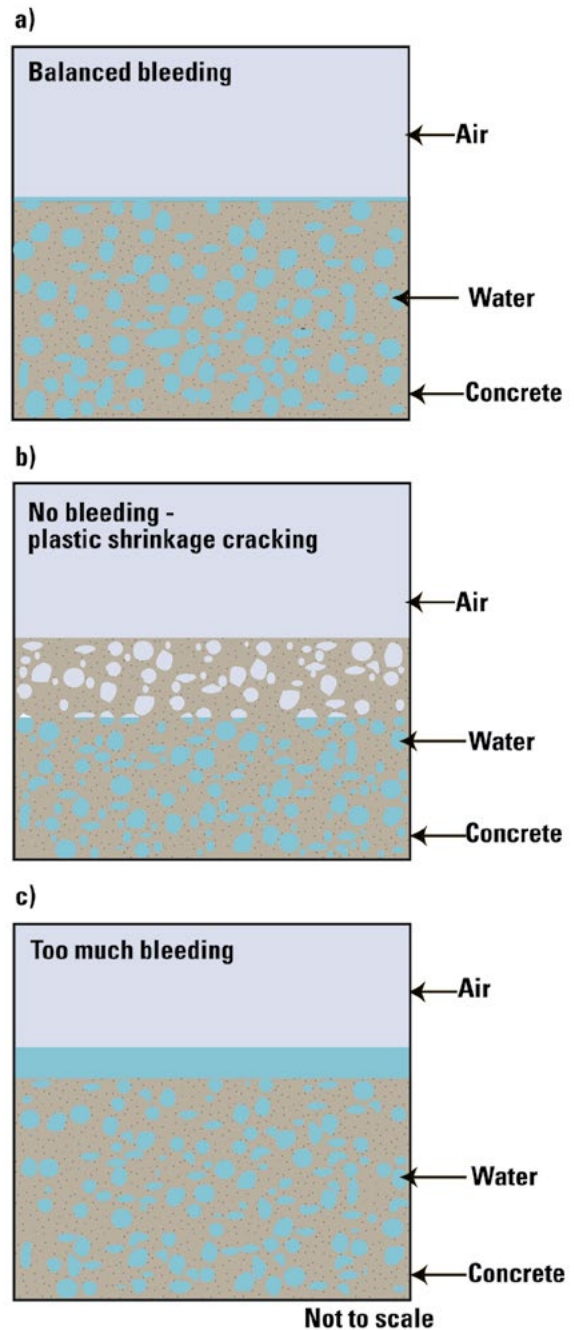
Figure 6-5. Bleeding
