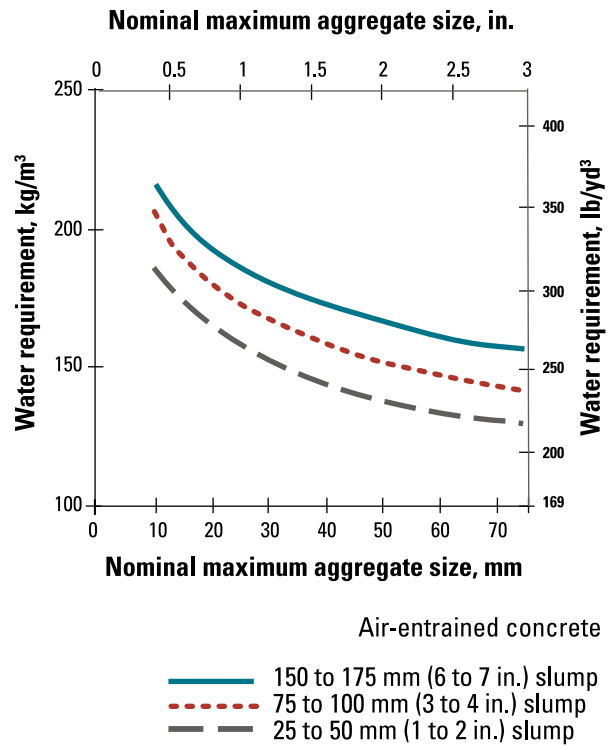
Figure 7-8. Approximate water requirement for various slumps and crushed aggregate sizes for air-entrained concrete
