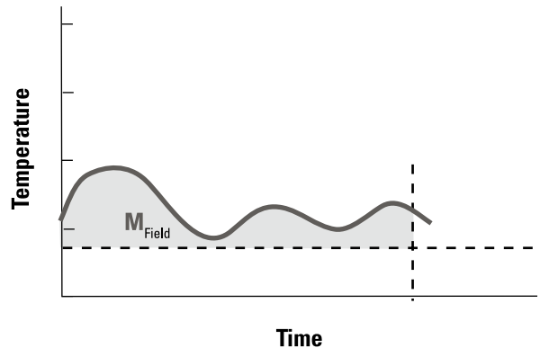
Figure 6-14. Maturity of the field concrete is equivalent to maturity of the laboratory concrete when the area under the curves is the same
