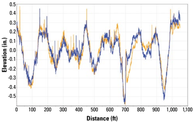
Figure 9-12. Raw profile data
