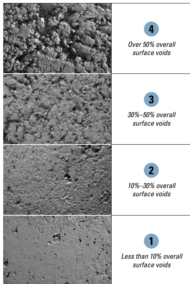
Figure 9-5. Rating standards for Box test
