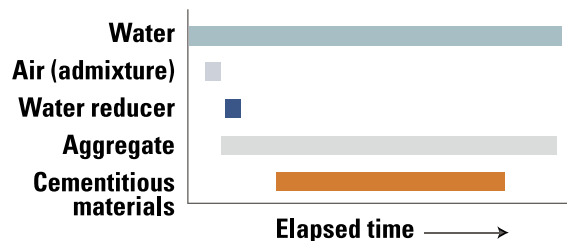
Figure 8-8. Typical sequence of adding material in a stationary mix plant
