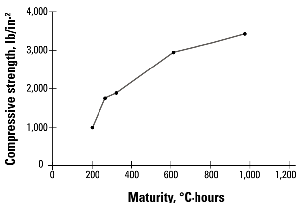
Figure 9-8. Sample maturity curve
