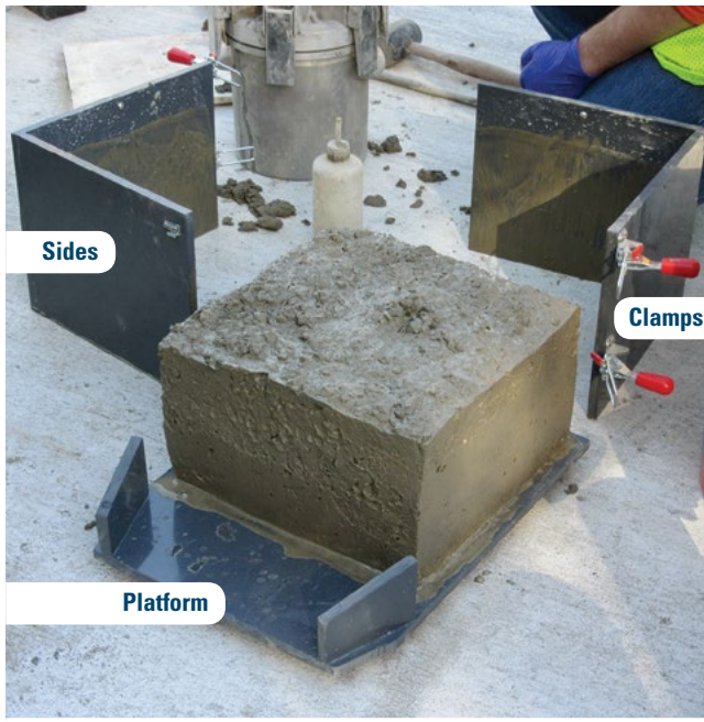
Step 1 Gather the different components of the Box test.
