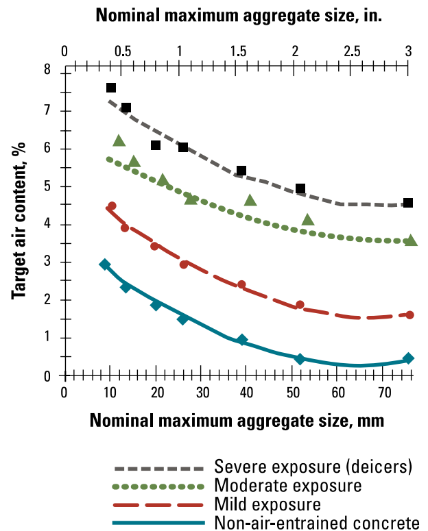
Figure 7-7. Target total air content requirements for concretes using different sizes of aggregate
