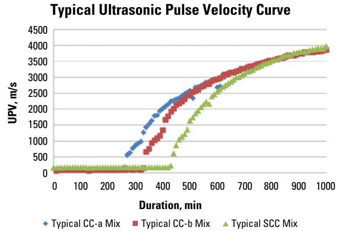
Figure 6-7. Ultrasonic velocity accelerates when mixture begins to set
