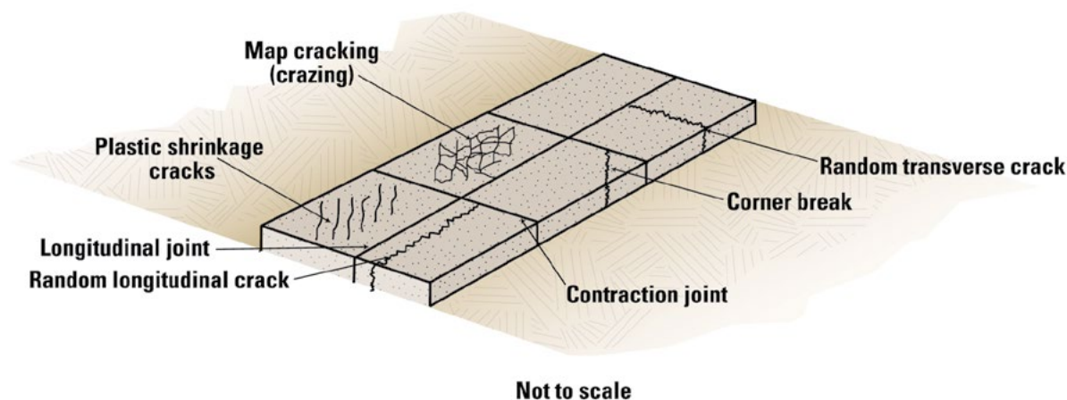
Figure 10-1. Early-age cracking
