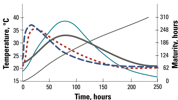
Figure 9-10. Heat signature sample plots
