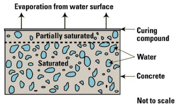
Figure 4-23. Curing compounds keep concrete partially saturated near the surface during the curing period
