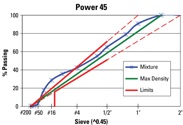
Figure 7-4. Sample Power 45 plot
