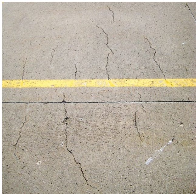
Figure 6-26. Plastic shrinkage cracks
