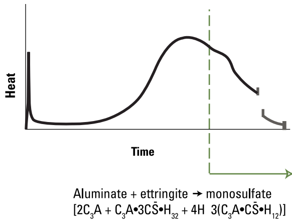
Figure 5-24. After C\bar{S} is consumed, remaining C_3A reacts with ettringite
