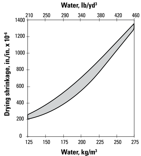
Figure 6-17. Relationship between total water content and drying shrinkage
