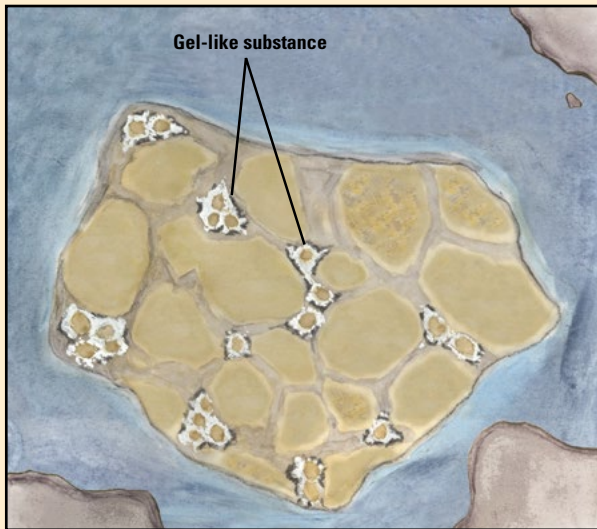
Figure 5-3. A gel-like substance coats cement compounds, controlling the reactions and heat
