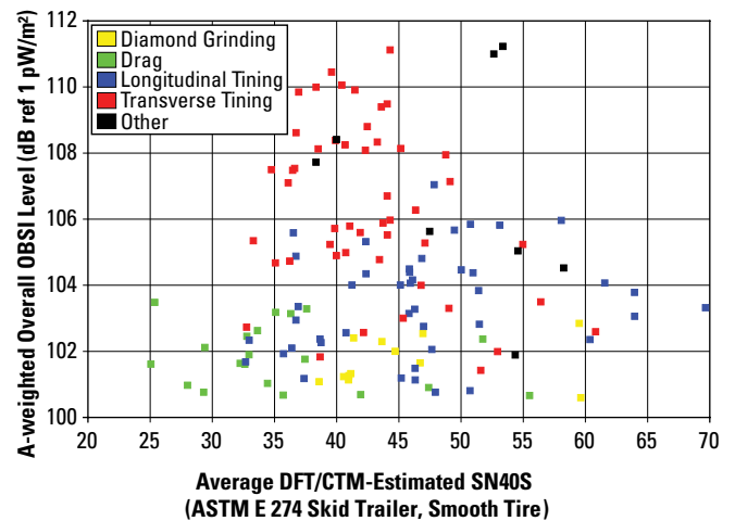
Figure 8-23. Noise and skid resistance are independent
