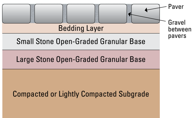
Figure 2-2. Examples of fully permeable concrete pavement systems
