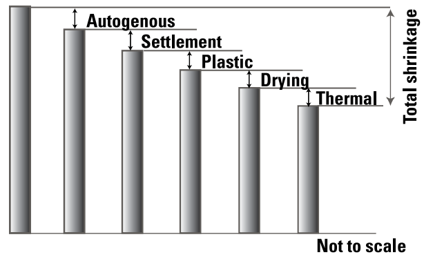
Figure 6-16. Total shrinkage is a sum of all individual shrinkage mechanisms. Minimizing any or all of the mechanisms will reduce the risk of cracking
