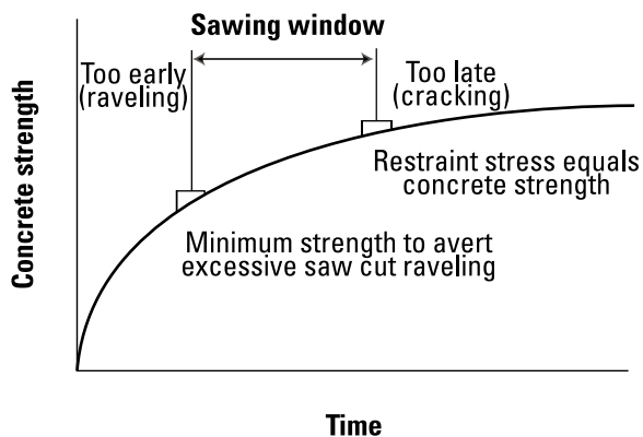
Figure 8-34. Sawing window
