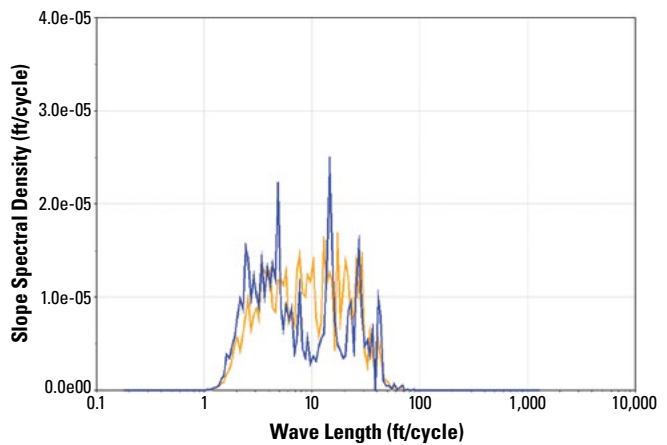
Figure 9-14. ProVAL power spectral density plot showing a repeating wavelength at 15 ft that corresponds to joint spacing
