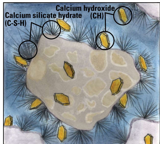
Figure 5-17. C-S-H and CH begin to form
