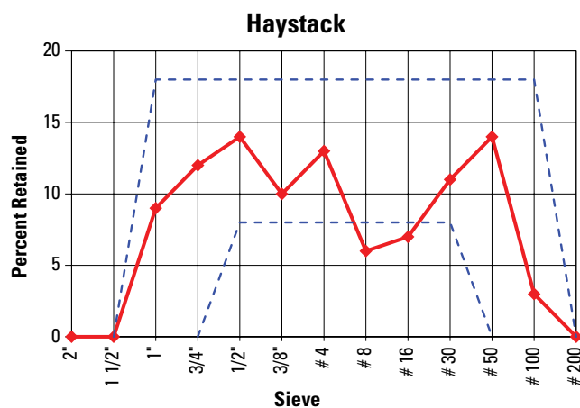
Figure 7-5. Sample Haystack plot
