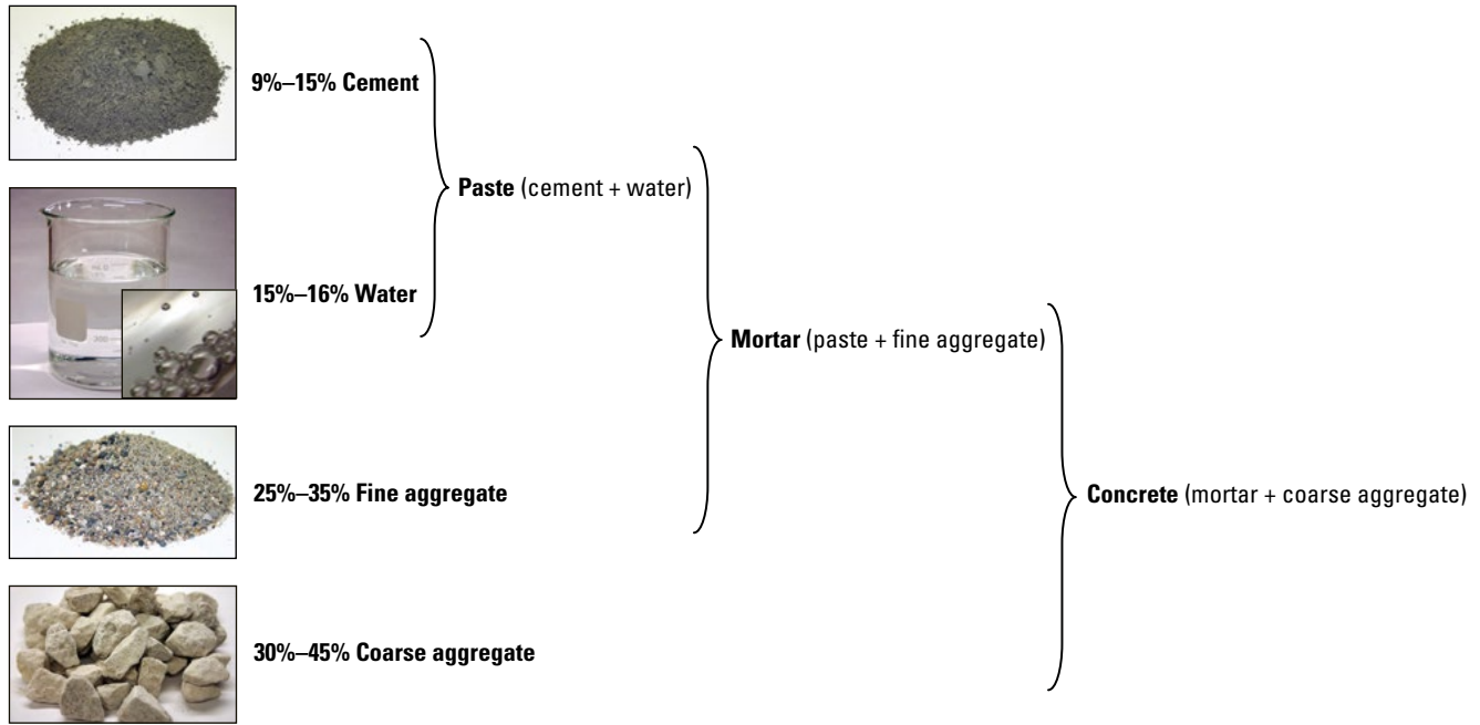
Figure 4-1. Concrete is basically a mixture of cement, water/air, and aggregates (percentages are by volume for pavements)
