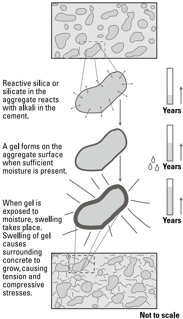
Figure 6-39. Alkali-silica reaction is an expansive reaction of reactive aggregates, alkali hydroxides, and water that may cause cracking in concrete
