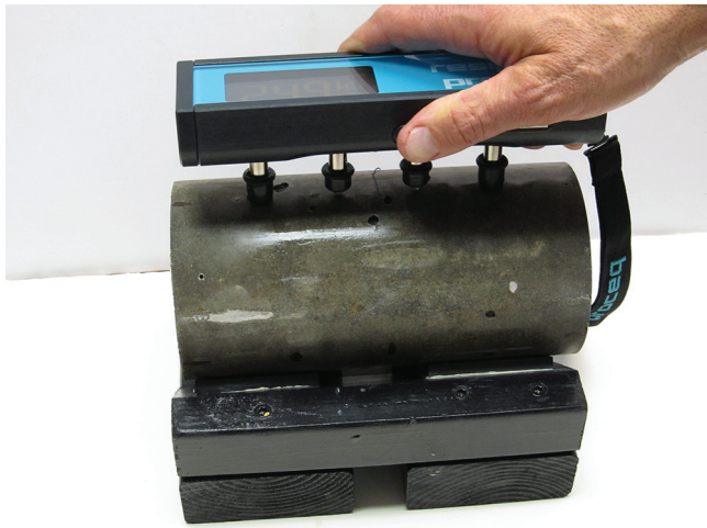
Figure 6-31. Wenner resistivity test
