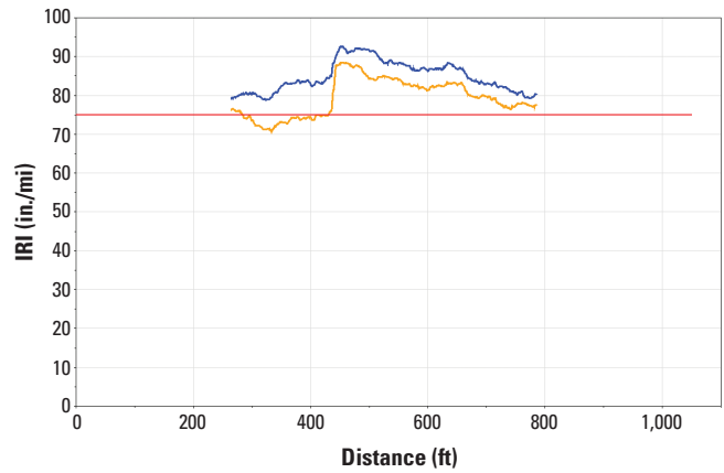
Figure 9-13. ProVAL roughness report
