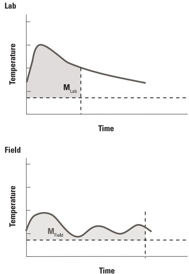
Figure 6-14. Maturity of the field concrete is equivalent to maturity of the laboratory concrete when the area under the curves is the same
