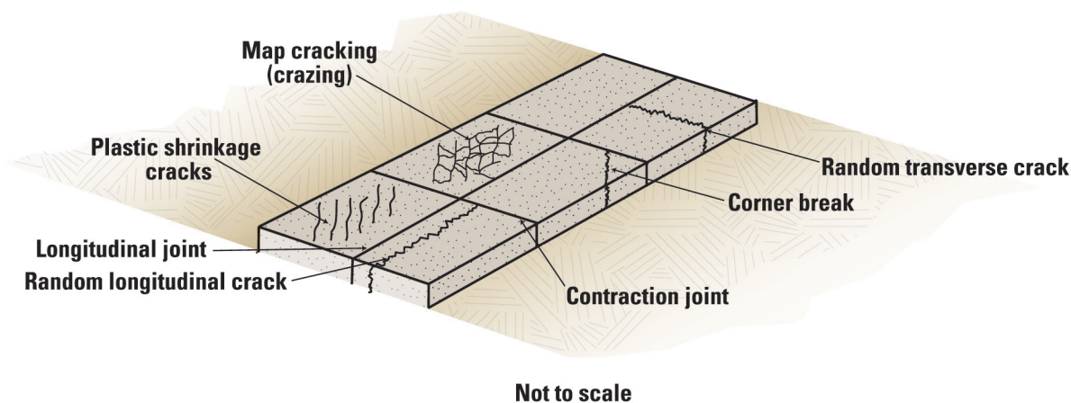
Figure 10-1. Early-age cracking
