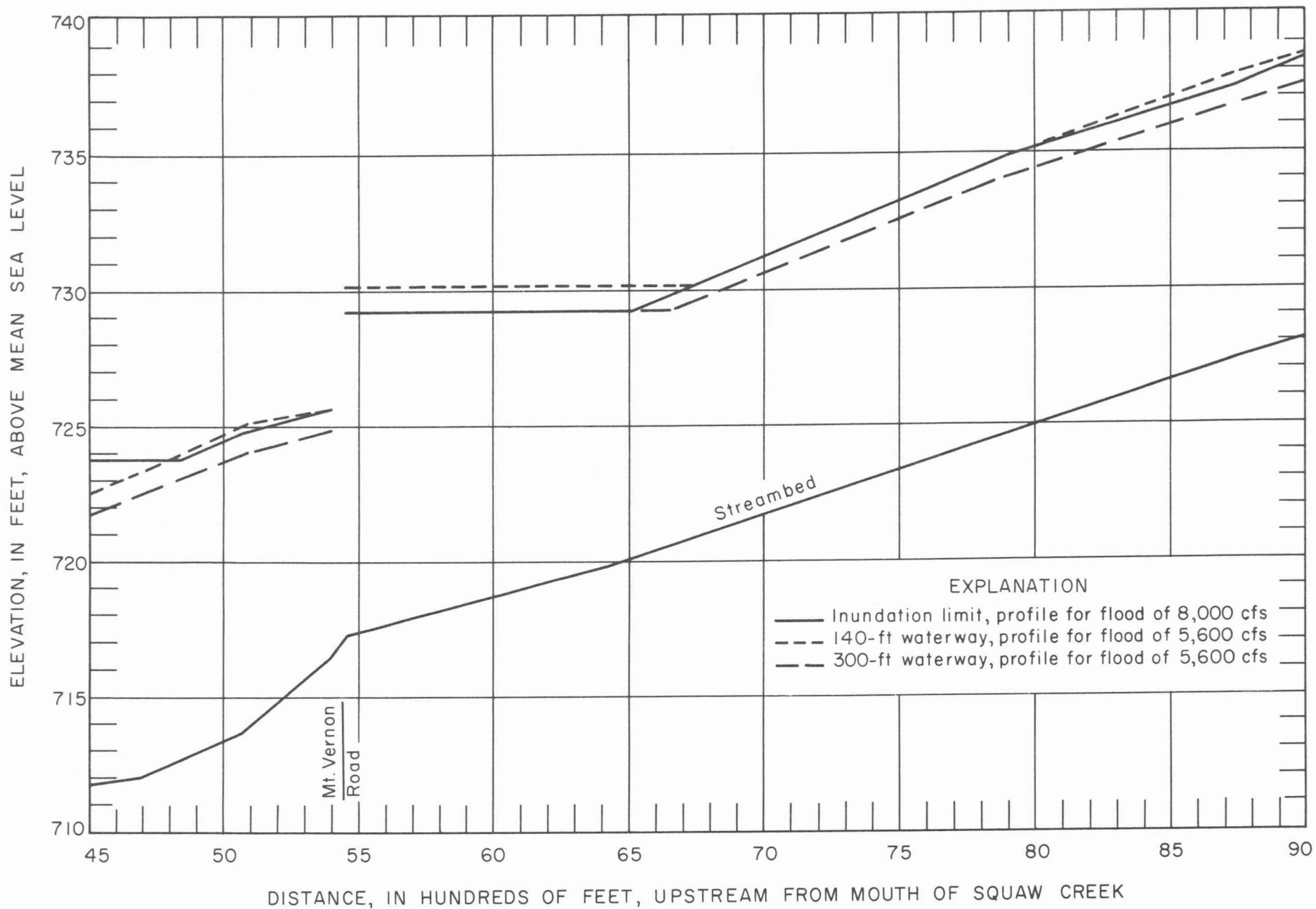
Figure 2. Flood profiles and streambed profile, station 45 to station 90, on Squaw Creek.
