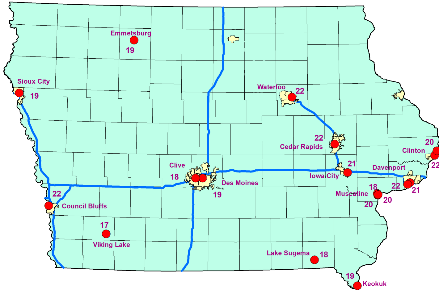
2020-2022 PM 2.5 24-hr Design Values ( \mu\text{g}/\text{m}^3 ) Source: EPA Design Value Report (AMP 480) 4/12/23. (The National Ambient Air Quality 24 hour Standard for PM 2.5 is 35 \mu\text{g}/\text{m}^3 .)
