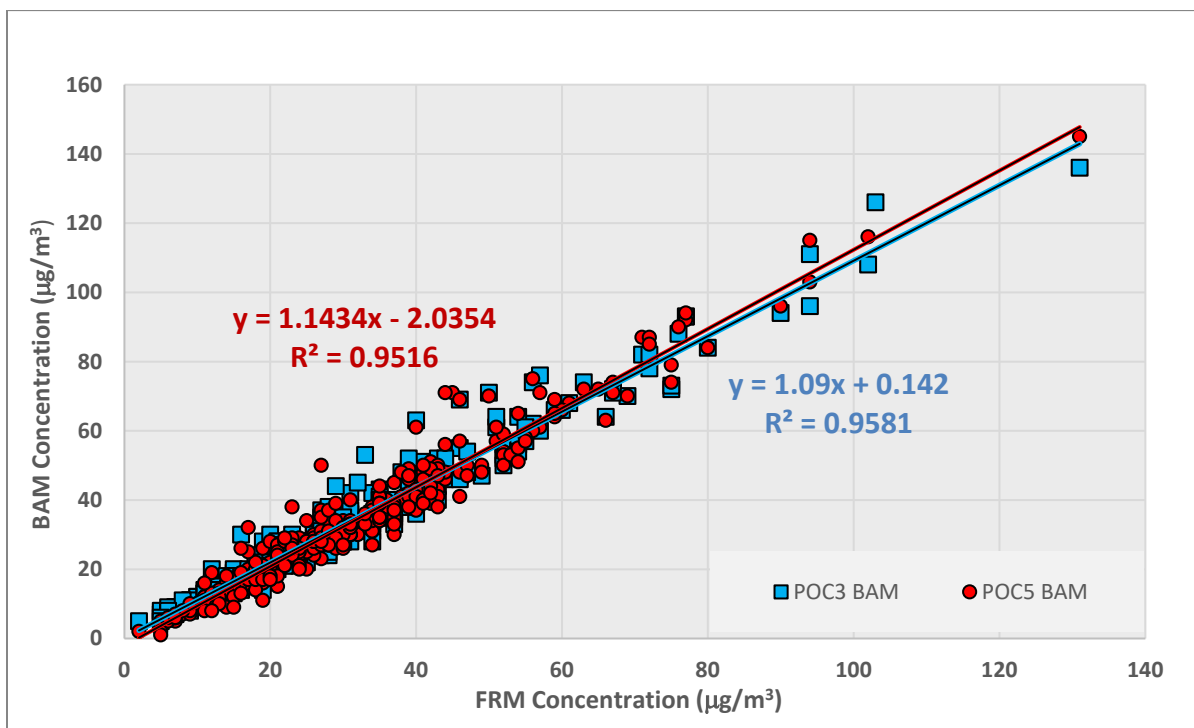
Figure K.3 Buffalo, Linwood Mining PM 10 BAMs vs FRM in 2022
