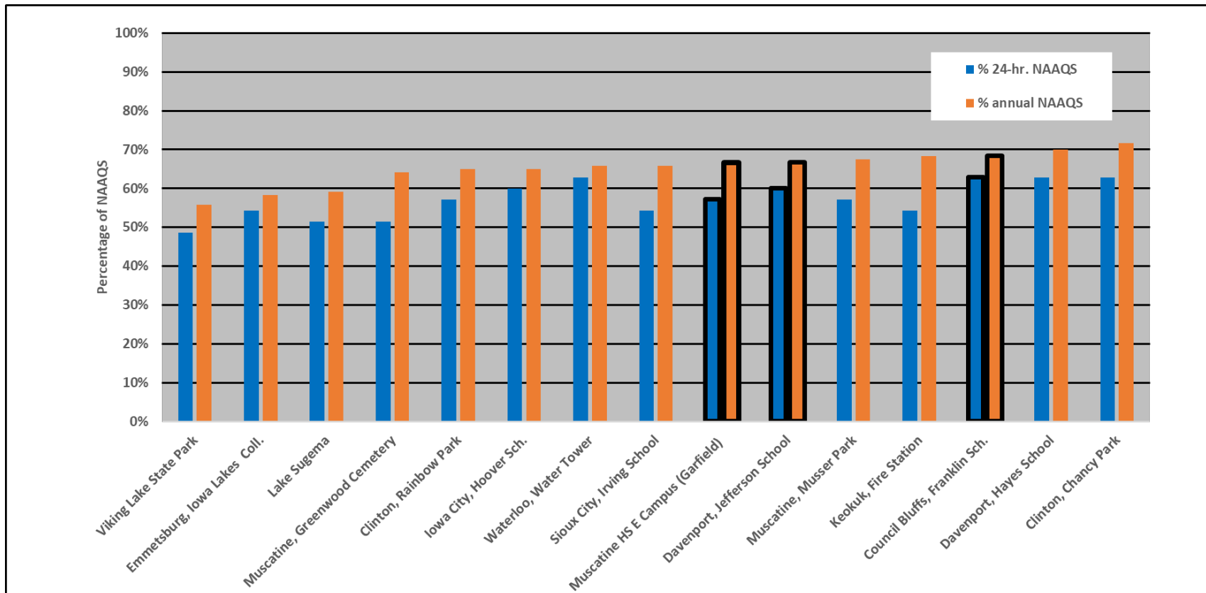
Figure K.1 SHL 2022 PM 2.5 Design Values as a percentage of the NAAQS. Collocated Monitors are outlined in black.
