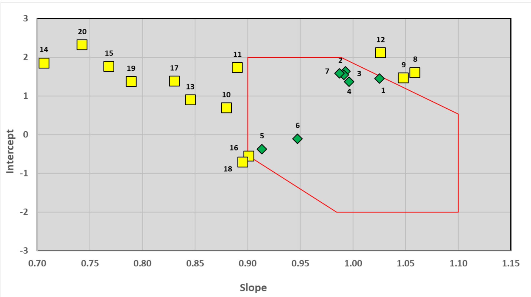
Figure K.2 2022 Continuous PM 2.5 Monitor Performance Relative to the Slope and Intercept Criteria in Part 53.
