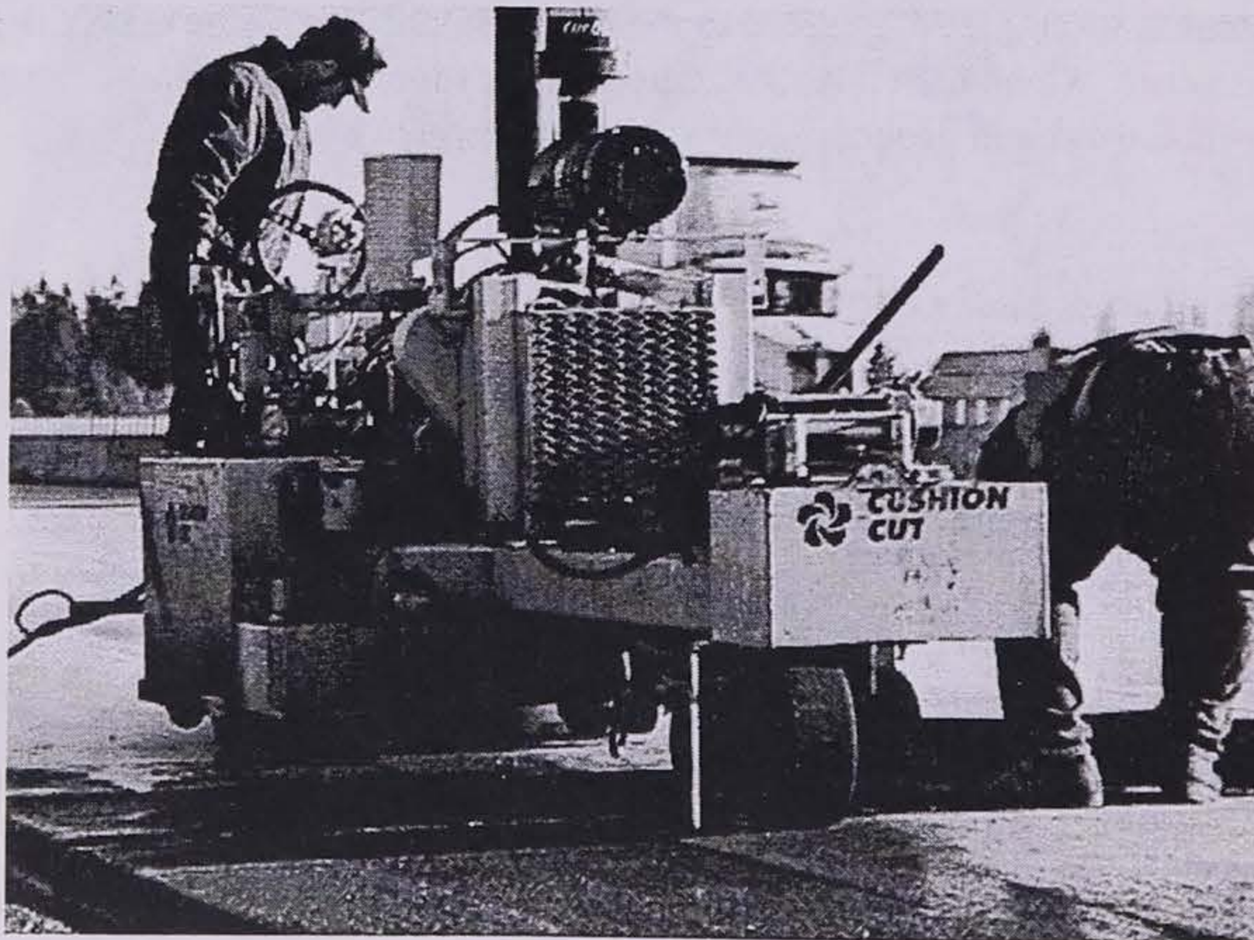
Figure 5.3 Pavement Grinding
