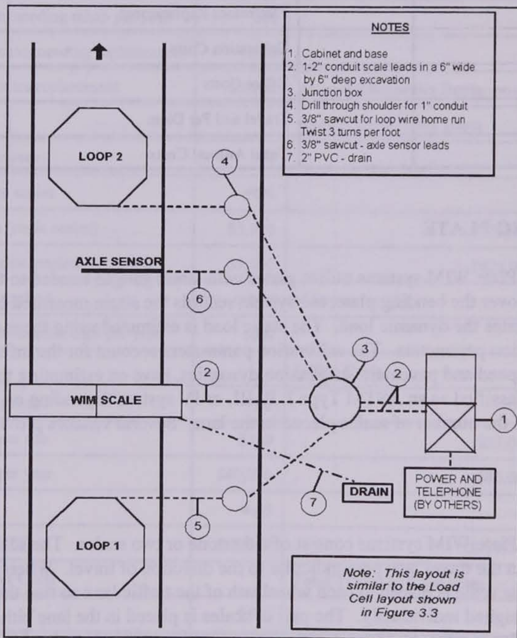
Figure 3.1 Example of Bending Plate System Layout
