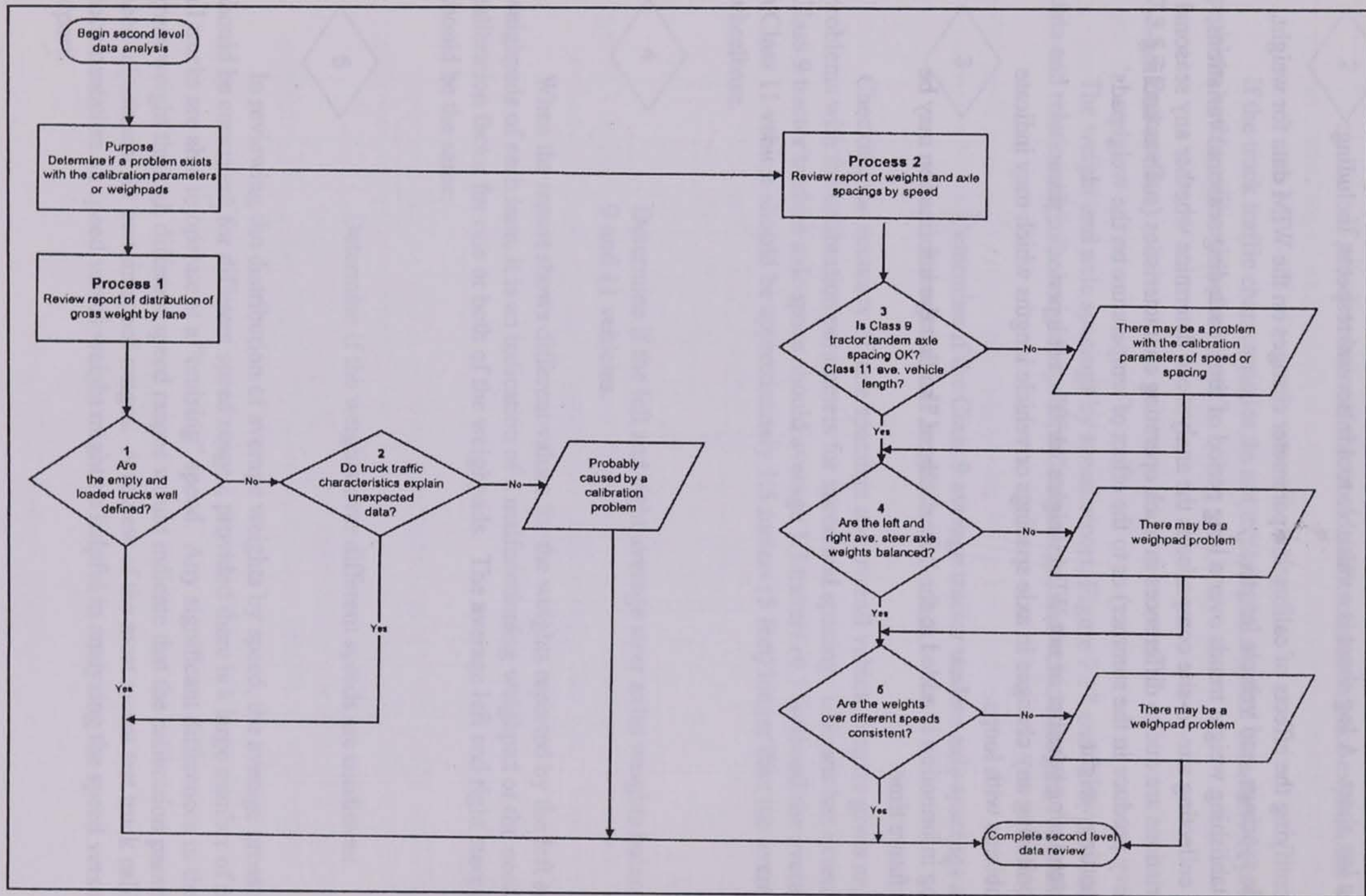
Figure 7.14 Second Level Data Review Flowchart
