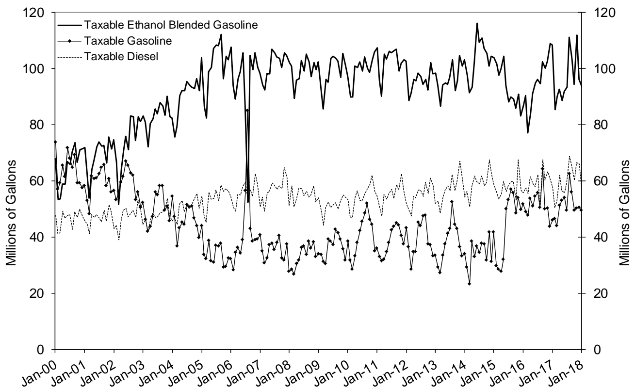
Figure 2. Iowa Monthly Taxable Ethanol Blended Gasoline, Gasoline, and Diesel Gallons: January 2000 – January 2018
