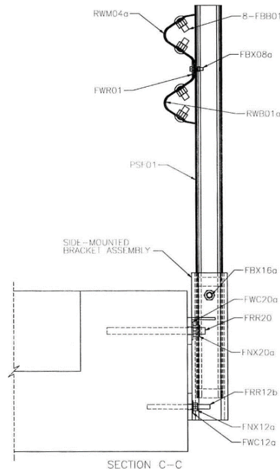
Figure 11. Side-Mounted Guardrail (FHWA Ref. B-264)
