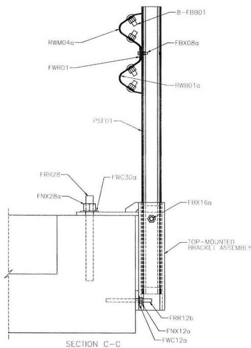
Figure 10. Top-Mounted Guardrail (FHWA Ref. B-262)
