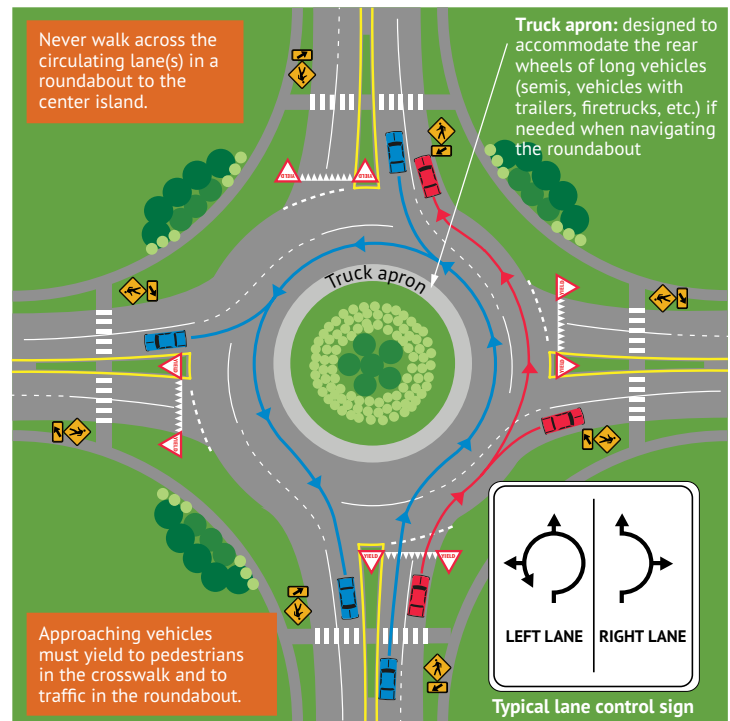
Figure 5.5: Multi-lane roundabout
