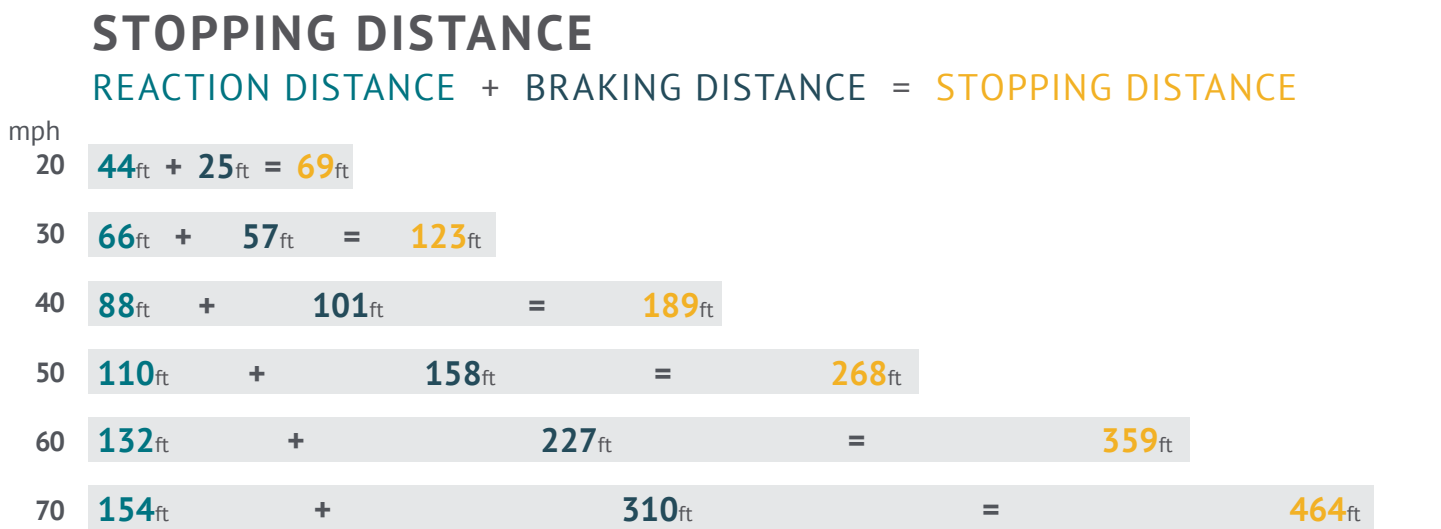
Figure 4. 1: Stopping distance
