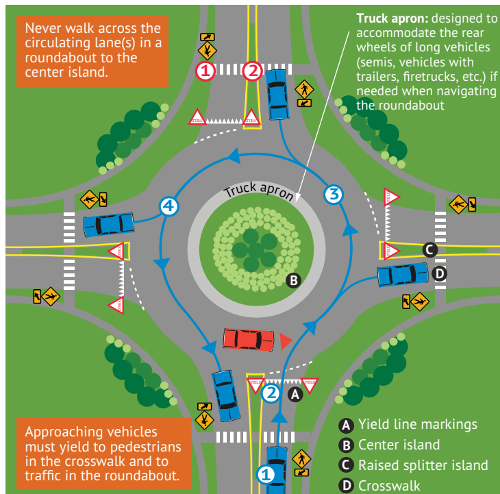
Figure 5.4: Single-lane roundabout
