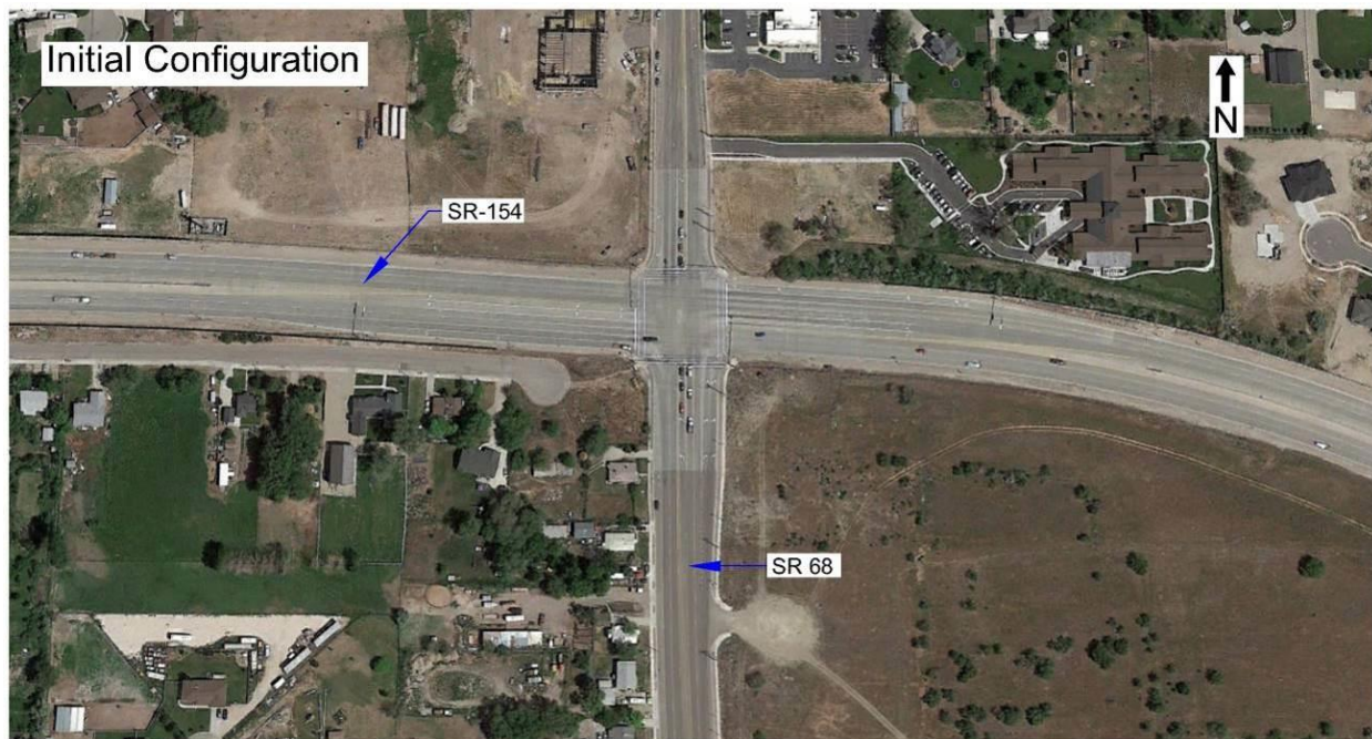
Figure C.2.2.1 Conventional signalized at-grade intersection at Bangerter Highway and SR-68 (Redwood Road)
