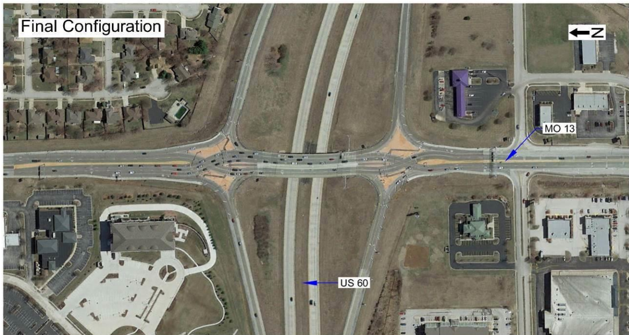
Figure C.3.1.7 Final configuration of DDI at US 60/160 (James River Freeway) and MO 13 (Kansas Expressway)
