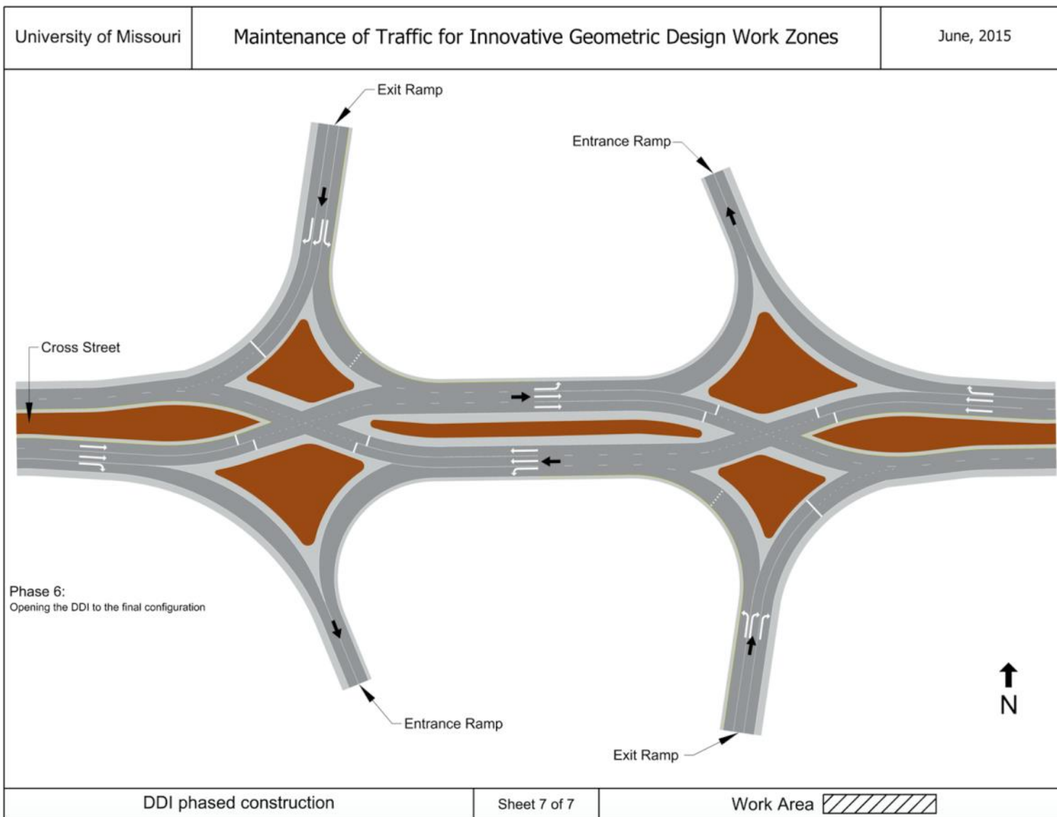
Figure D.1.3.7 DDI phased construction final configuration
