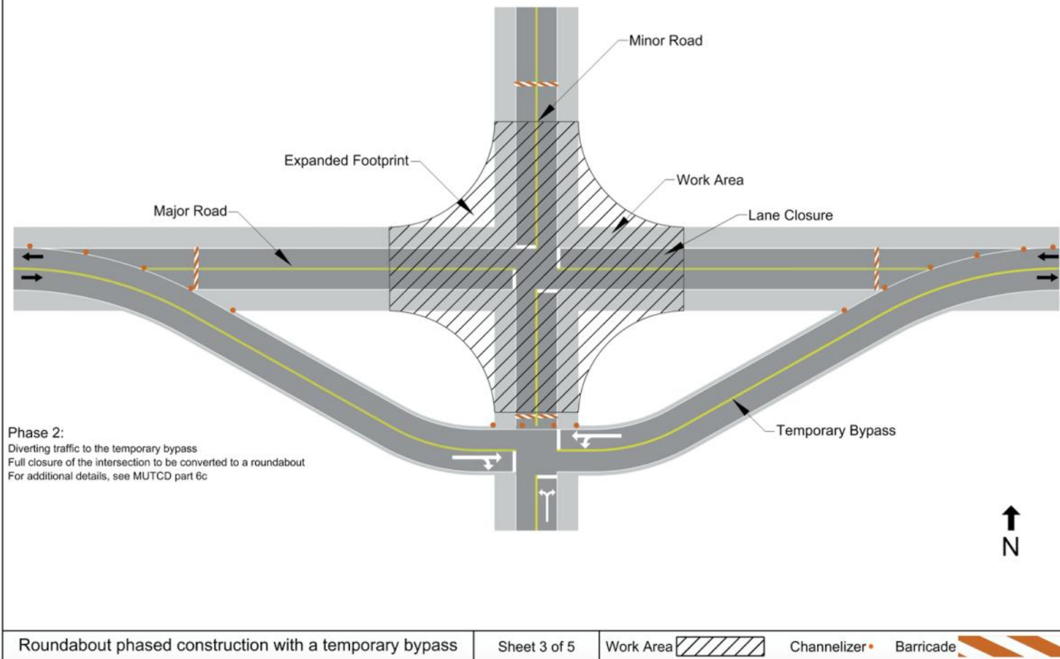
Figure D.1.1.8 Roundabout phased construction with a temporary bypass Phase 2 (construction of roundabout)
