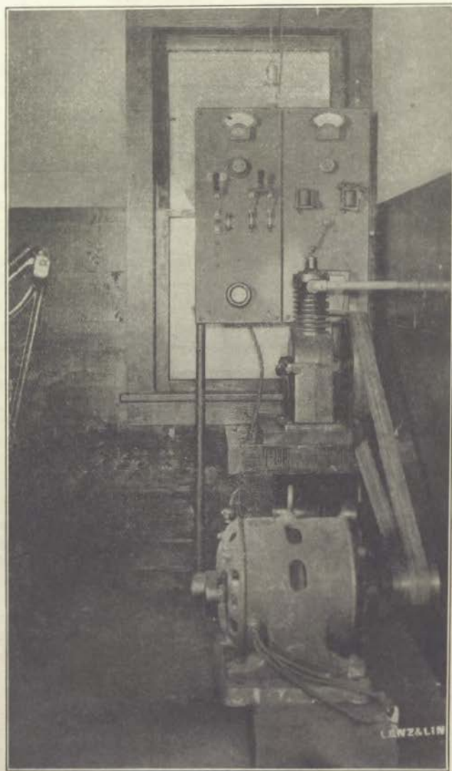
Sabula Hatchery, engine room.
