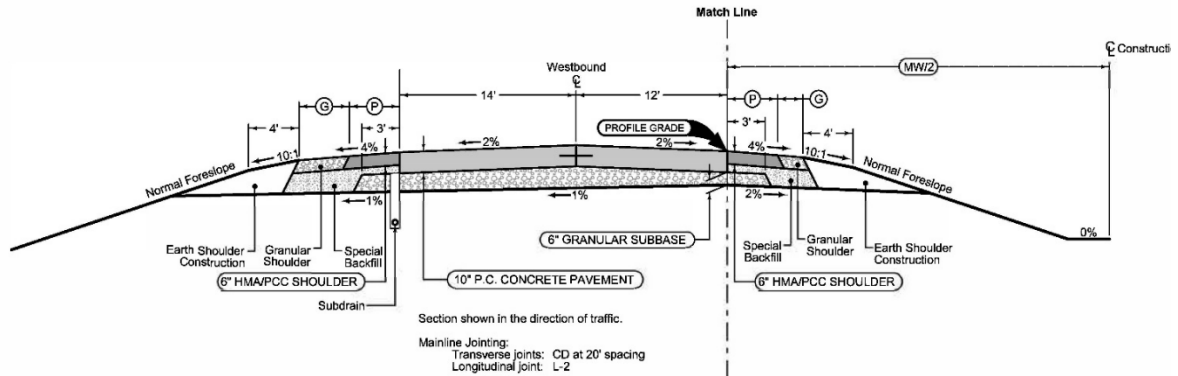
Figure 2. U.S. 20 Cross Section
