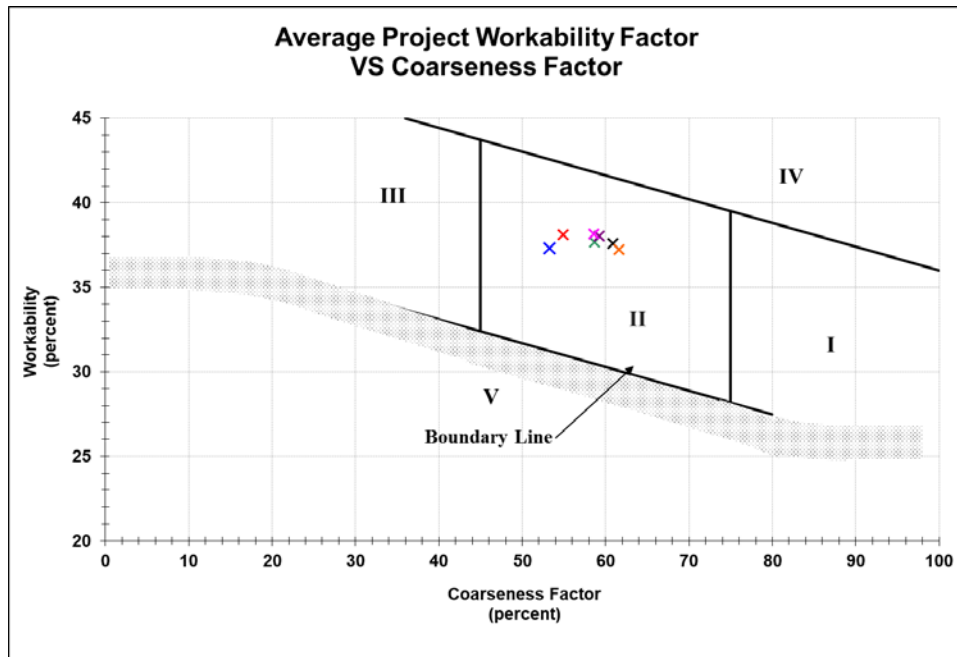
Figure 11: Weekly Averages Shilstone Coarseness/Workability Factors
