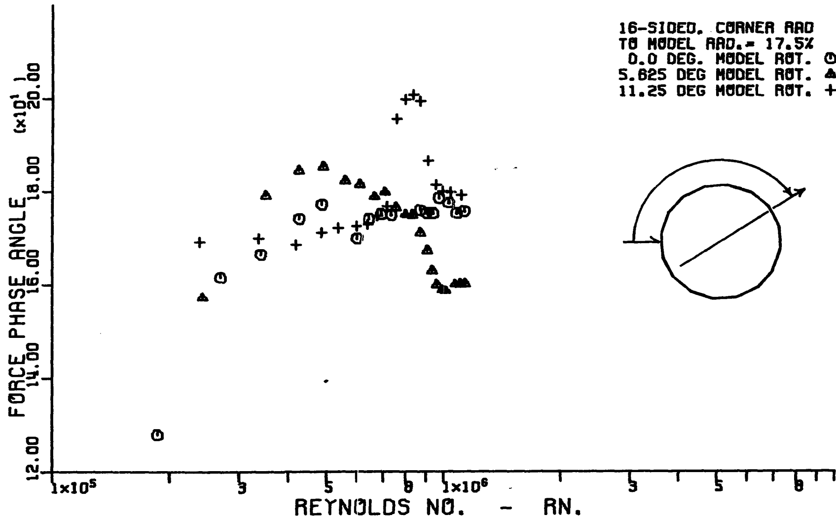
Figure 137. Variation of corrected cross-flow force phase angle with corrected cross-flow Reynolds number for a hexdecagonal cylinder having a corner radius equal to 17.5 percent of the radius of the inscribed circular cylinder.
