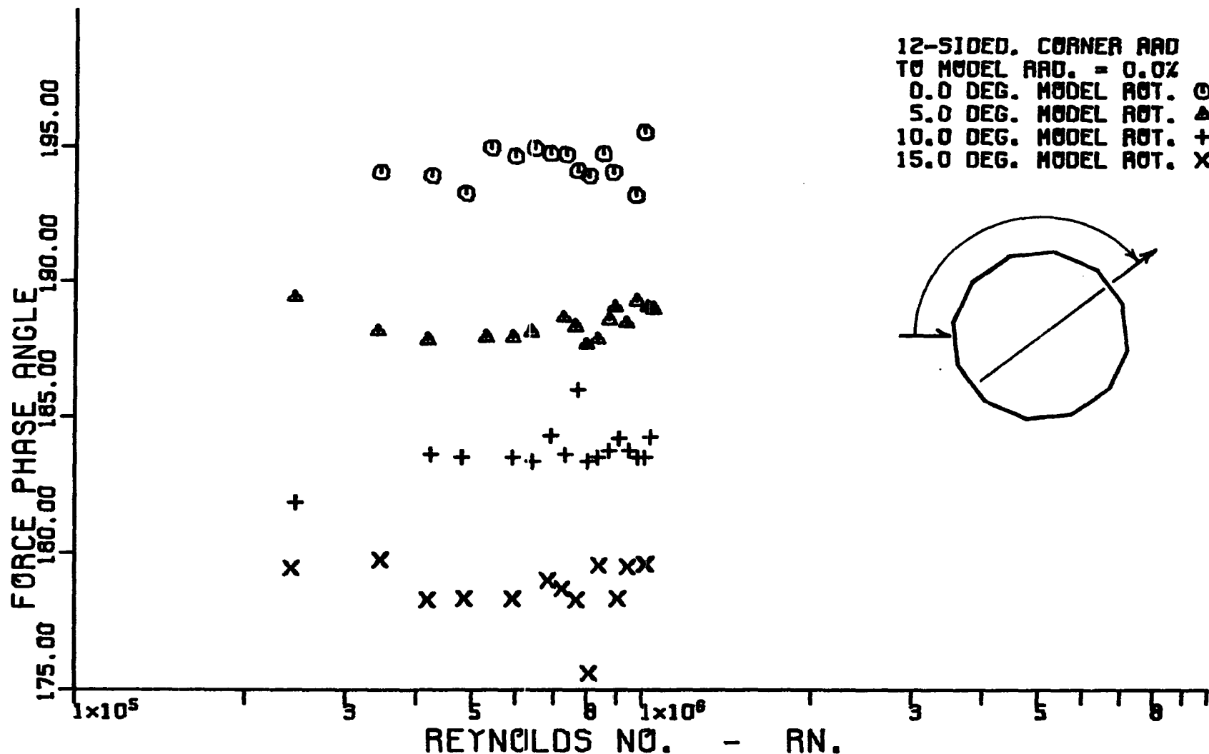
Figure 119. Variation of corrected cross-flow force phase angle with corrected cross-flow Reynolds number for a dodecagonal cylinder having a corner radius equal to 0.0 percent of the radius of the inscribed circular cylinder.
