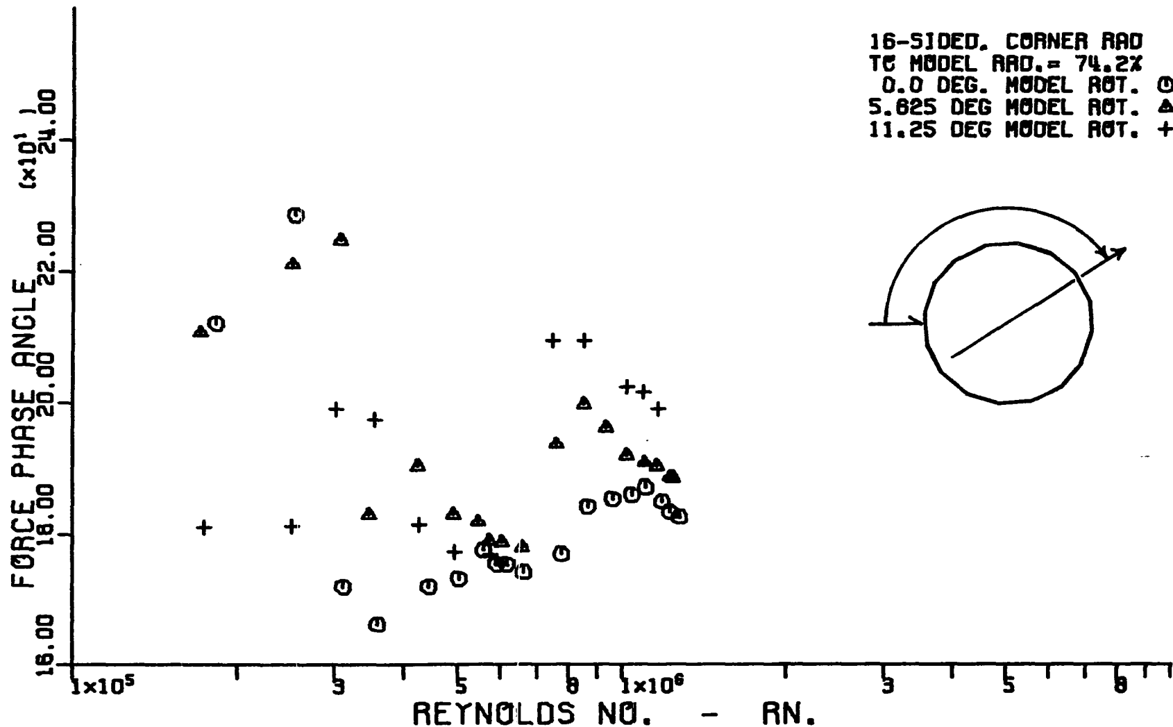
Figure 145. Variation of corrected cross-flow force phase angle with corrected cross-flow Reynolds number for a hexadecagonal cylinder having a corner radius equal to 74.2 percent of the radius of the inscribed circular cylinder.
