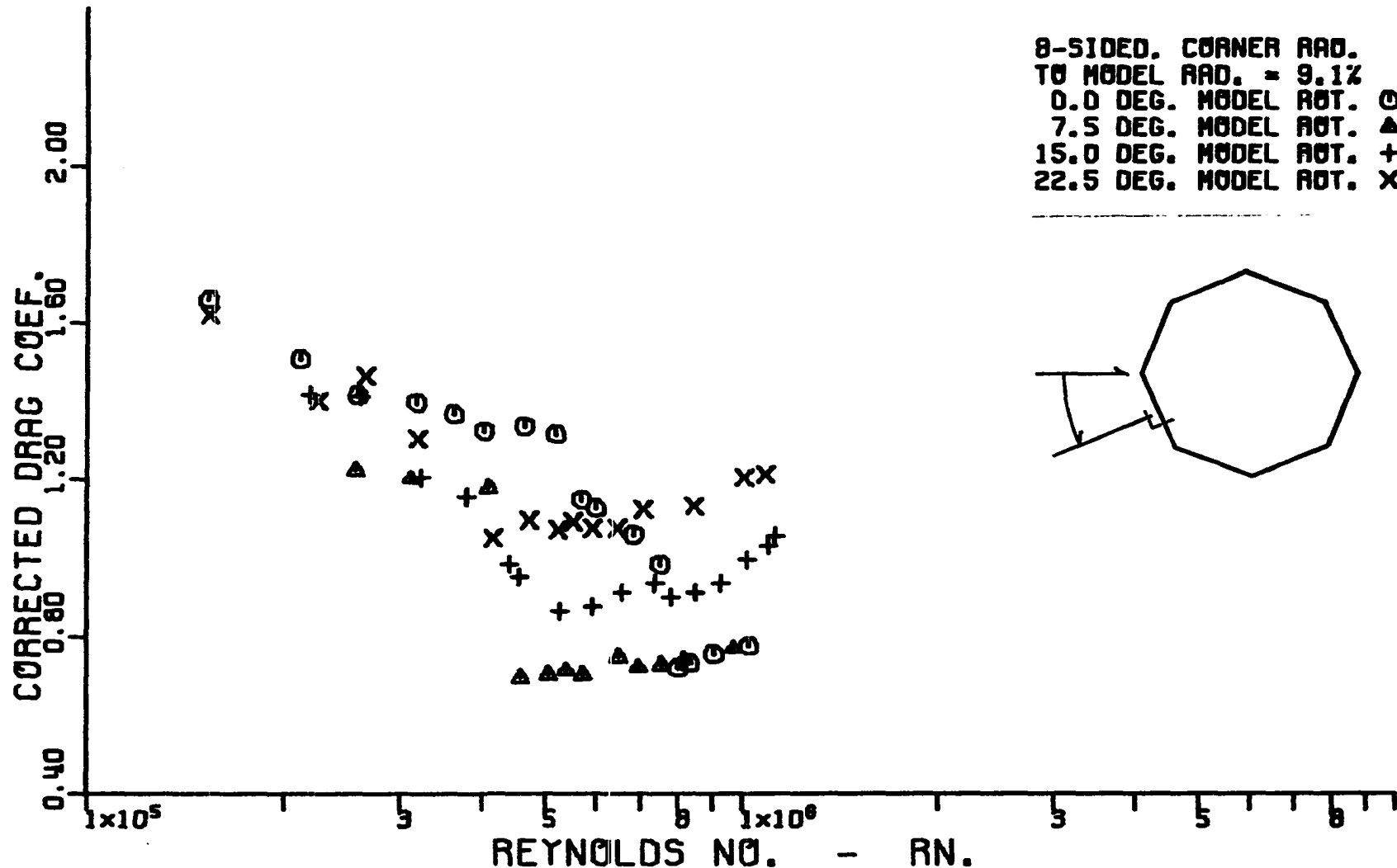
Figure 38. Variation of corrected cross-flow drag coefficient with corrected cross-flow Reynolds number for an octagonal cylinder having a corner radius equal to 9.1 percent of the radius of the inscribed circular cylinder.
