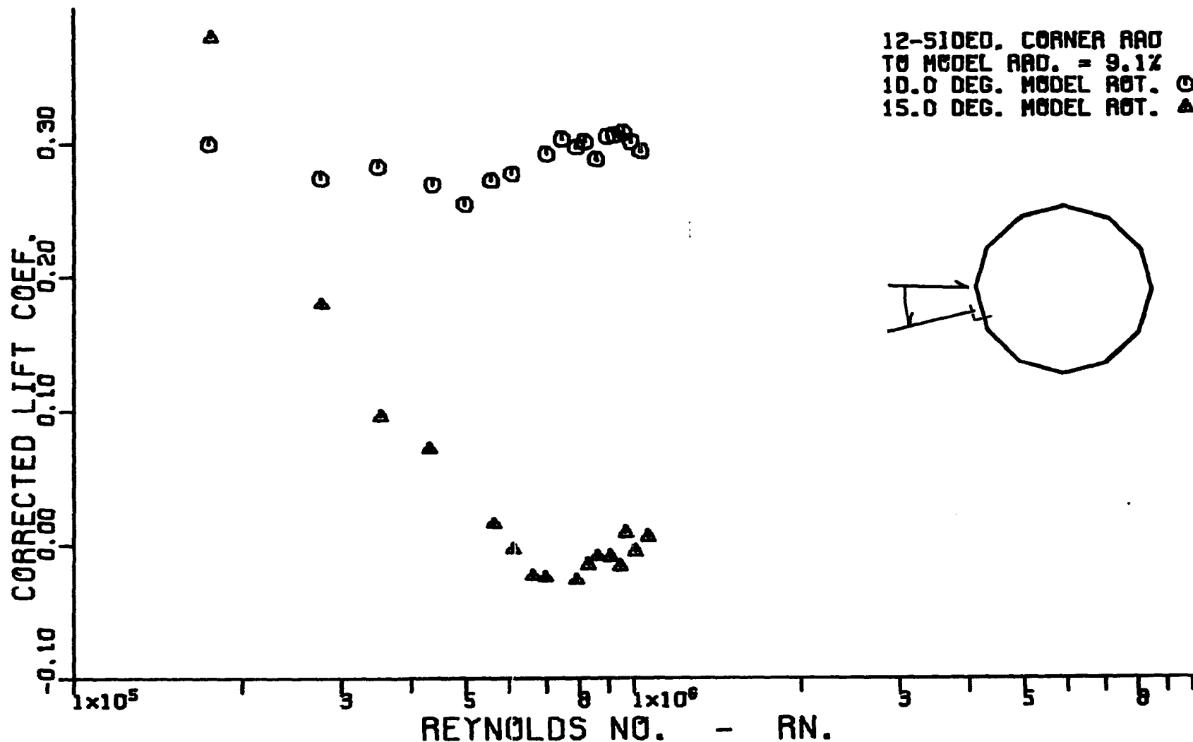
Figure 85. Variation of corrected cross-flow lift coefficient with corrected cross-flow Reynolds number for a dodecagonal cylinder having a corner radius equal to 9.1 percent of the radius of the inscribed circular cylinder.
