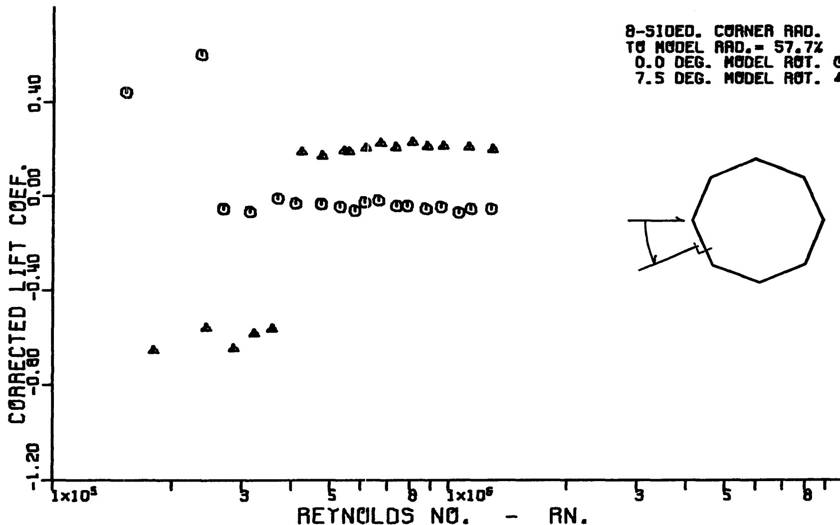
Figure 78. Variation of corrected cross-flow lift coefficient with corrected cross-flow Reynolds number for an octagonal cylinder having a corner radius equal to 57.7 percent of the radius of the inscribed circular cylinder.
