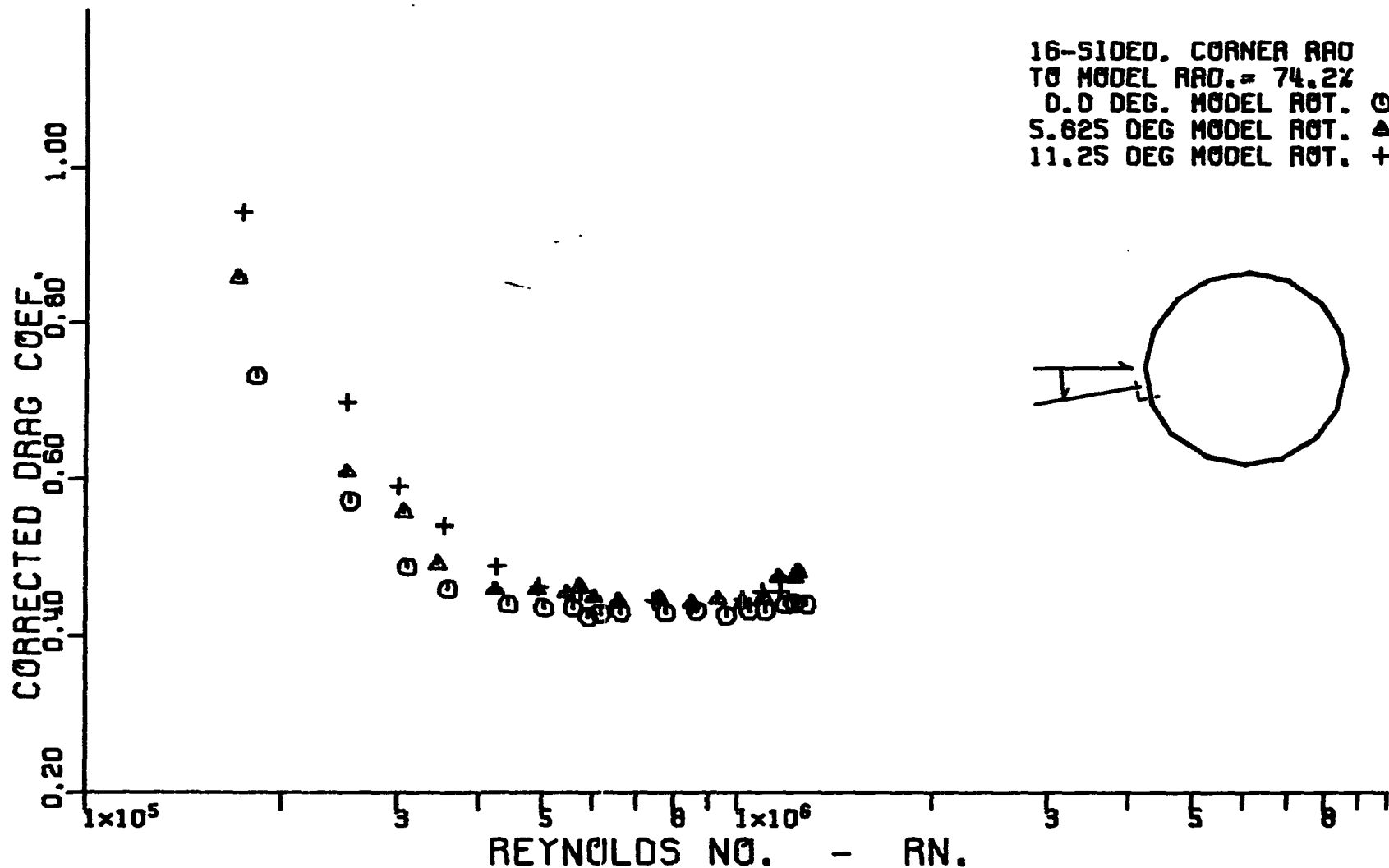
Figure 57. Variation of corrected cross-flow drag coefficient with corrected cross-flow Reynolds number for a hexdecagonal cylinder having a corner radius equal to 74.2 percent of the radius of the inscribed circular cylinder.
