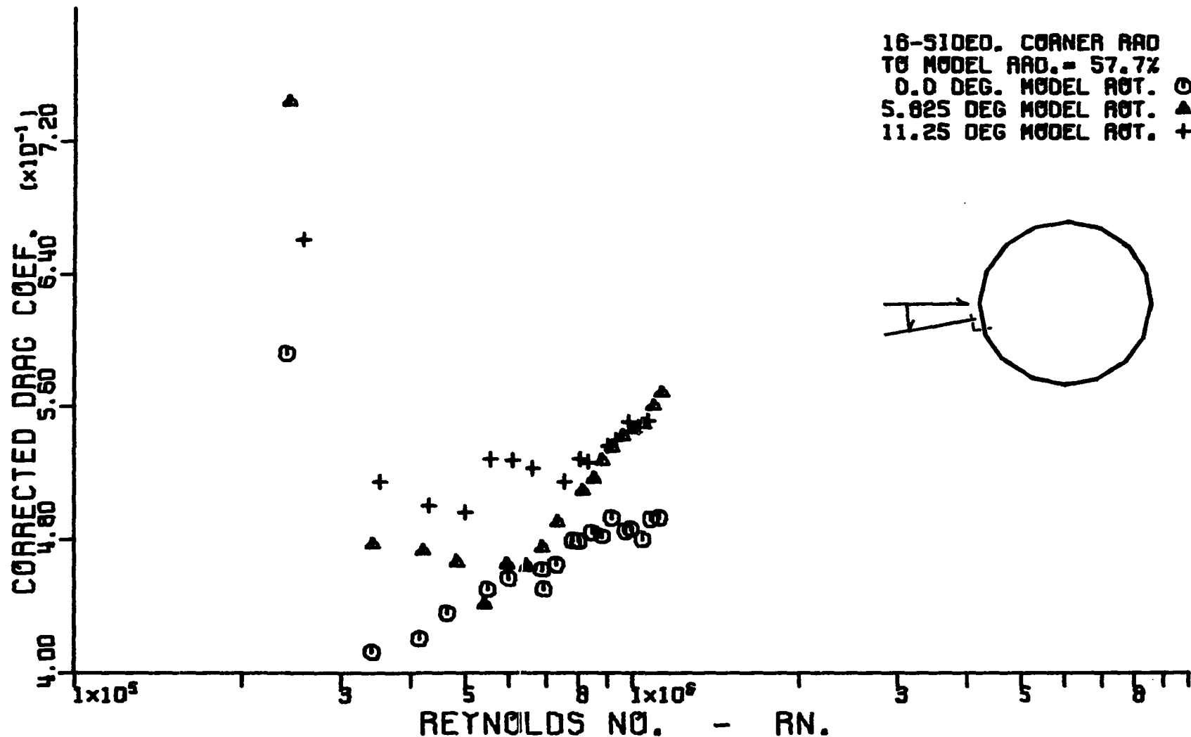
Figure 56. Variation of corrected cross-flow drag coefficient with corrected cross-flow Reynolds number for a hexadecagonal cylinder having a corner radius equal to 57.7 percent of the radius of the inscribed circular cylinder.
