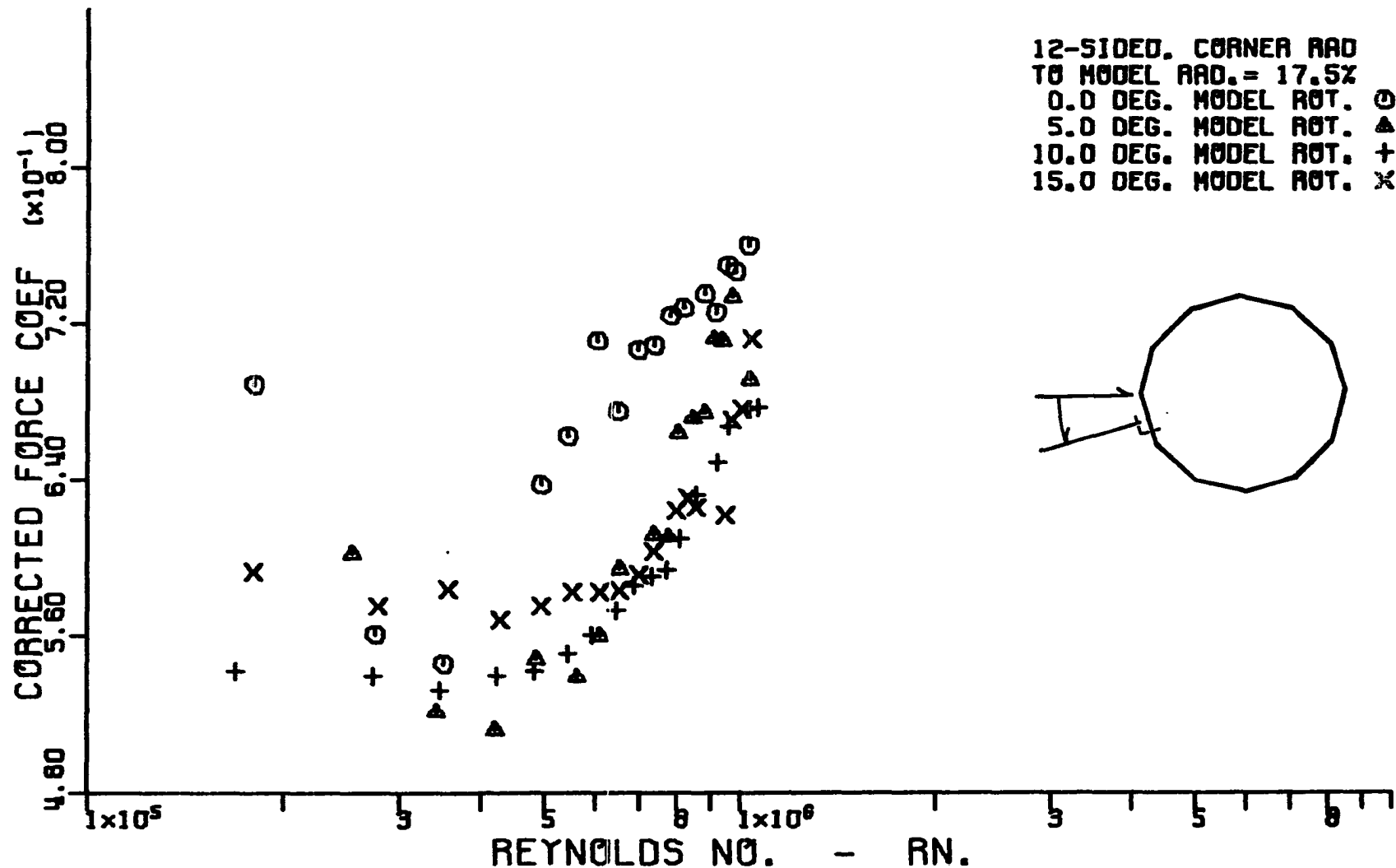
Figure 122. Variation of corrected cross-flow force coefficient with corrected cross-flow Reynolds number for a dodecagonal cylinder having a corner radius equal to 17.5 percent of the radius of the inscribed circular cylinder.
