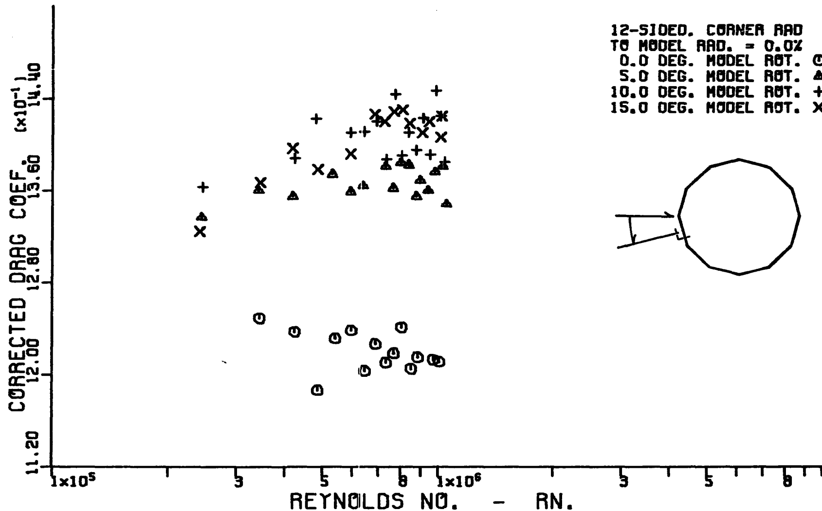
Figure 44. Variation of corrected cross-flow drag coefficient with corrected cross-flow Reynolds number for a dodecagonal cylinder having a corner radius equal to 0.0 percent of the radius of the inscribed circular cylinder.
