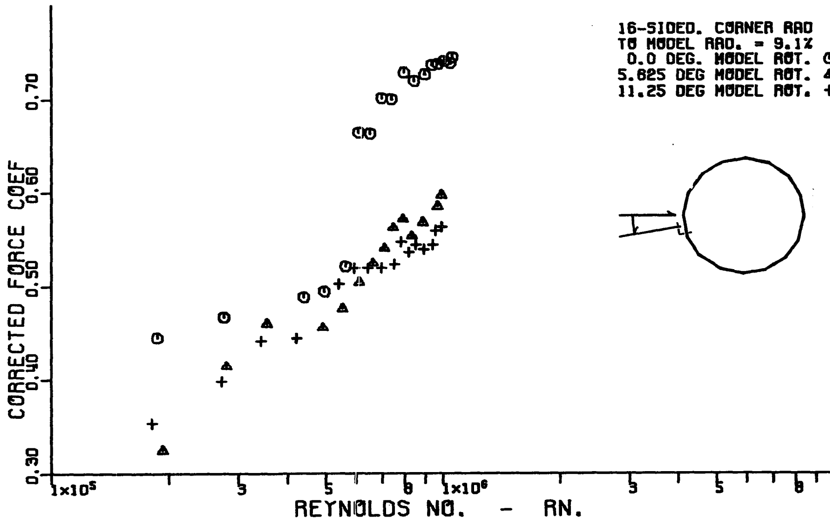
Figure 134. Variation of corrected cross-flow force coefficient with corrected cross-flow Reynolds number for a hexadecagonal cylinder having a corner radius equal to 9.1 percent of the radius of the inscribed circular cylinder.
