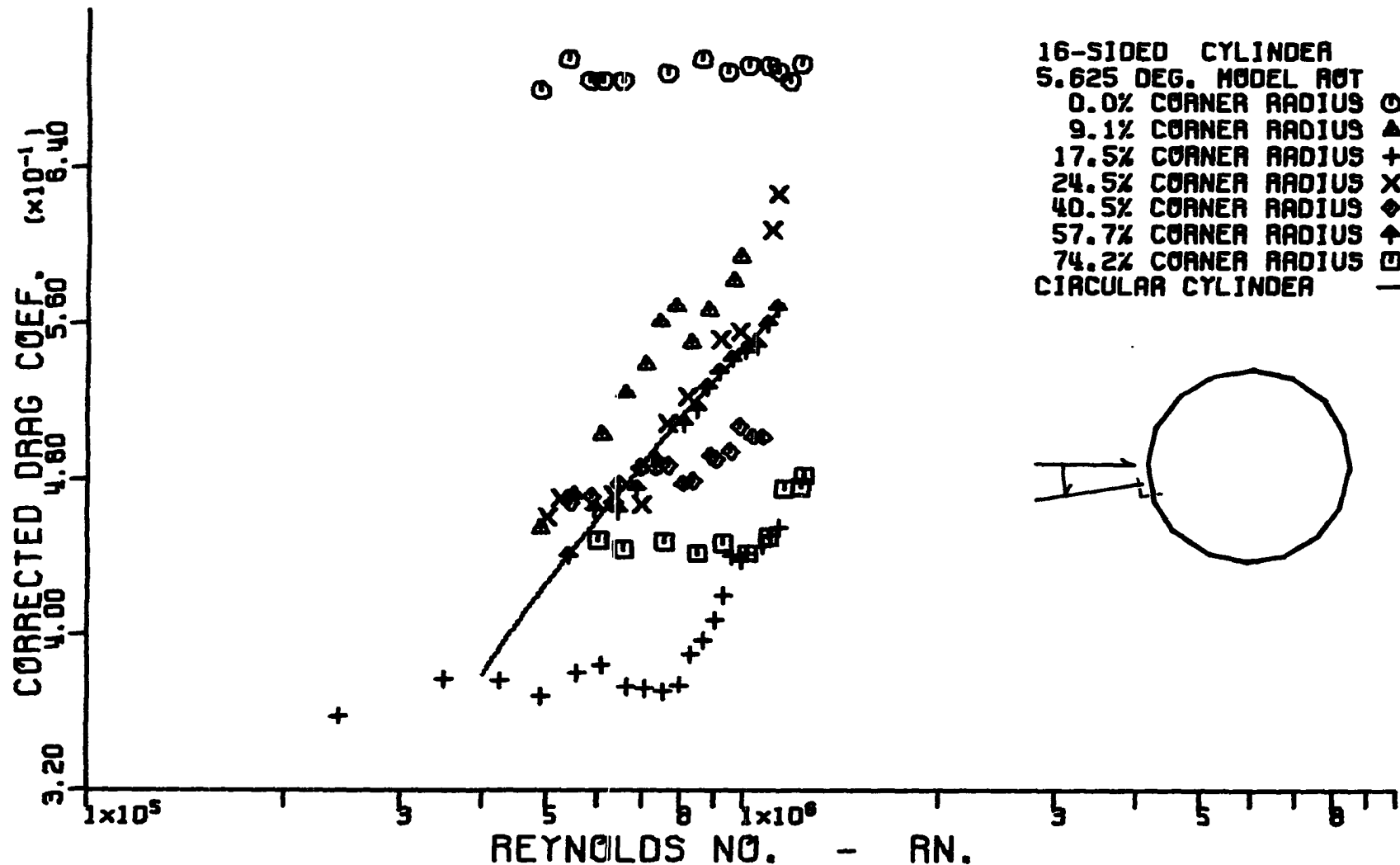
Figure 35. Variation of corrected cross-flow drag coefficient with corrected cross-flow Reynolds number for hexdecagonal cylinders. Models orientated at 5.6^\circ with respect to the relative wind.
