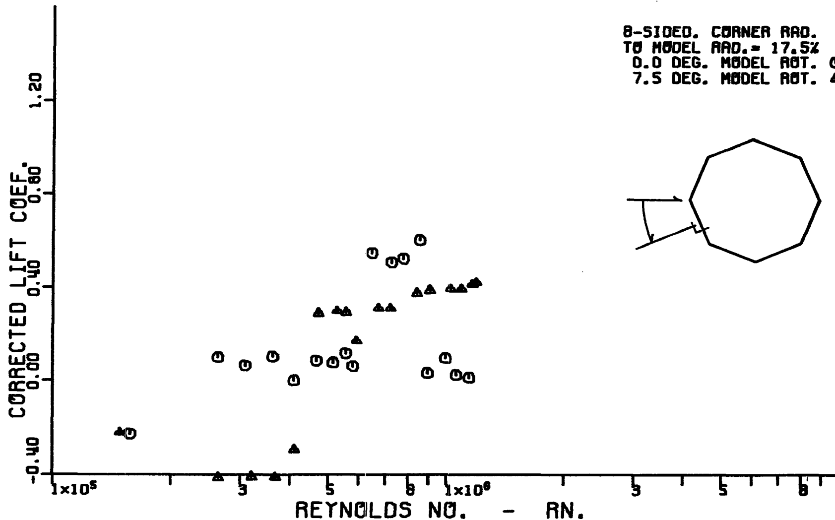
Figure 72. Variation of corrected cross-flow lift coefficient with corrected cross-flow Reynolds number for an octagonal cylinder having a corner radius equal to 17.5 percent of the radius of the inscribed circular cylinder.
