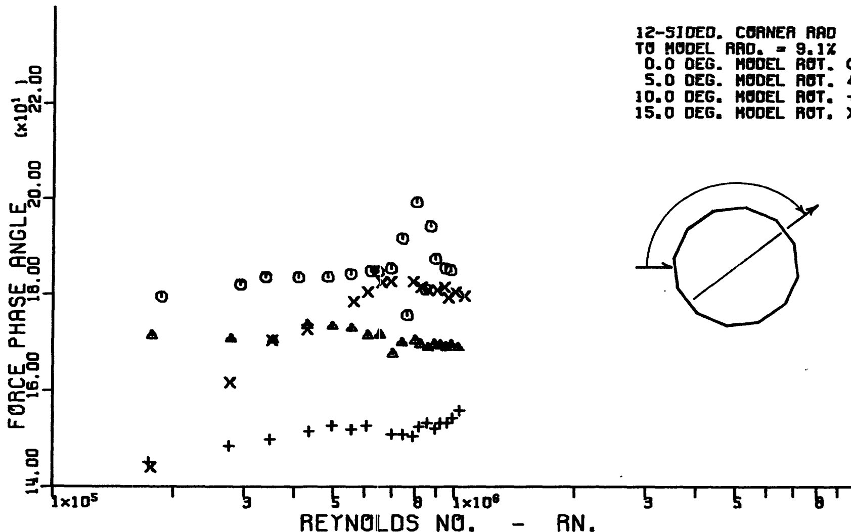
Figure 121. Variation of corrected cross-flow force phase angle with corrected cross-flow Reynolds number for a dodecagonal cylinder having a corner radius equal to 9.1 percent of the radius of the inscribed circular cylinder.
