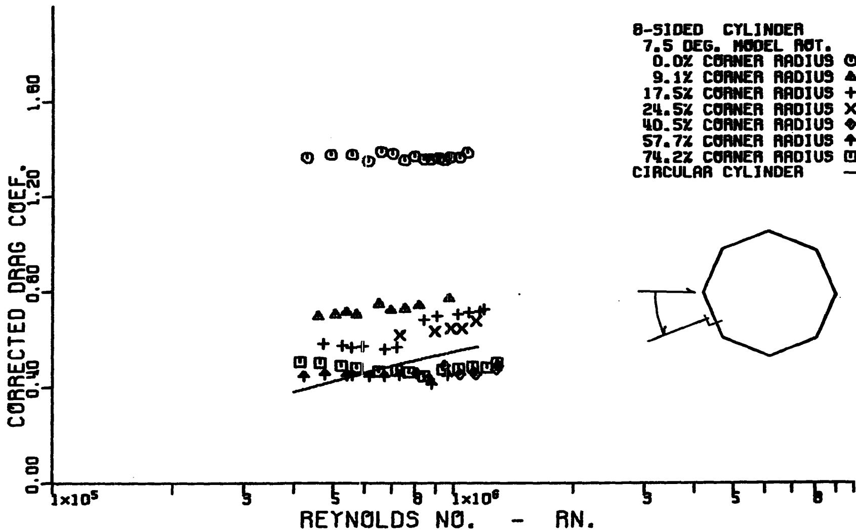
Figure 27. Variation of corrected cross-flow drag coefficient with corrected cross-flow Reynolds number for octagonal cylinders. Models orientated at 7.5° with respect to the relative wind.
