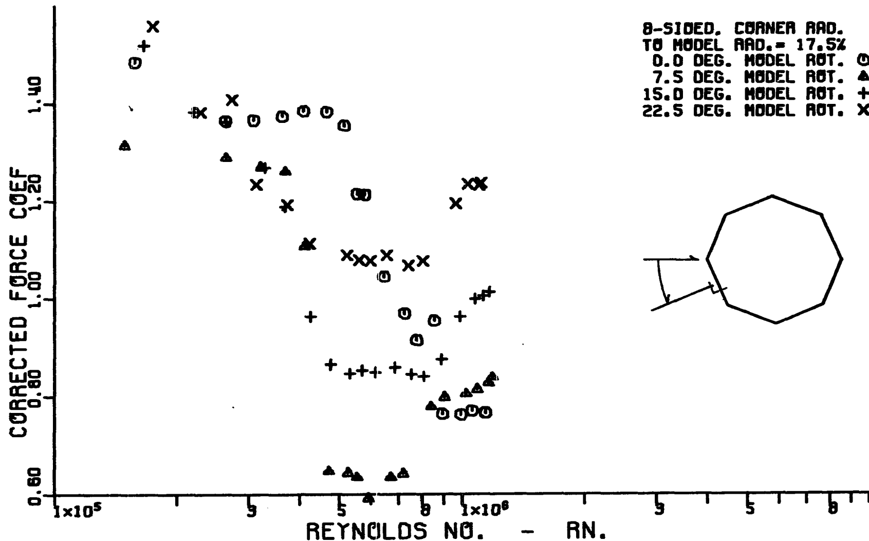
Figure 108. Variation of corrected cross-flow force coefficient with corrected cross-flow Reynolds number for an octagonal cylinder having a corner radius equal to 17.5 percent of the radius of the inscribed circular cylinder.
