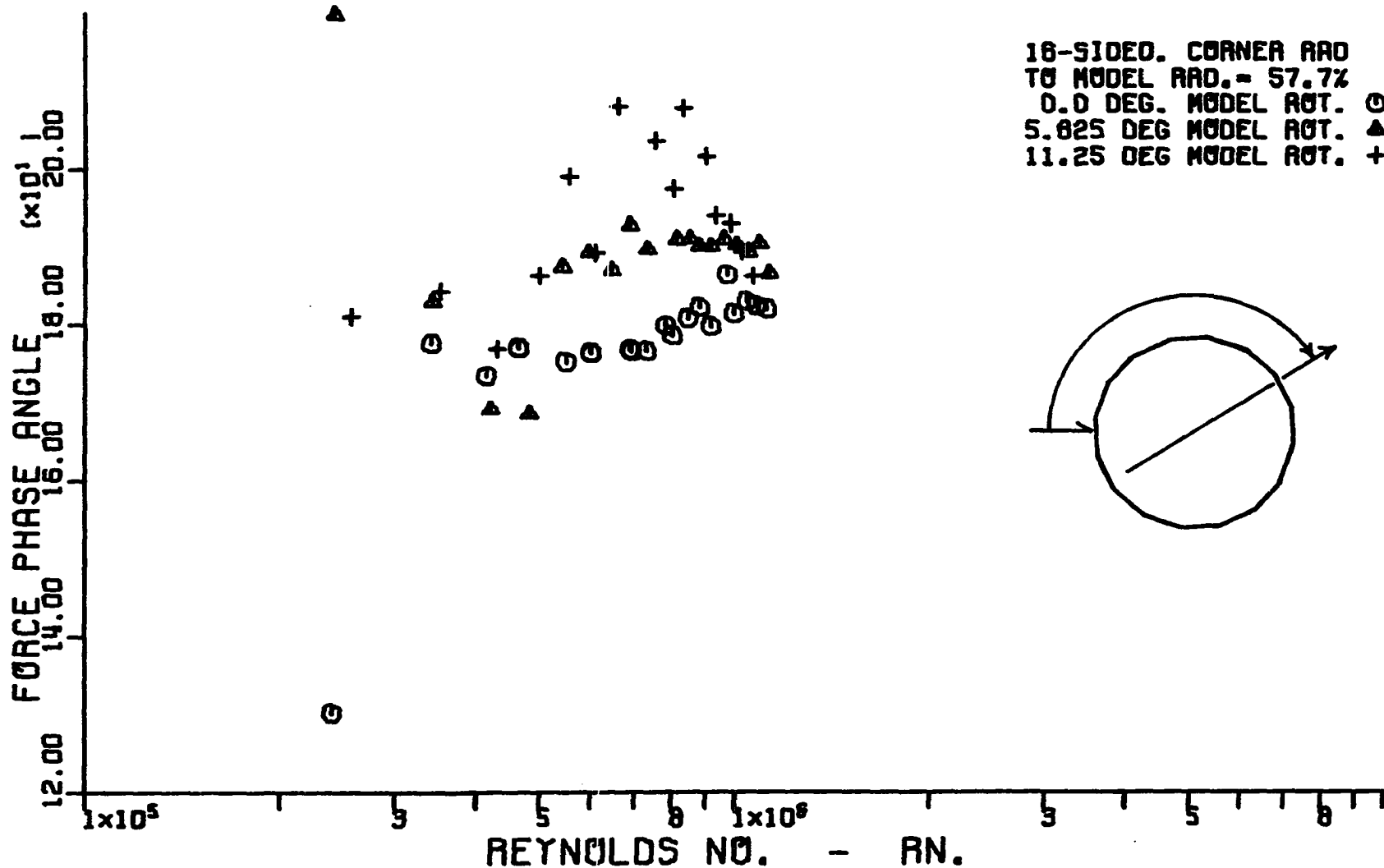
Figure 143. Variation of corrected cross-flow force phase angle with corrected cross-flow Reynolds number for a hexadecagonal cylinder having a corner radius equal to 57.7 percent of the radius of the inscribed circular cylinder.
