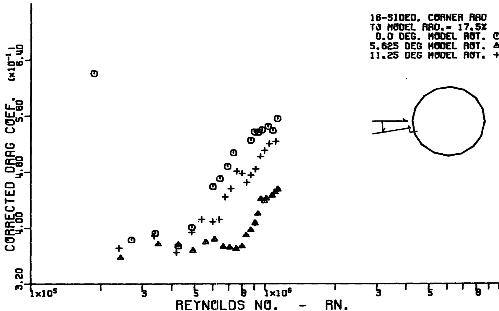
Figure 53. Variation of corrected cross-flow drag coefficient with corrected cross-flow Reynolds number for a hexadecagonal cylinder having a corner radius equal to 17.5 percent of the radius of the inscribed circular cylinder.
