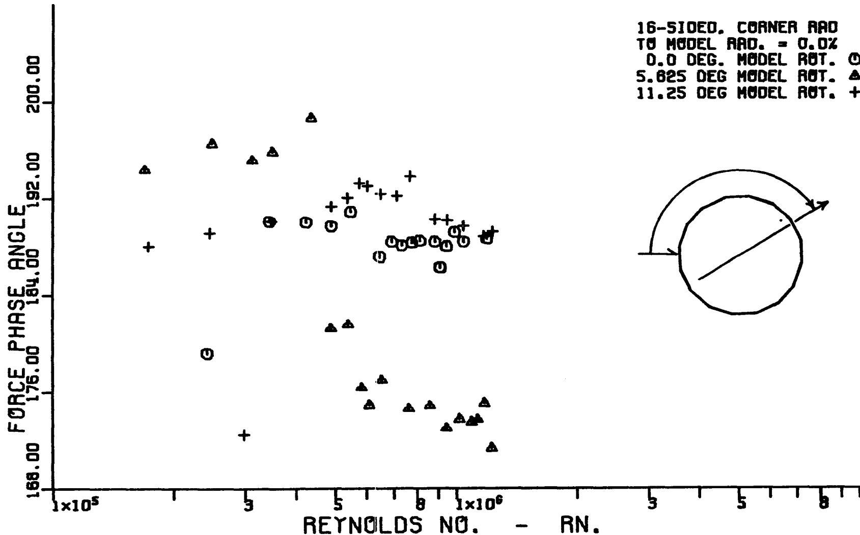
Figure 133. Variation of corrected cross-flow phase angle with corrected cross-flow Reynolds number for a hexdecagonal cylinder having a corner radius equal to 0.0 percent of the radius of the inscribed circular cylinder.
