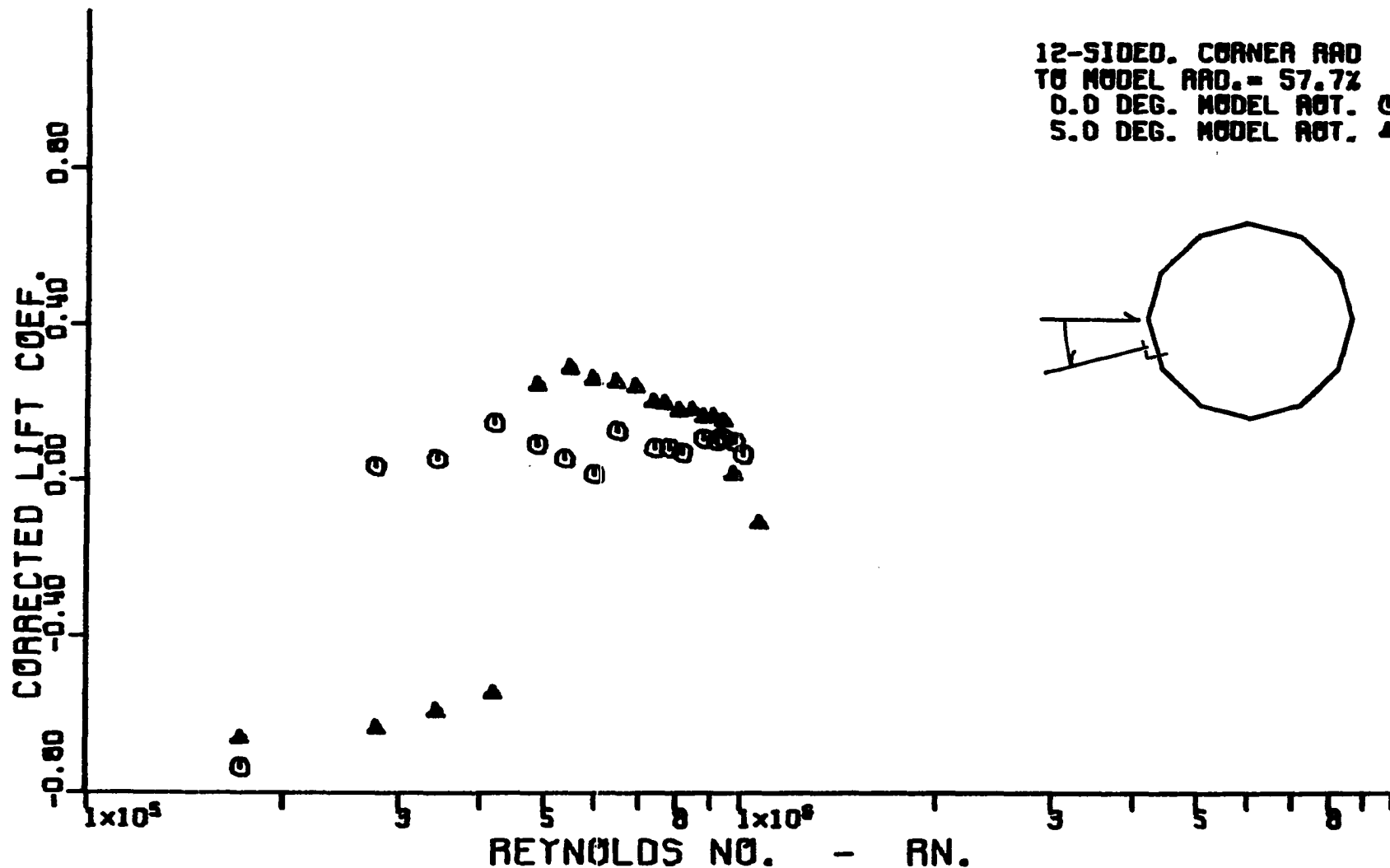
Figure 92. Variation of corrected cross-flow lift coefficient with corrected cross-flow Reynolds number for a dodecagonal cylinder having a corner radius equal to 57.7 percent of the radius of the inscribed circular cylinder.
