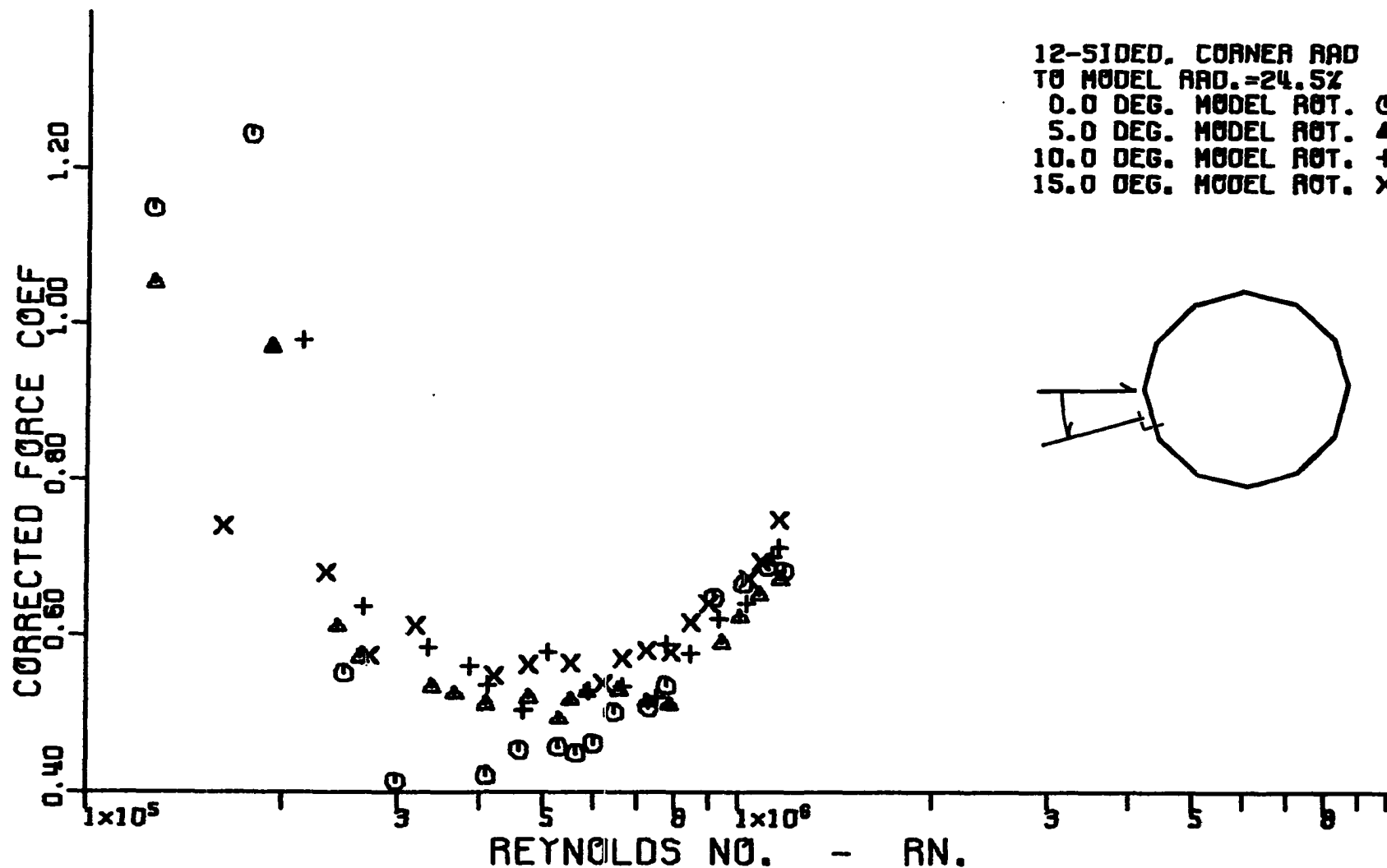
Figure 124. Variation of corrected cross-flow force coefficient with corrected cross-flow Reynolds number for a dodecagonal cylinder having a corner radius equal to 24.5 percent of the radius of the inscribed circular cylinder.
