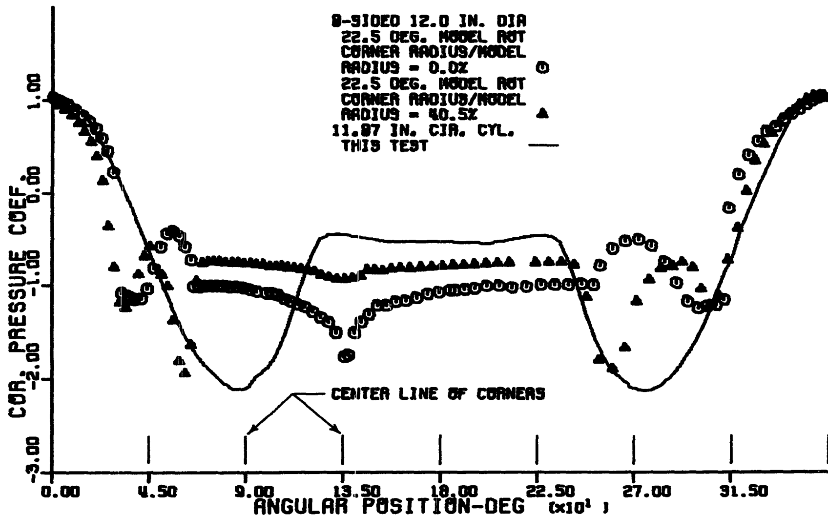
Figure 64. Variation of corrected pressure coefficient with change in angular position from the forward stagnation point for a circular cylinder and two octagonal cylinders, 0.0 and 40.5 percent corner radii, at 22.5° model rotation. Cylinders have corrected Reynolds numbers of 1,000,000.
