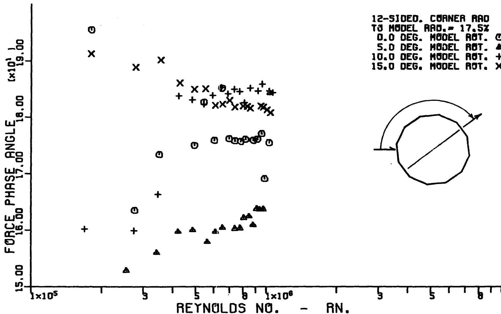
Figure 123. Variation of corrected cross-flow force phase angle with corrected cross-flow Reynolds number for a dodecagonal cylinder having a corner radius equal to 17.5 percent of the radius of the inscribed circular cylinder.
