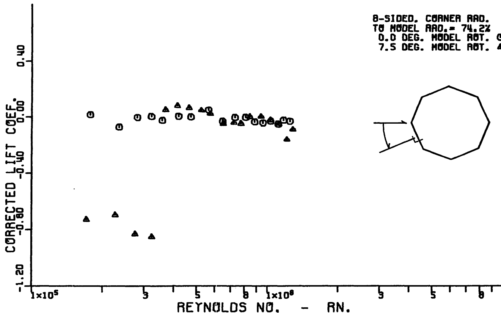
Figure 80. Variation of corrected cross-flow lift coefficient with corrected cross-flow Reynolds number for an octagonal cylinder having a corner radius equal to 74.2 percent of the radius of the inscribed circular cylinder.
