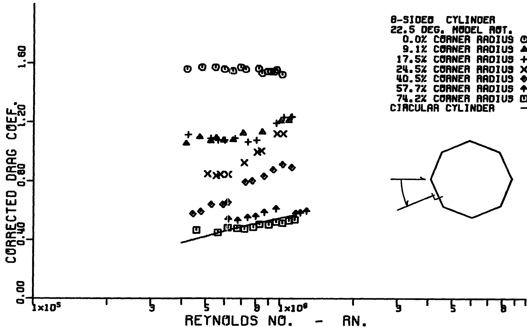
Figure 29. Variation of corrected cross-flow drag coefficient with corrected cross-flow Reynolds number for octagonal cylinders. Models orientated at 22.5° with respect to the relative wind.
