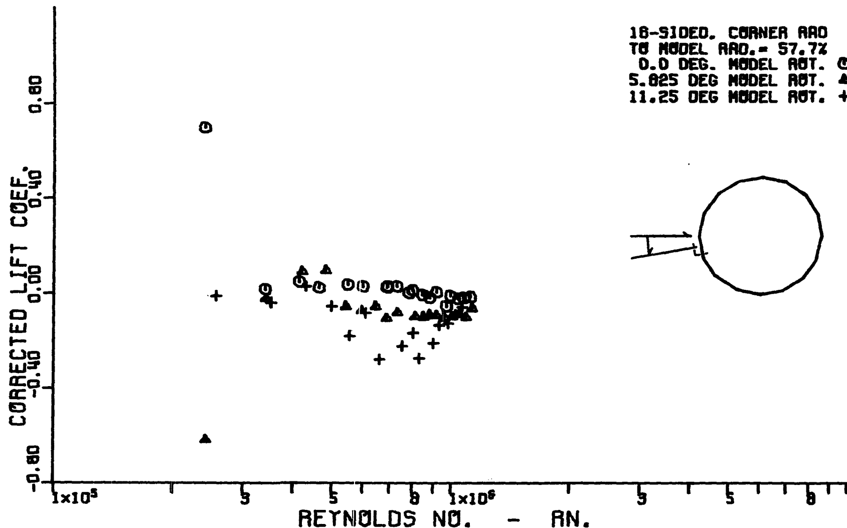
Figure 101. Variation of corrected cross-flow lift coefficient with corrected cross-flow Reynolds number for a hexadecagonal cylinder having a corner radius equal to 57.7 percent of the radius of the inscribed circular cylinder.
