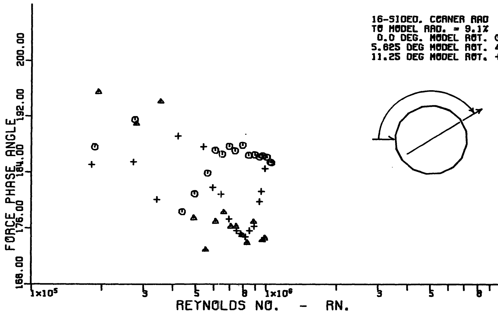
Figure 135. Variation of corrected cross-flow force phase angle with corrected cross-flow Reynolds number for a hexadecagonal cylinder having a corner radius equal to 9.1 percent of the radius of the inscribed circular cylinder.
