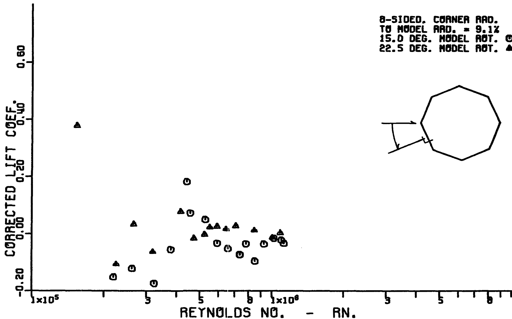
Figure 71. Variation of corrected cross-flow lift coefficient with corrected cross-flow Reynolds number for an octagonal cylinder having a corner radius equal to 9.1 percent of the radius of the inscribed circular cylinder.
