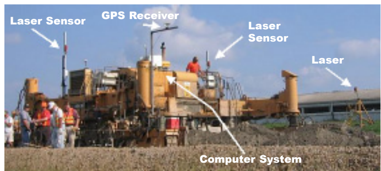
Slip-form paver with GPS equipment attached
