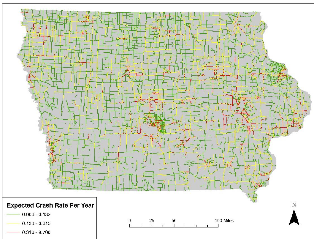
Figure 15. Expected centerline- and edgeline-related crashes per mile per year
