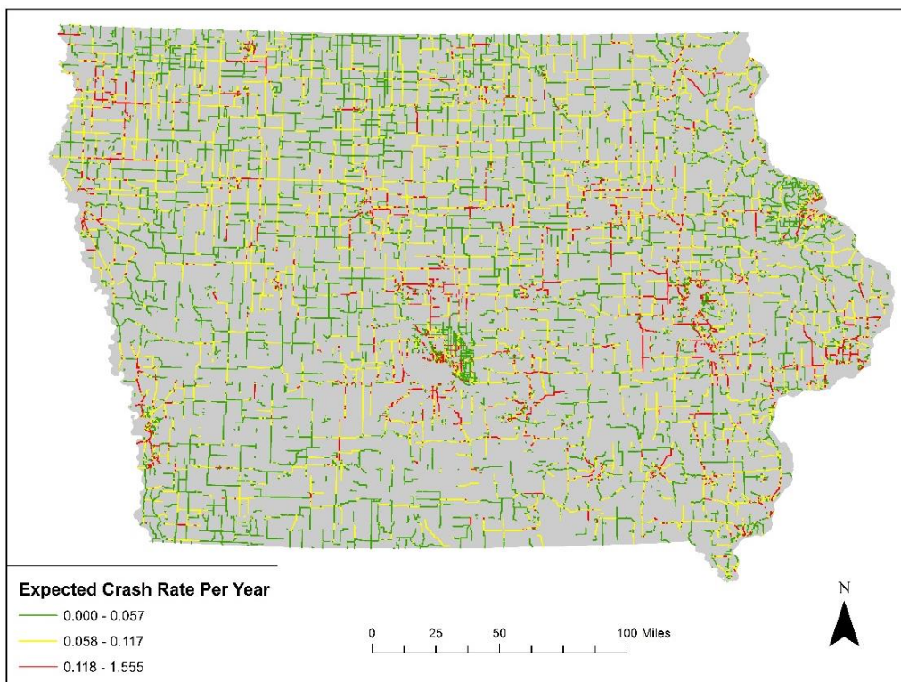
Figure 17. Expected edgeline-related crashes per mile per year
