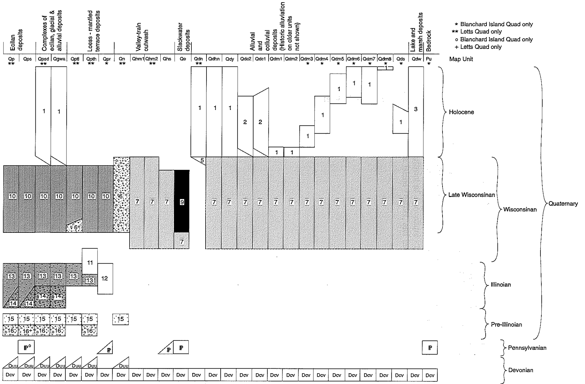
Figure 1. Correlation of Map and Cross-Section Units: Letts, Iowa and Blanchard Island, Illinois-Iowa 7.5' Quadrangles.
