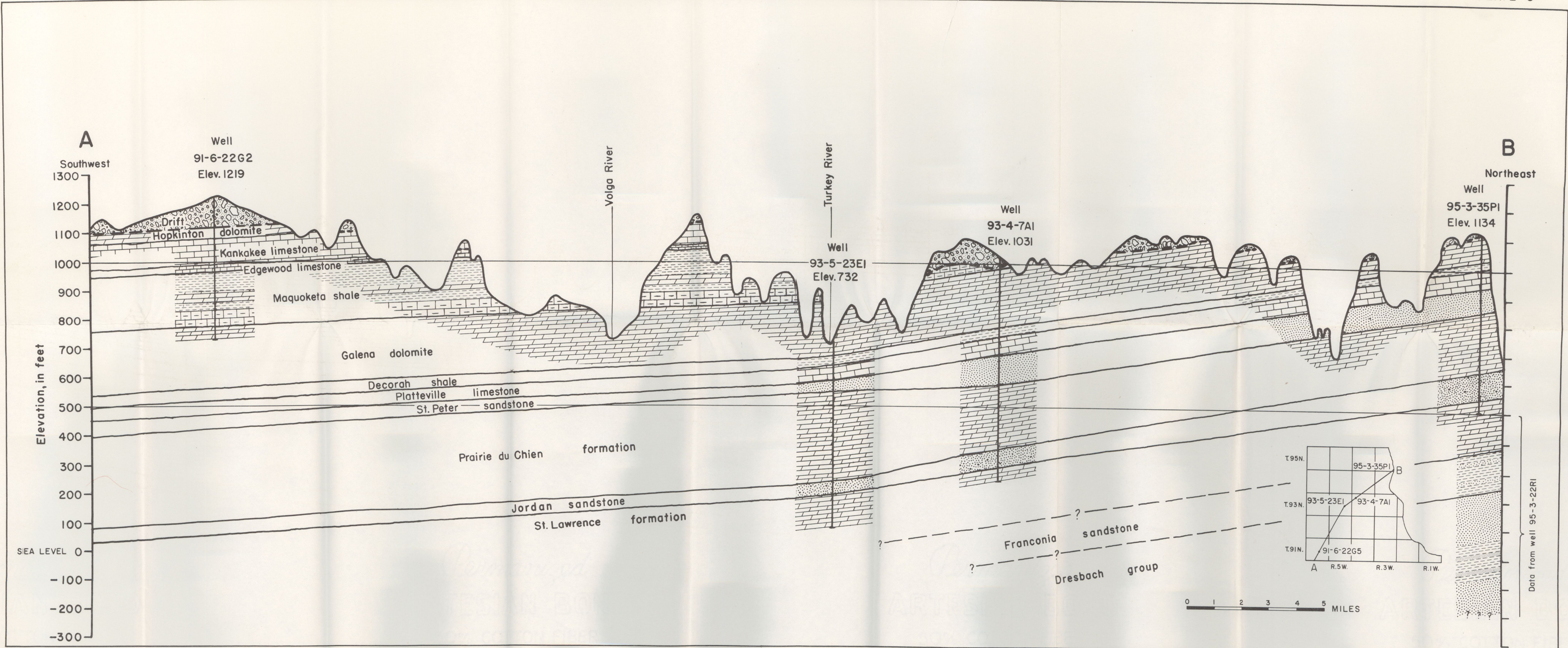
GEOLOGIC SECTION FROM STRAWBERRY POINT TO MCGREGOR, CLAYTON COUNTY, IOWA
