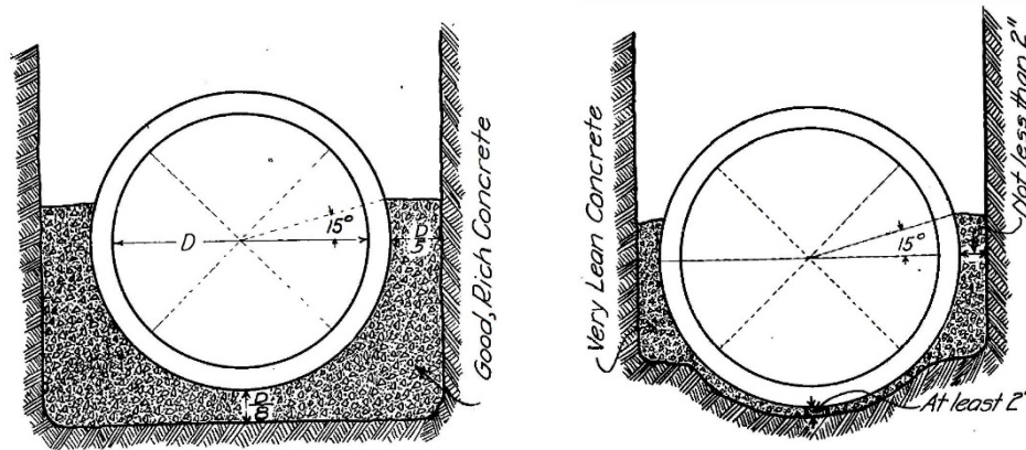
Figure 3. Method of Strengthening Drain Tile and Sewer Pipe to Carry Heavy Loads (Reproduced from Ref. 1)
