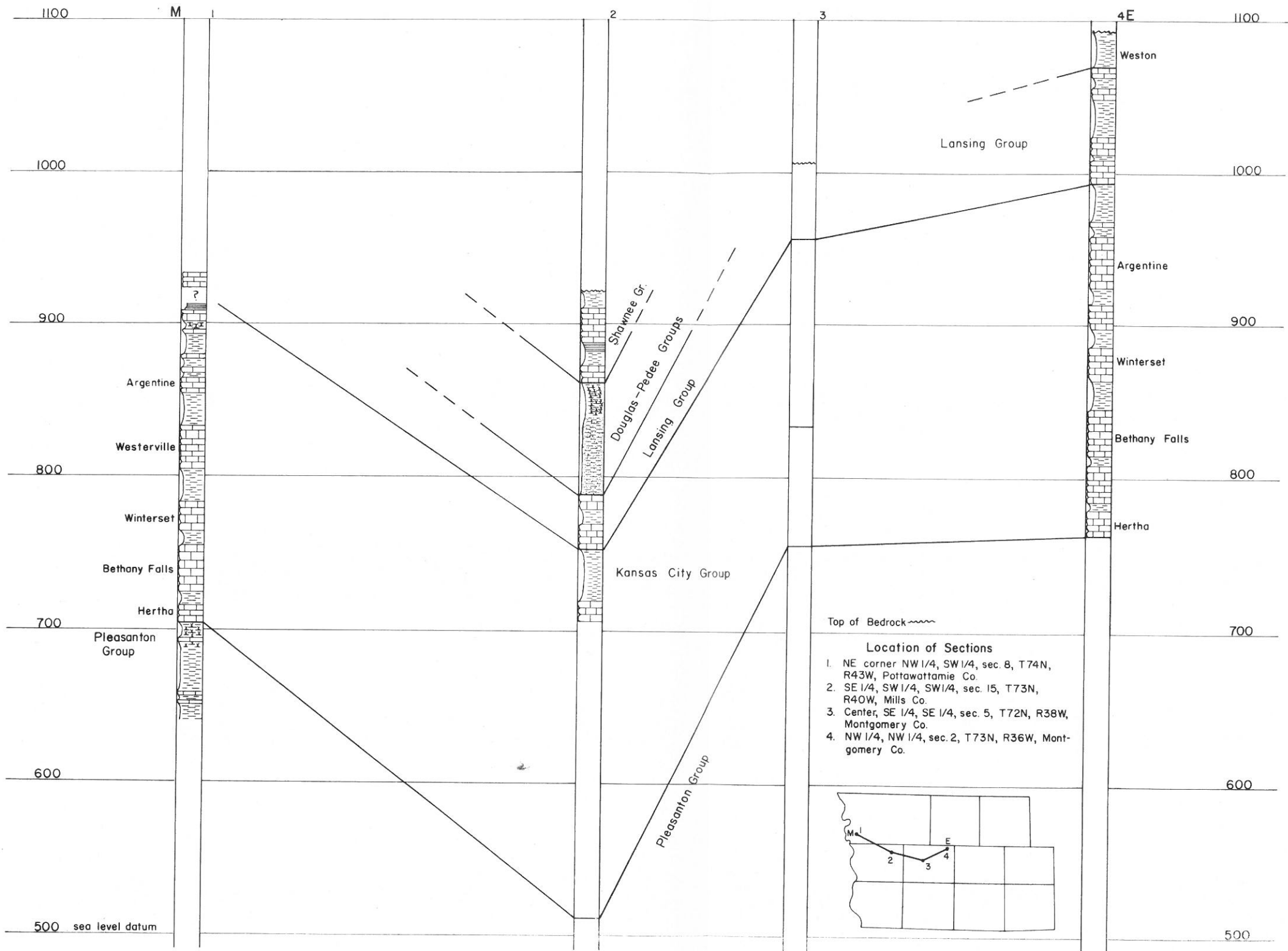
Figure 13. Cross section M-E, Council Bluffs to Grant.
