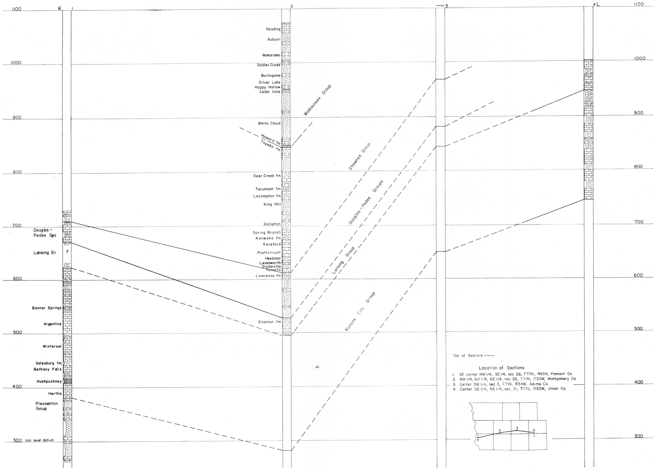
Figure 14. Cross section K-L, Thurman to Creston.
