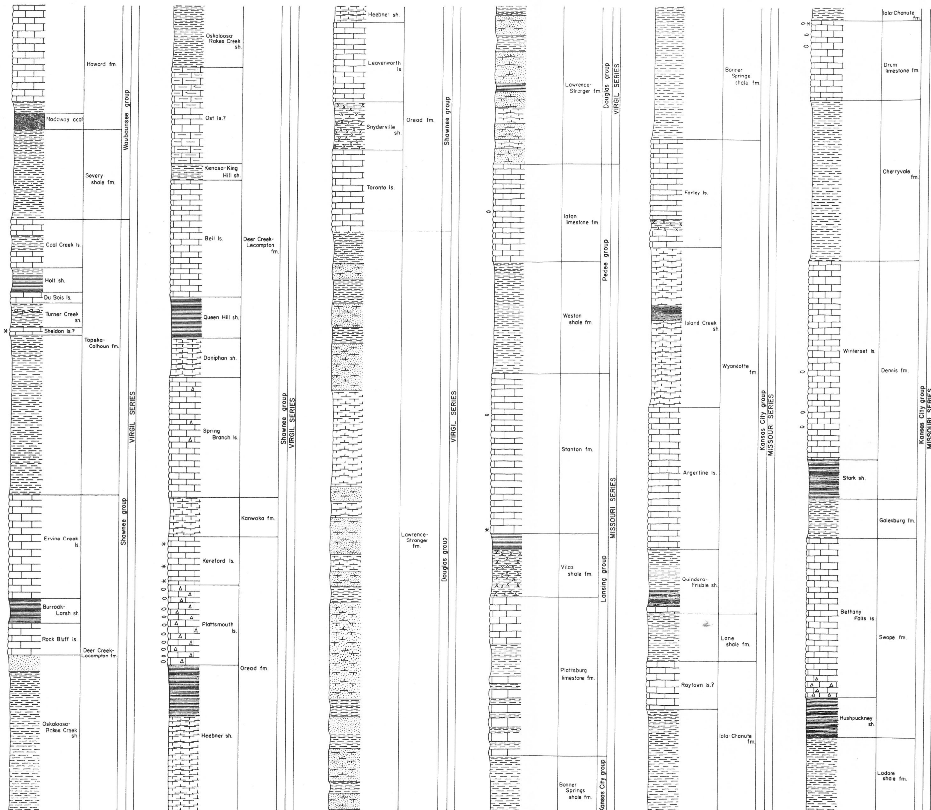
FIGURE 27. GRAPHIC COLUMN OF THE ROCKS OF THE PENNSYLVANIAN SYSTEM TAYLOR COUNTY, IOWA
