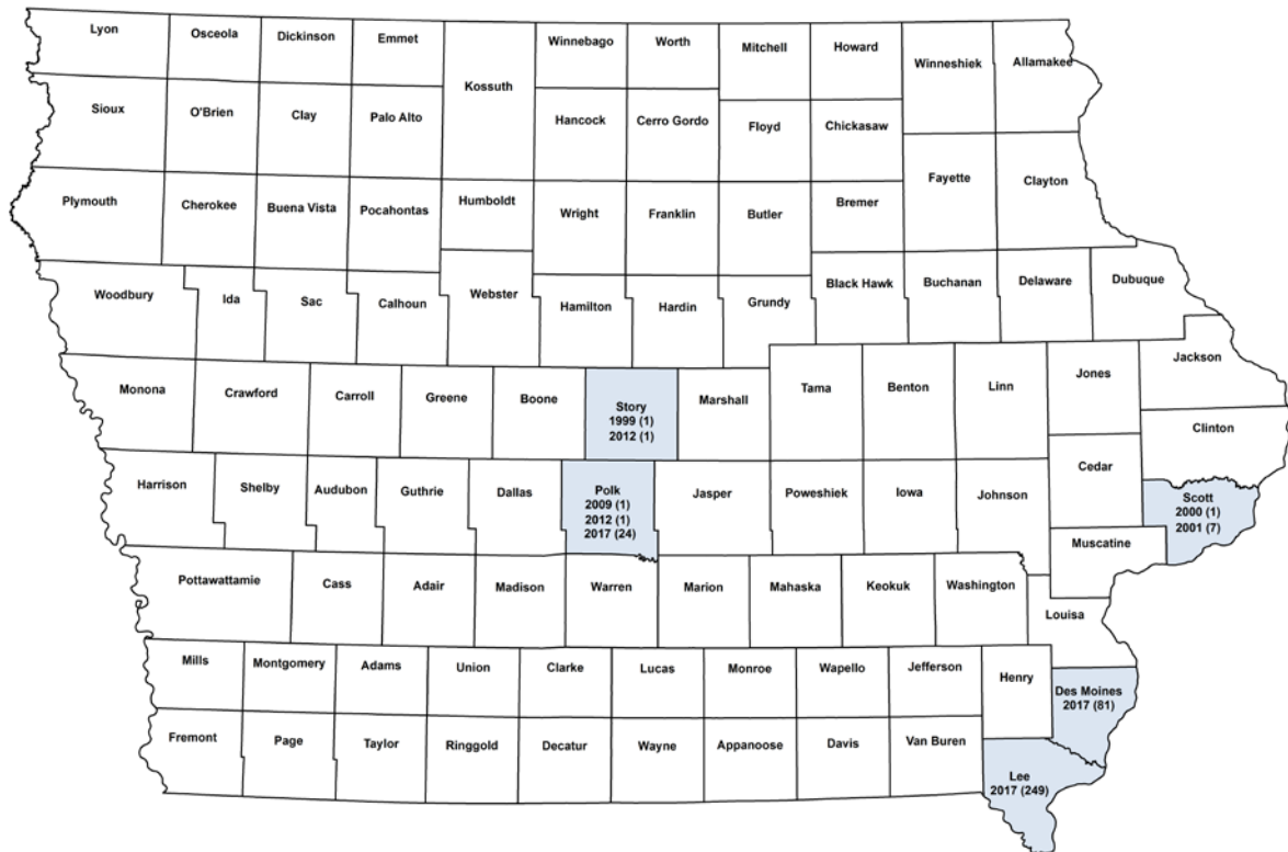
Figure 7. Aedes albopictus identified in Iowa
