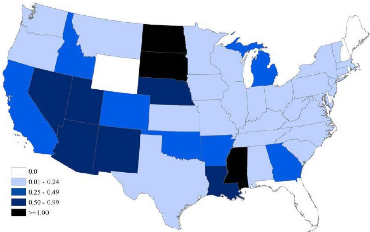
Figure 3. WNV neuroinvasive disease incidence* reported to ArboNET, by state–United States, 2017 (as of September 26, 2017)
