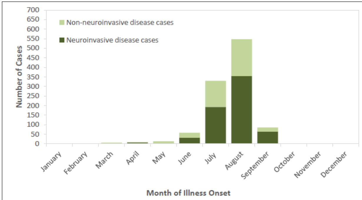
Figure 4. WNV disease cases reported to ArboNET, by month of onset – United States, 2017 (as of September 26, 2017)
