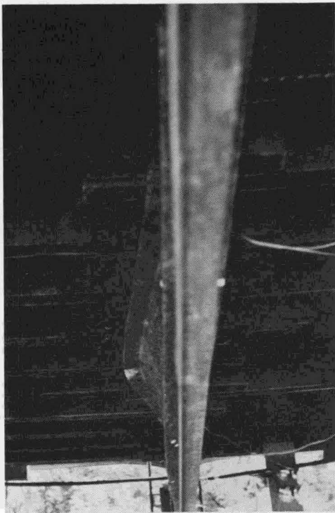
Fig. 48. Photograph of buckling of compression flange of floorbeam 5.
