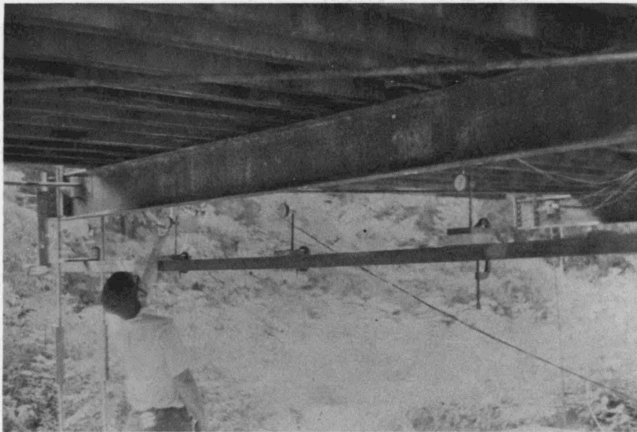
Fig. 44. Photograph of deflection dial placement for floorbeam test.
