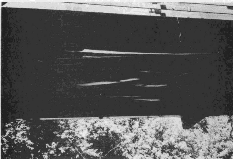
Fig. 19. Photograph of failed stringers from deck test 1.
