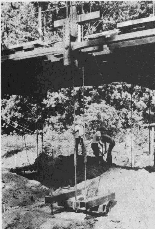
Fig. 26. Photograph showing system used to attach steel rods to concrete mats.
