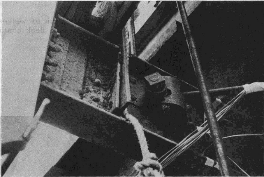
Fig. 52. Photograph showing where last four bolts broke.
