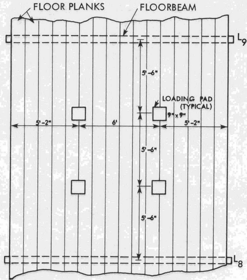
Fig. 8. Load location for deck test 1 (plan view).
