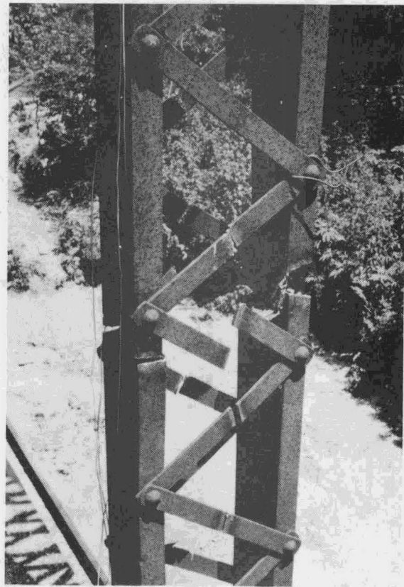
Fig. 41. Photograph of damaged member after collapsing upon itself.
