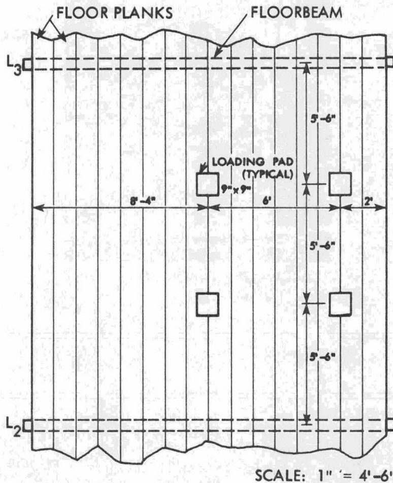
Fig. 10. Load location for deck test 2 (plan view).
