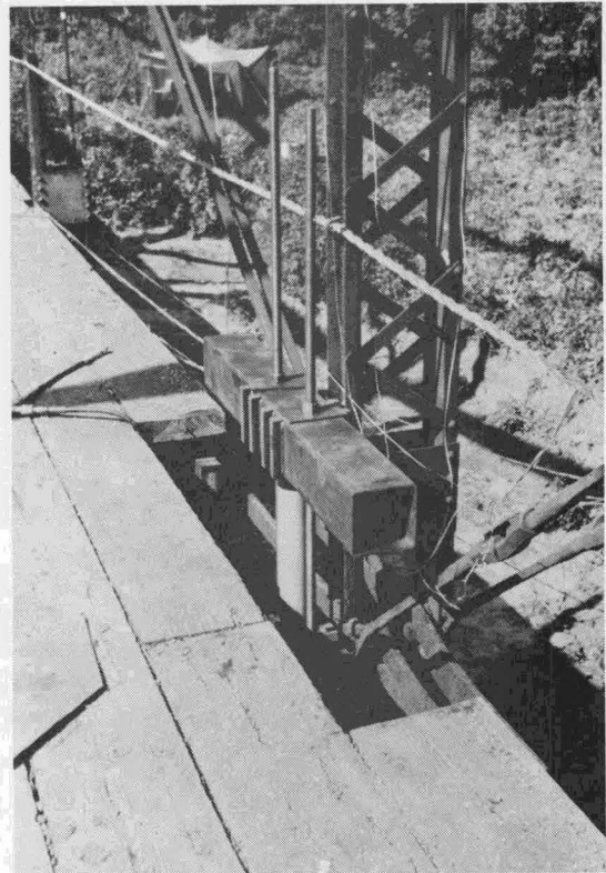
Fig. 27. Photograph showing hydraulic jack and structural tube arrangement.
