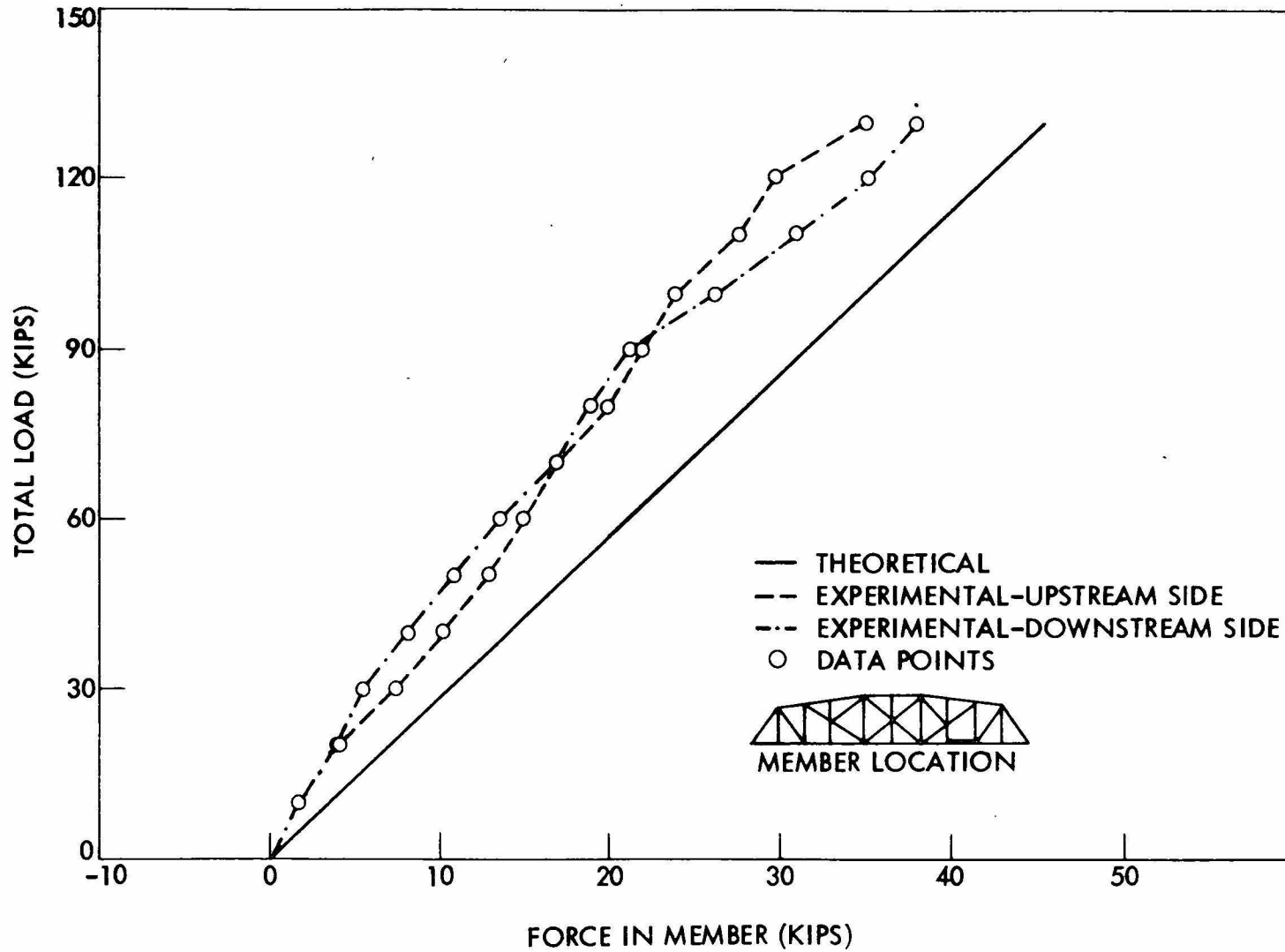
Fig. 67. Total load-force in member L_7L_8 .
