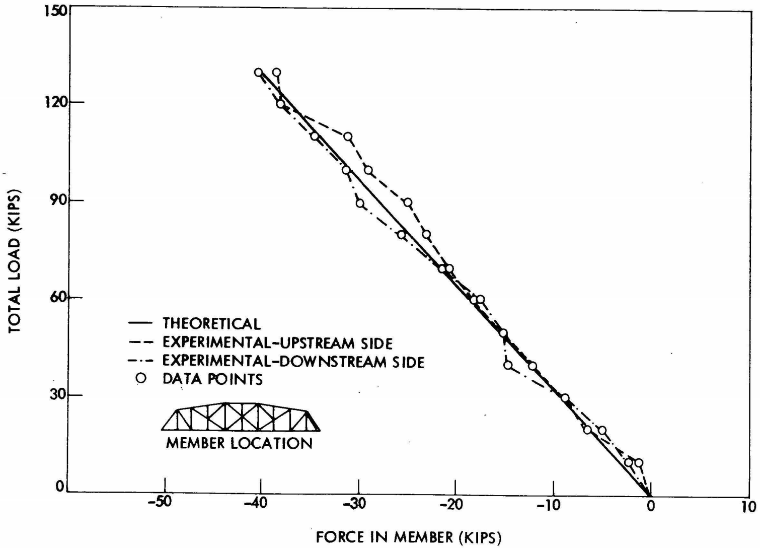
Fig. 69. Total load-force in member L_{10}U_9 (upper gages).
