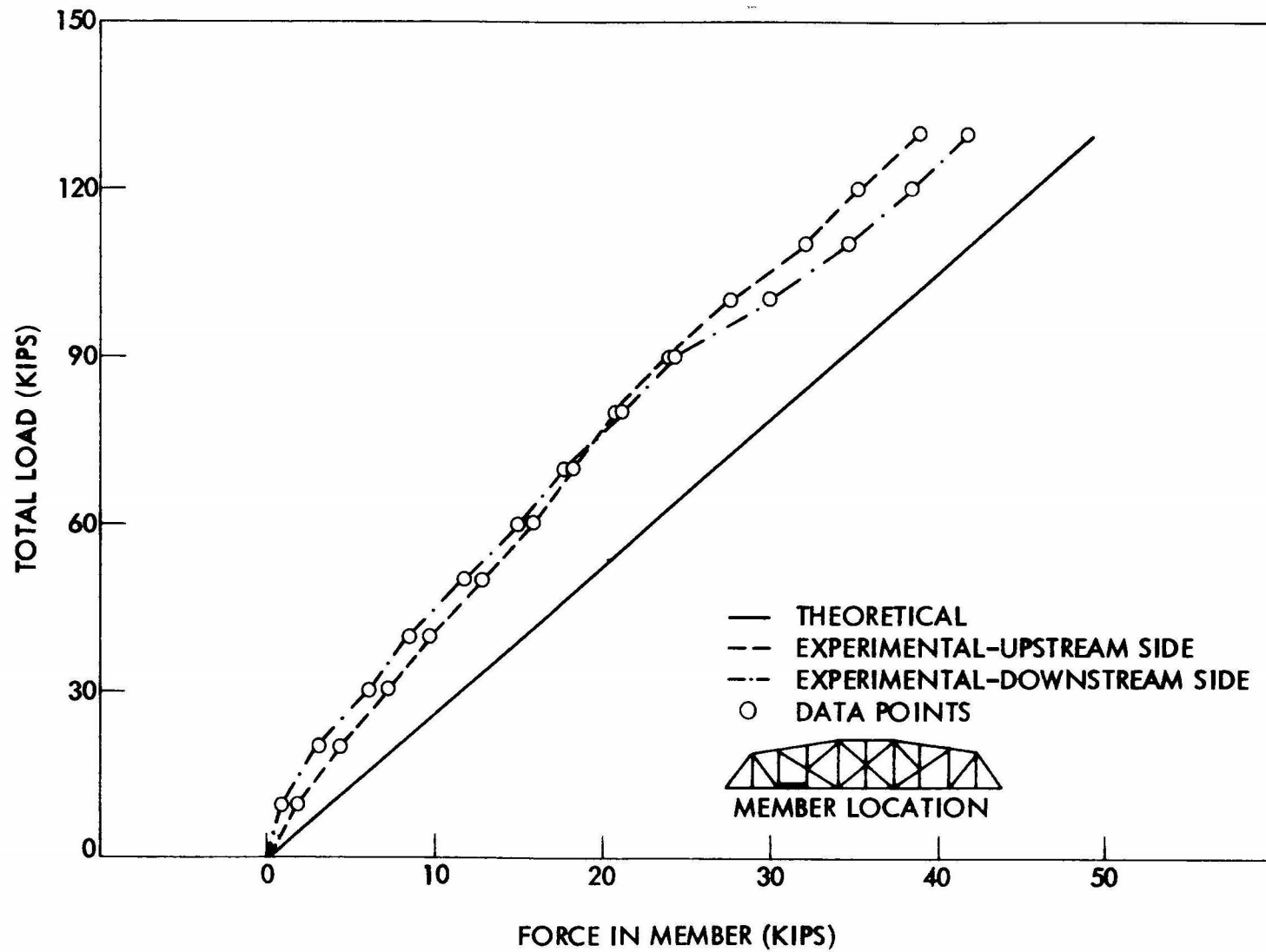
Fig. 64. Total load-force in member L_2L_3 .
