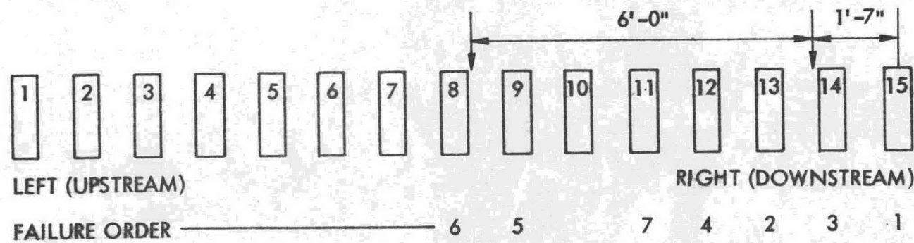
Fig. 13. Numbering system and failure order of stringers for deck tests 1 and 2.
