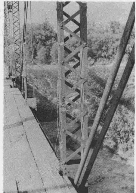
Fig. 39. Photograph of damaged member with only web of outside channel remaining.
