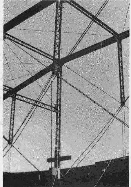
Fig. 37. Photograph of distortion of lower chord at L_5 .
