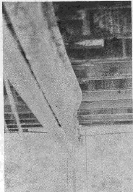
Fig. 51. Photograph of lateral buckling of floorbeam 4.
