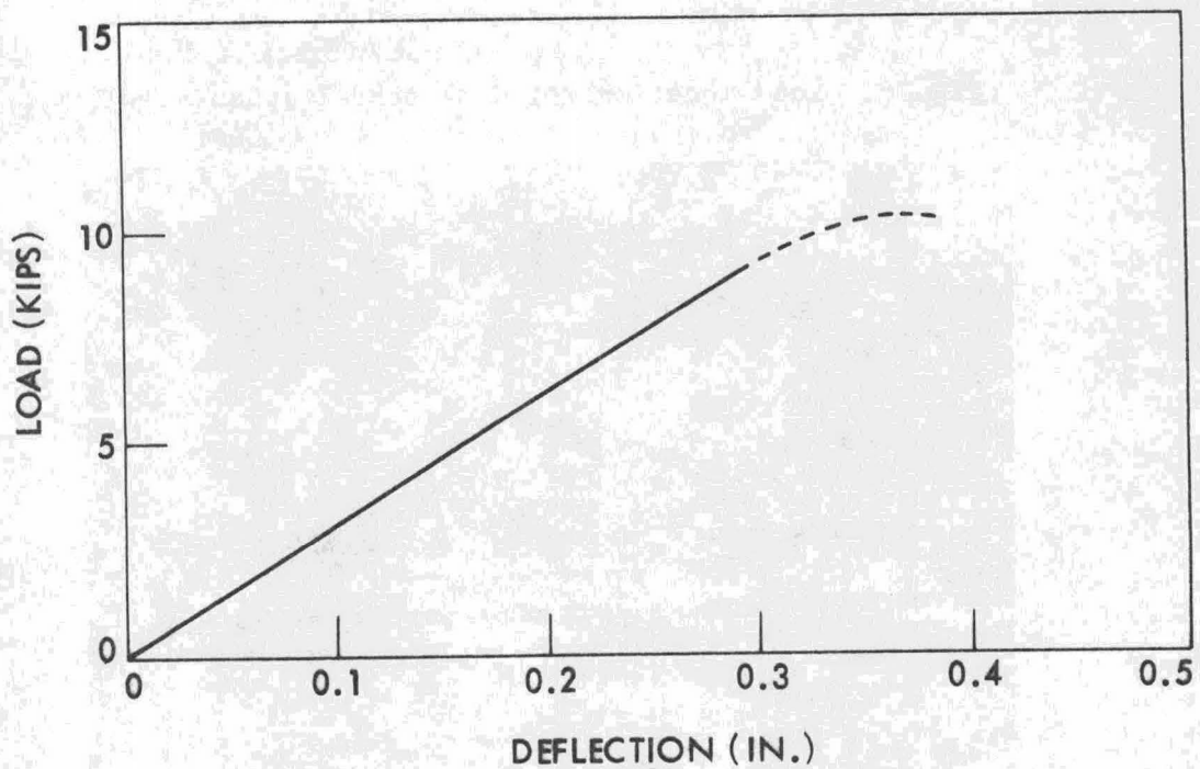
Fig. 7. Typical load-deflection curve for timber flexure test.
