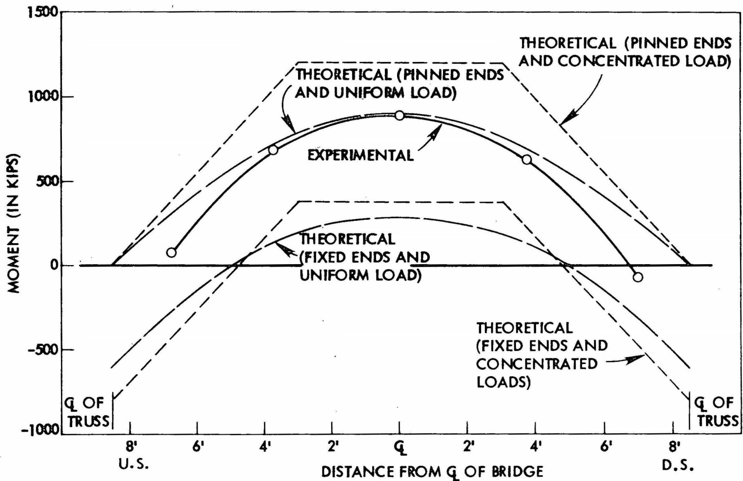
Fig. 75. Moment cross section for floorbeam test at L_4 for a load of 35 kips.
