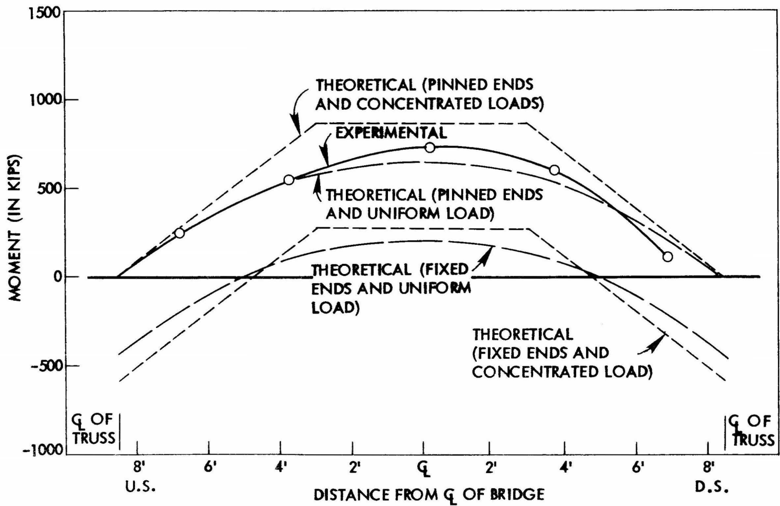
Fig. 76. Moment cross section for floorbeam test at L_5 for a load of 25 kips.
