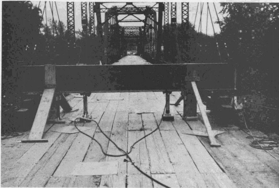
Fig. 42. Photograph of floorbeam test setup.
