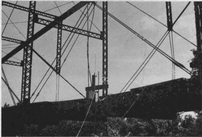
Fig. 36. Photograph of hangers buckling at L_5 .
