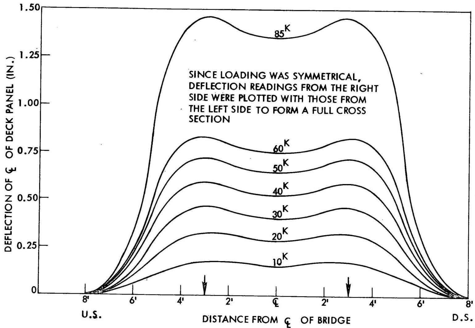
Fig. 55. Deflection cross section at mid-span of deck panel for deck test 1 at various loads.
