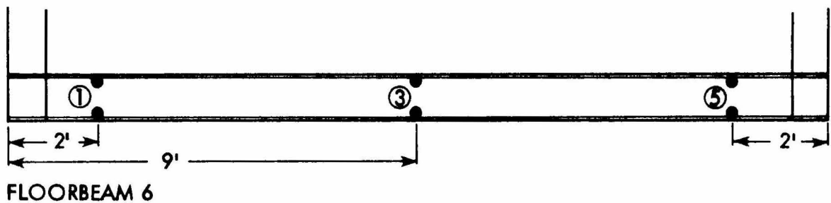
Fig. 47. Location of strain gages on floorbeams.
