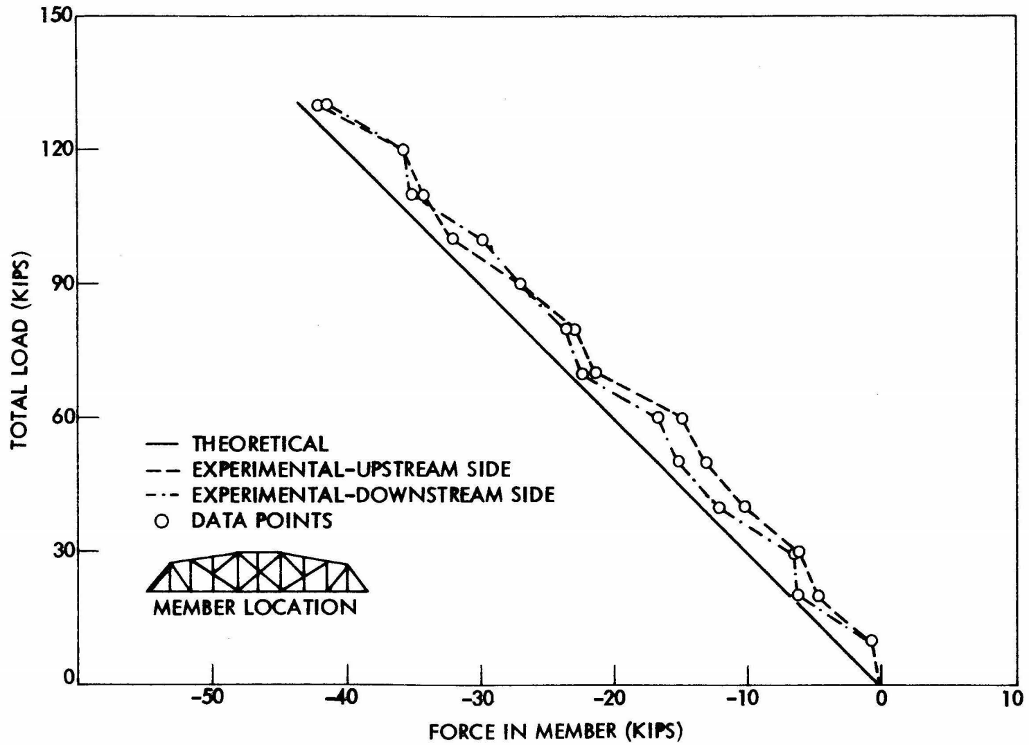
Fig. 60. Total load-force in member I_0U_1 (upper gages).
