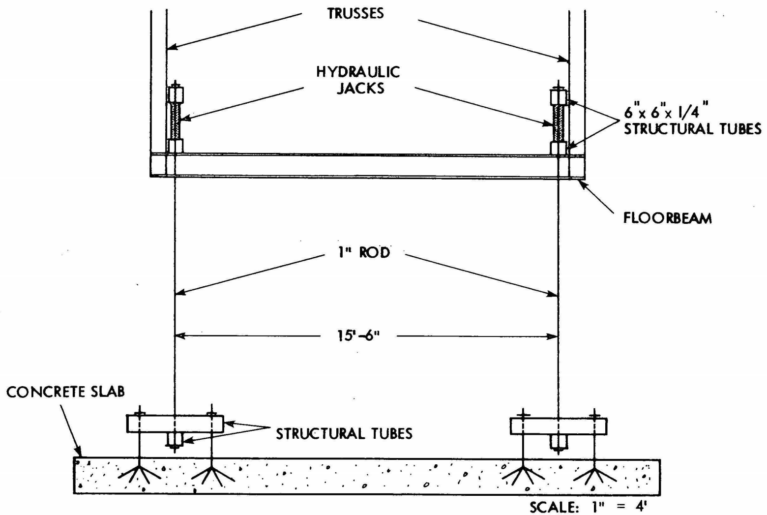
Fig. 30. Loading system details (end view).
