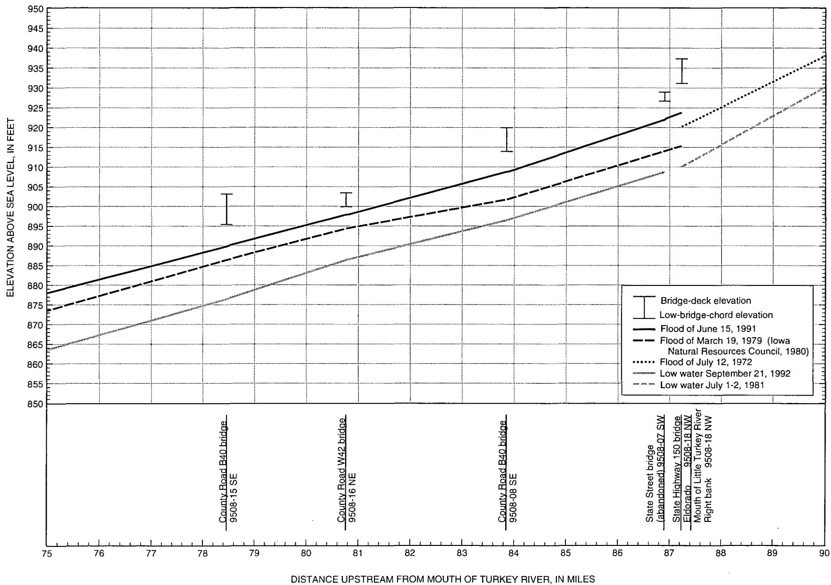
Figure 3F. Water-surface-elevation profiles for the Turkey River, river miles 75-90.
