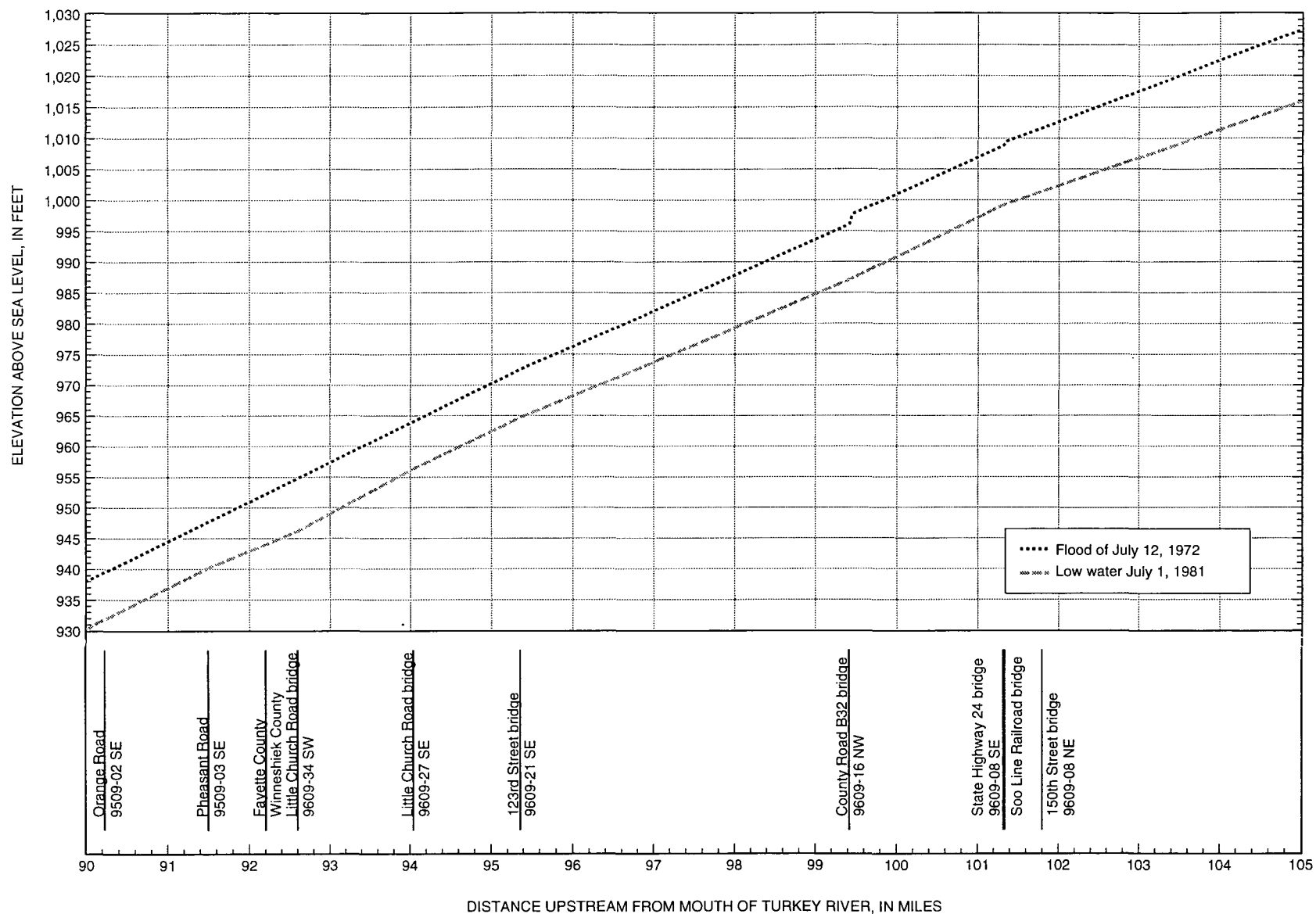
Figure 3G. Water-surface-elevation profiles for the Turkey River, river miles 90-105.
