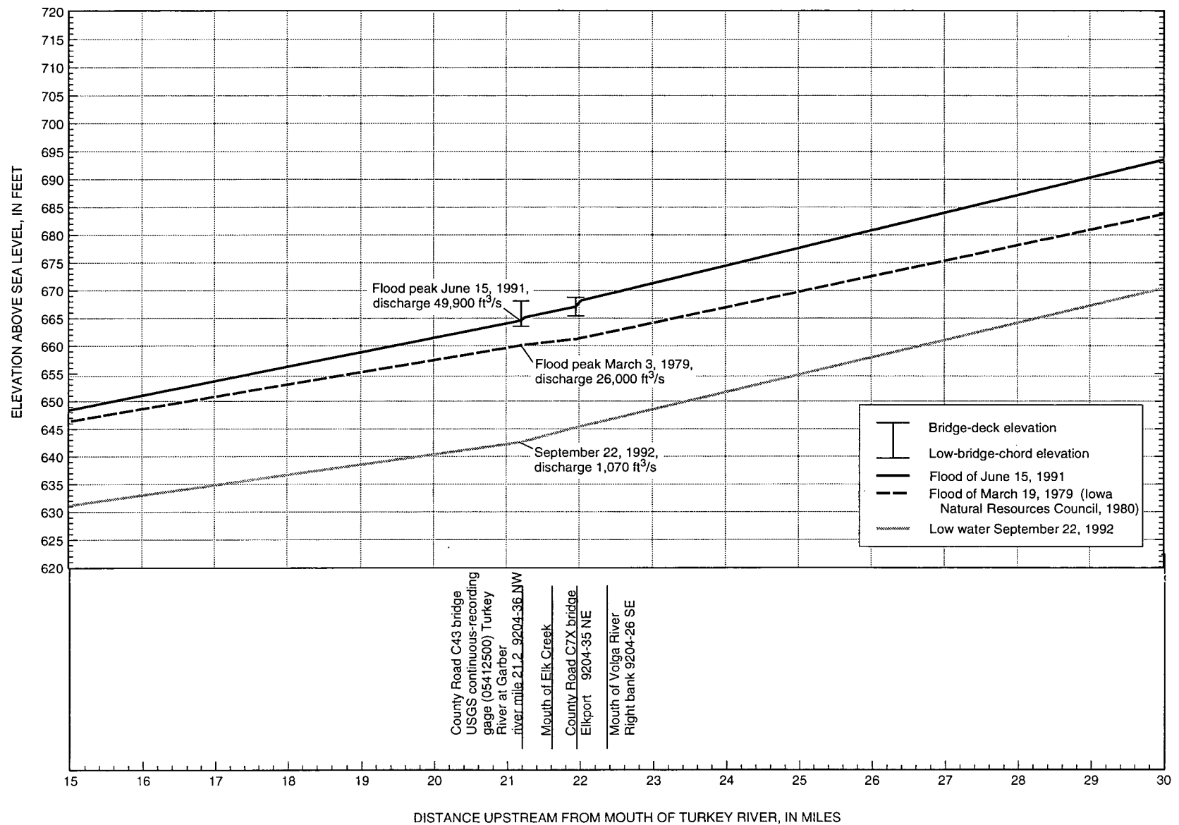
Figure 3B. Water-surface-elevation profiles for the Turkey River, river miles 15-30.
