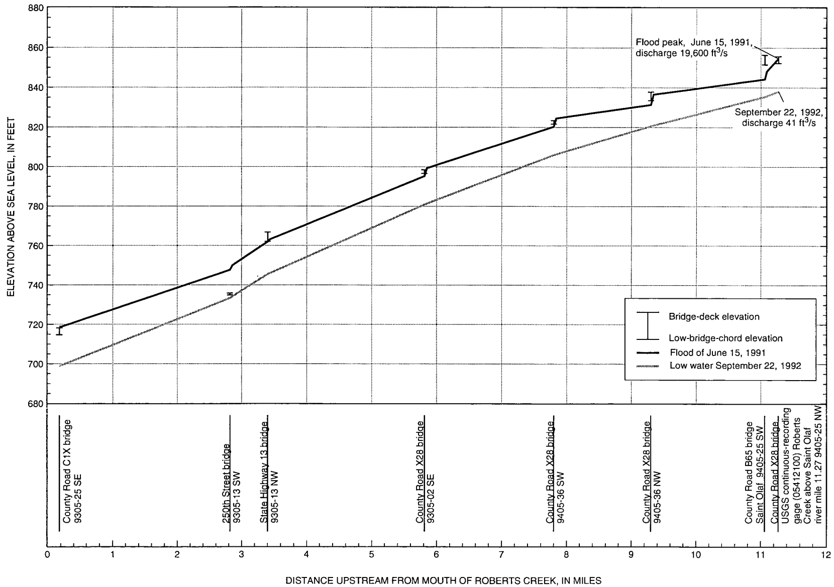
Figure 6. Water-surface-elevation profiles for Roberts Creek, river miles 0.18-11.27.
