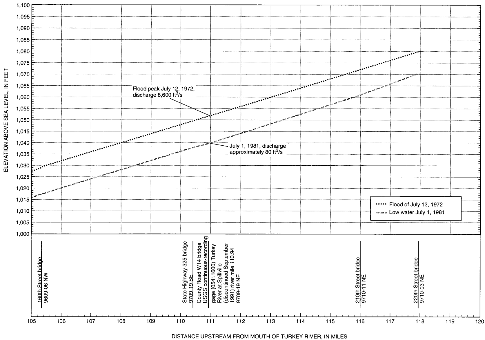
Figure 3H. Water-surface-elevation profiles for the Turkey River, river miles 105-117.94.
