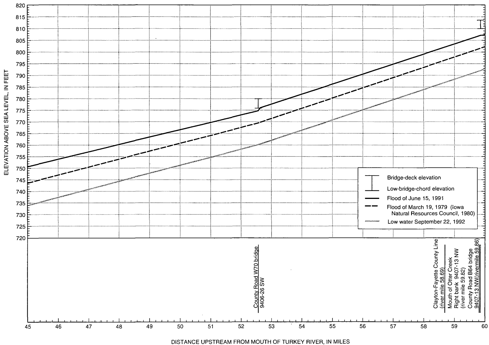
Figure 3D. Water-surface-elevation profiles for the Turkey River, river miles 45-60.
