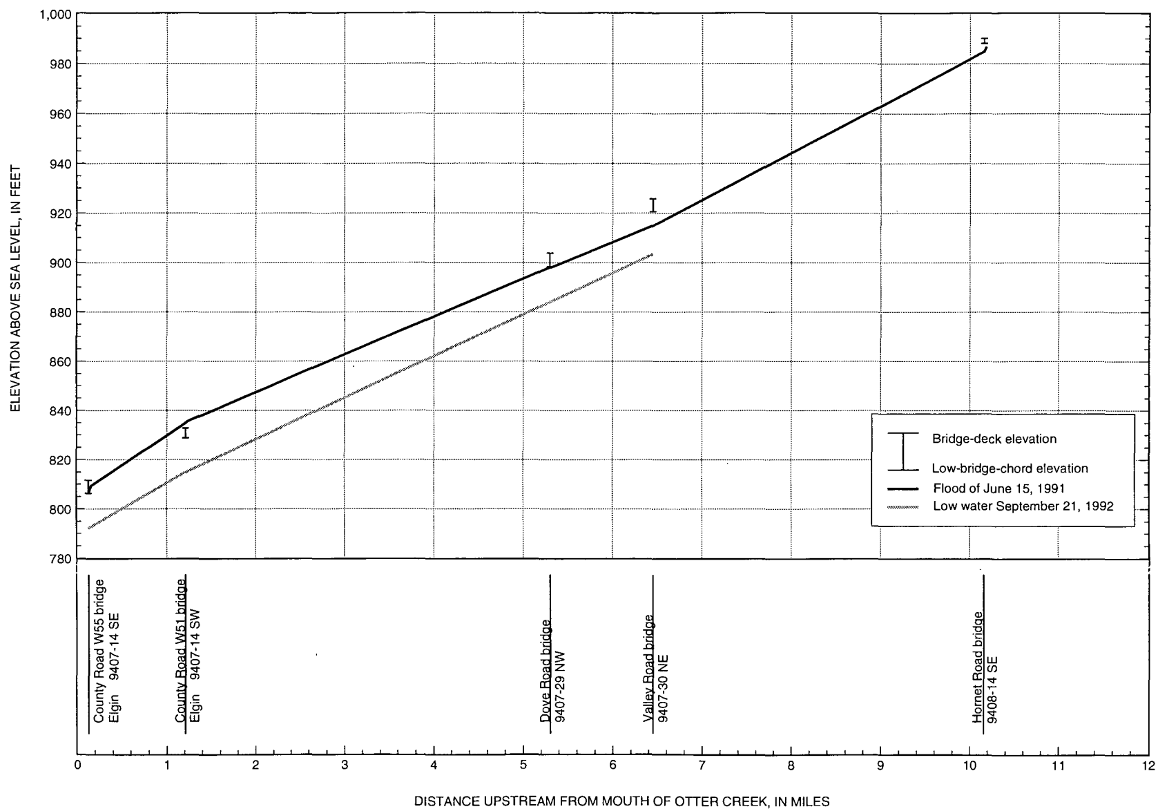
Figure 7. Water-surface-elevation profiles for Otter Creek, river miles 0.13-10.16.
