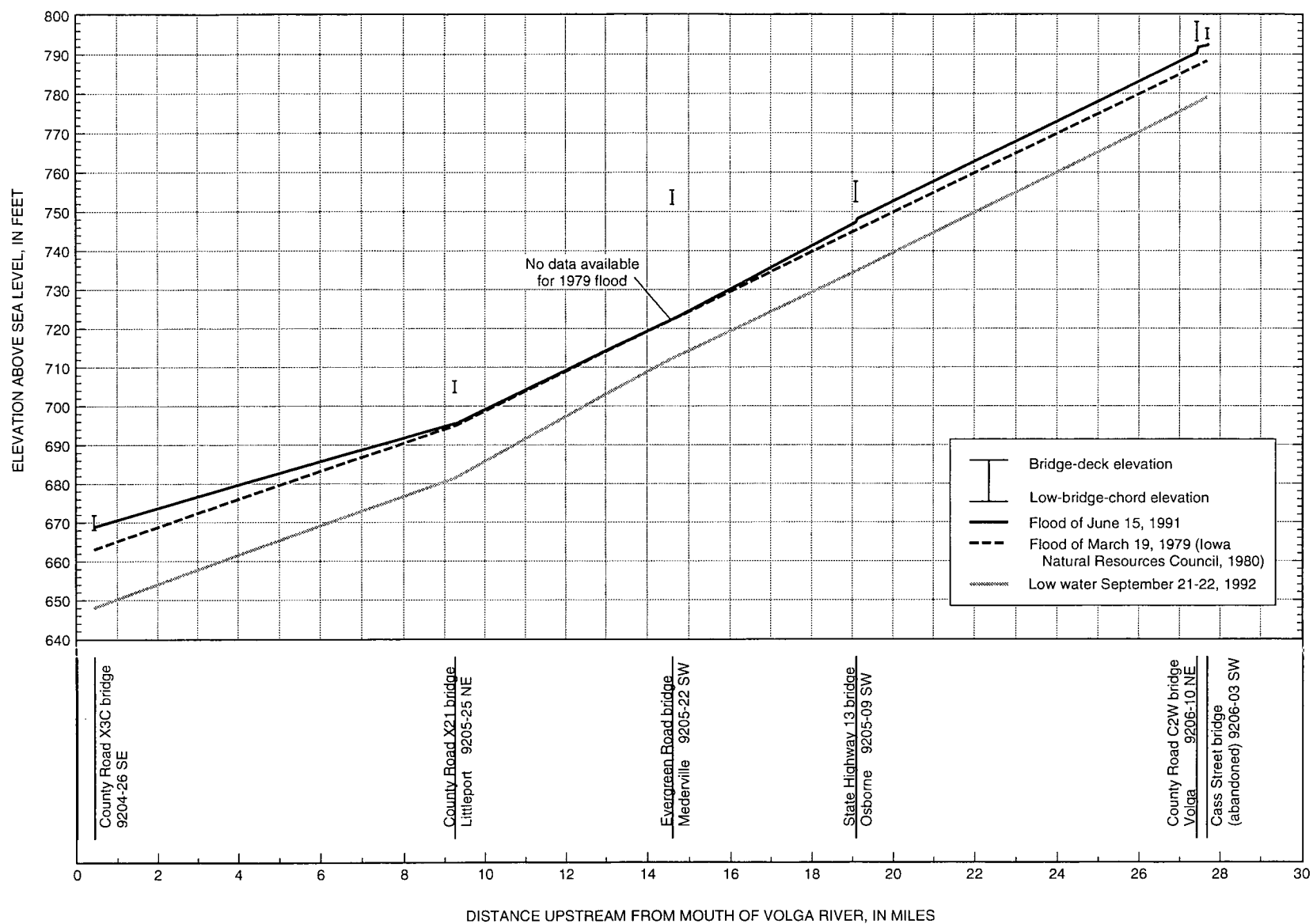
Figure 4. Water-surface-elevation profiles for the Volga River, river miles 0.42-27.68.
