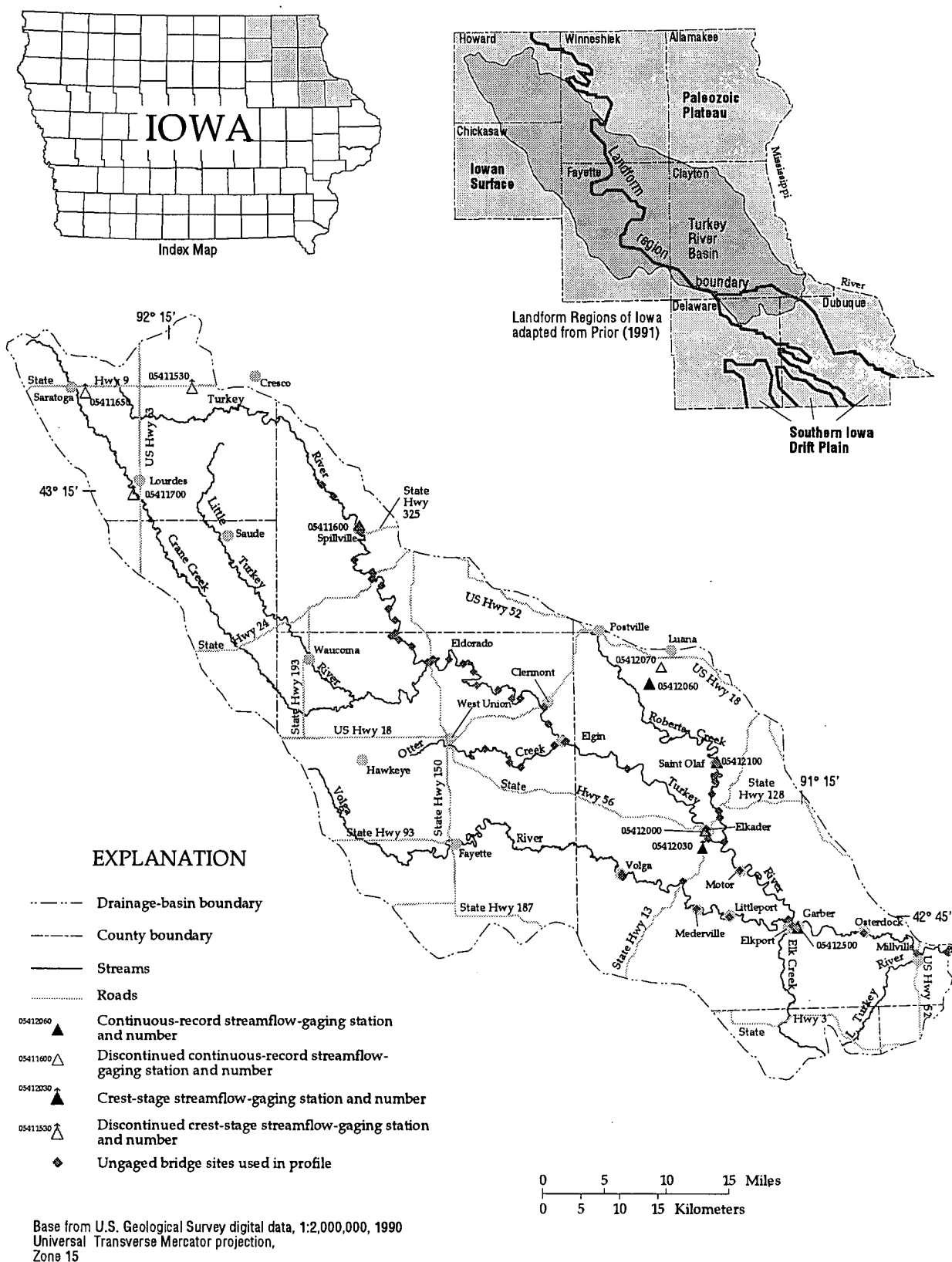
Figure 1. Turkey River Basin showing location of bridge sites used in July 12, 1972, March 19, 1979, and June 15, 1991, flood profiles and U.S. Geological Survey streamflow-gaging stations.
