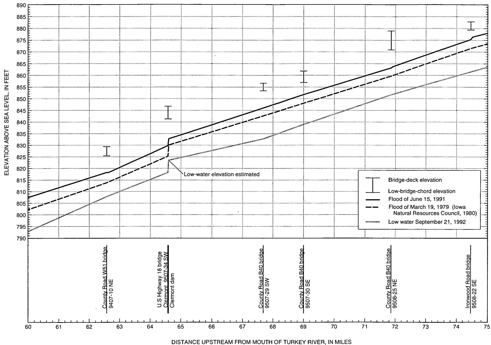
Figure 3E. Water-surface-elevation profiles for the Turkey River, river miles 60-75.
