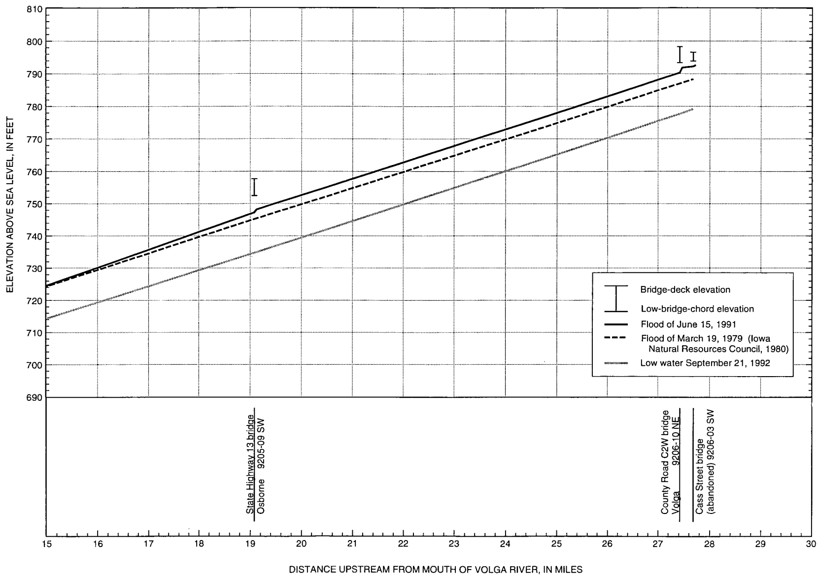
Figure 5B. Water-surface-elevation profiles for the Volga River, river miles 15-27.68.
