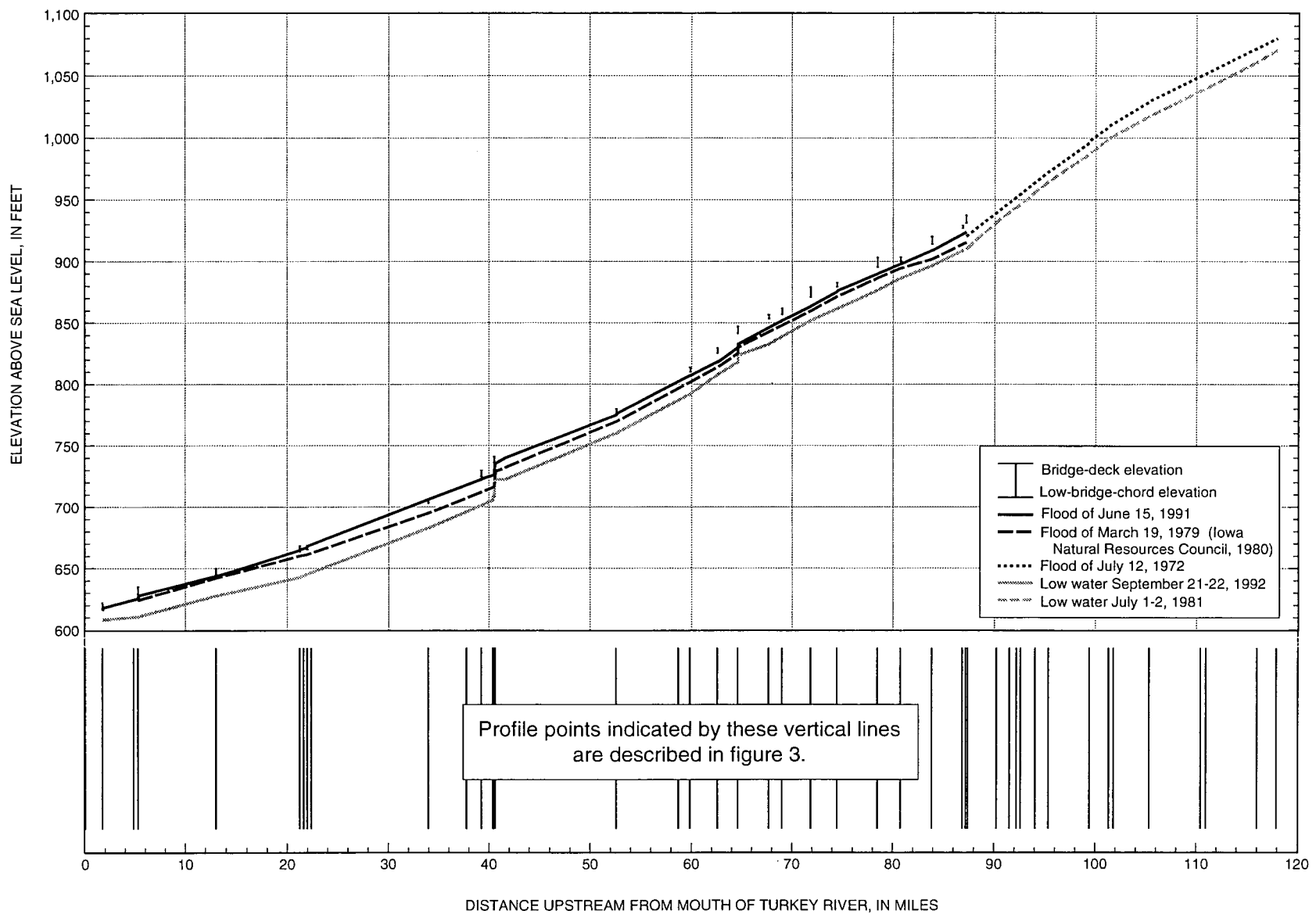
Figure 2. Water-surface-elevation profiles for the Turkey River, river miles 1.71-117.94.
