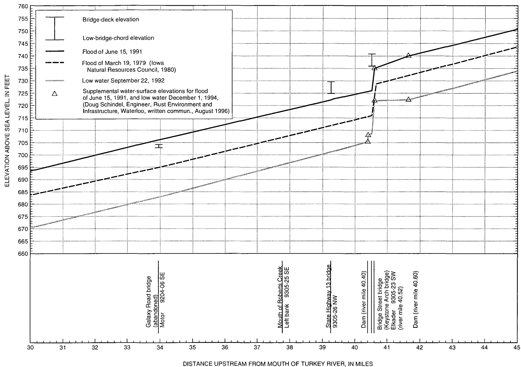
Figure 3C. Water-surface-elevation profiles for the Turkey River, river miles 30-45.
