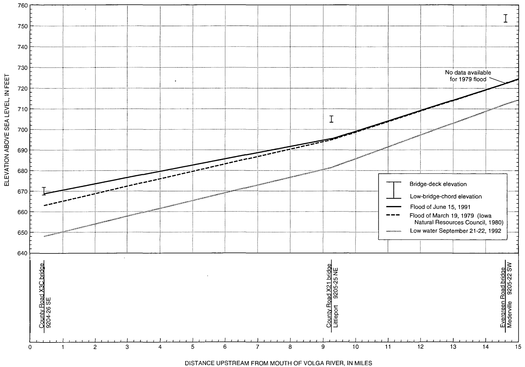
Figure 5A. Water-surface-elevation profiles for the Volga River, river miles 0.42-15.
