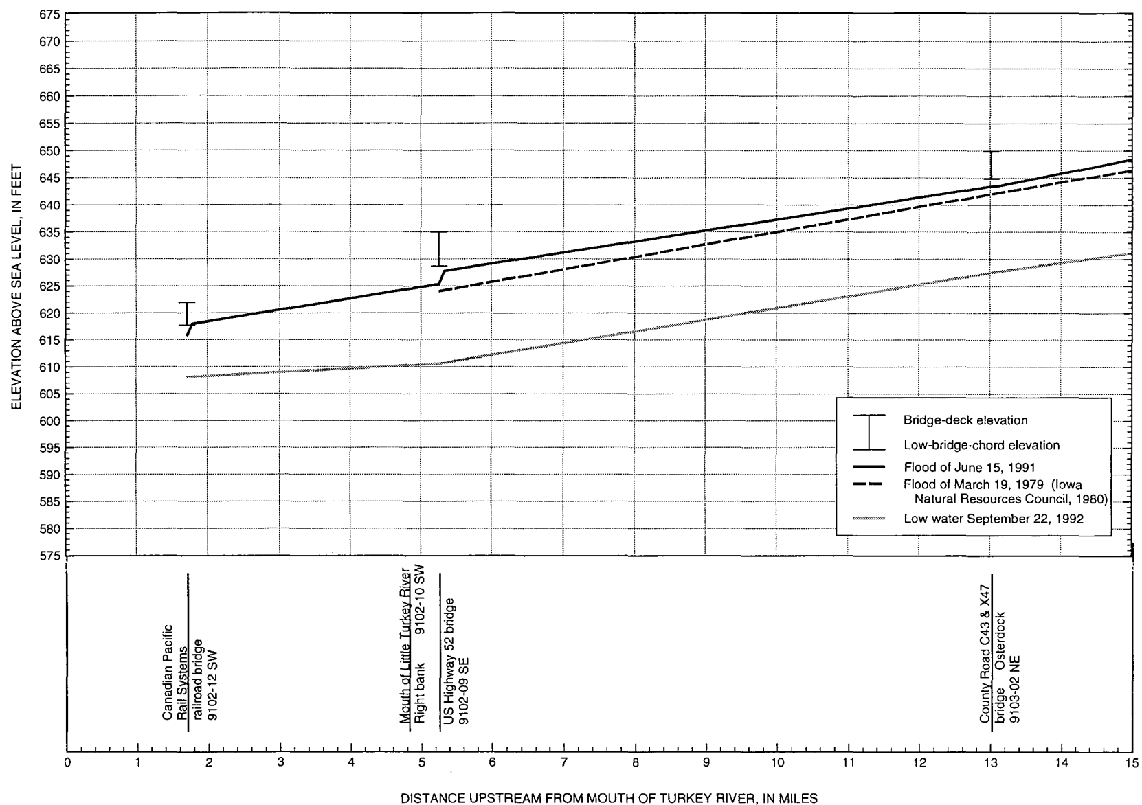
Figure 3A. Water-surface-elevation profiles for the Turkey River, river miles 1.71-15.
