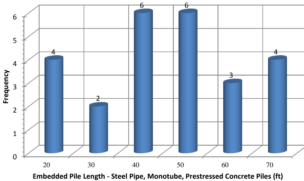
Figure 5.21: Distribution of Embedded Pile Lengths for Historical Steel Pipe, Monotube, and Prestressed Concrete Piles
