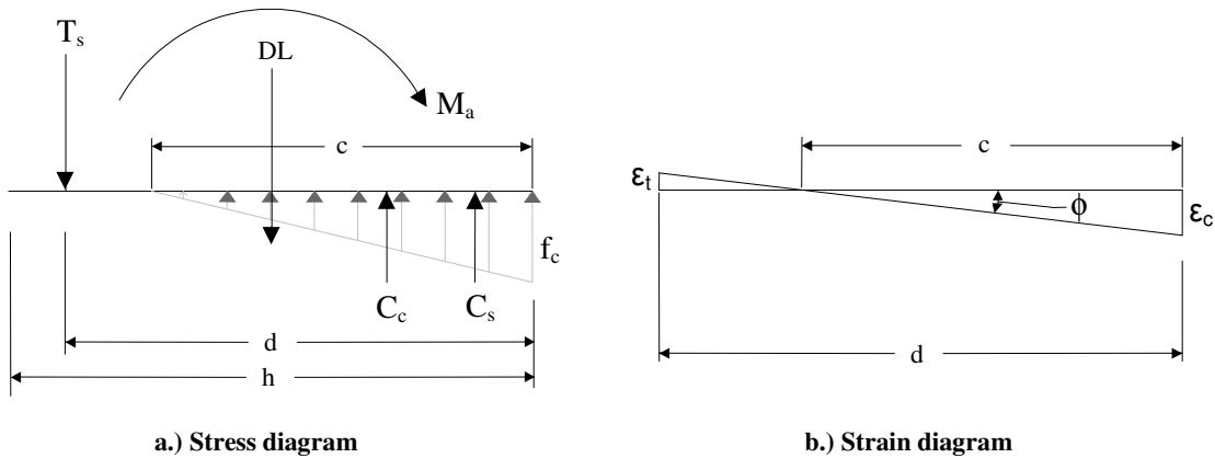
Figure 188. Stress and strain diagrams of R/C column (Column 1) for displacements up to yield moment.
