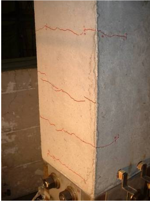
a.) East face of upper segment crack distribution b.) West face of upper segment crack distribution
