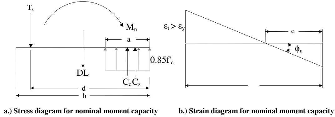
Figure 189. Stress and strain diagrams of reinforced concrete column at nominal moment capacity.
