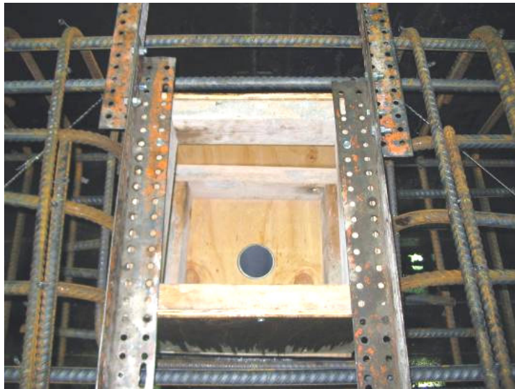
Figure 29. Photograph of boxout in forms.
