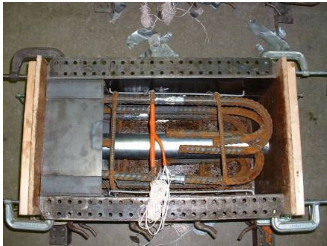
Figure 43. Photograph of Column 3, 2 ft. segment reinforcement in forms.
