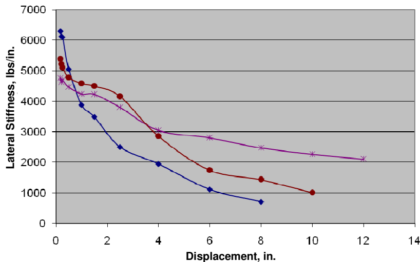
Figure 172. Test “b” lateral stiffness comparisons between Columns 1, 5, and 6.
