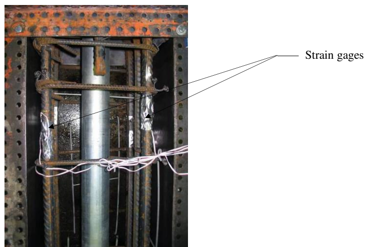
Figure 37. Photograph of Column 2 Strain gages.
