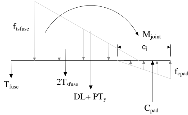
a.) Stress diagram at segment joint
