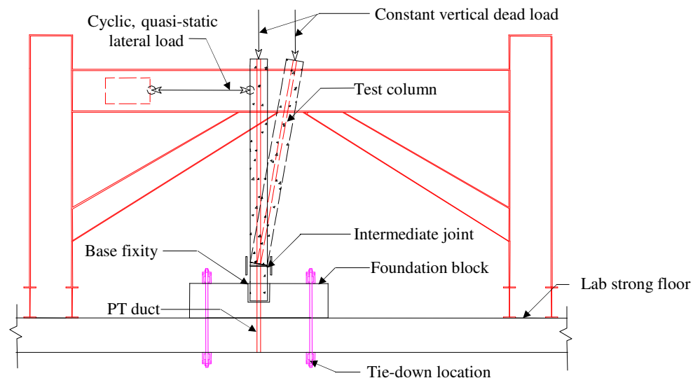
Figure 6. Test schematic.
