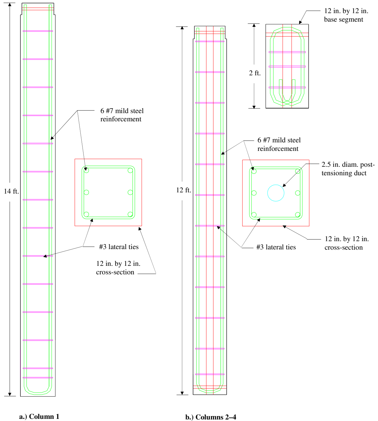
Figure 16. Reinforcement in Columns 1-4.
