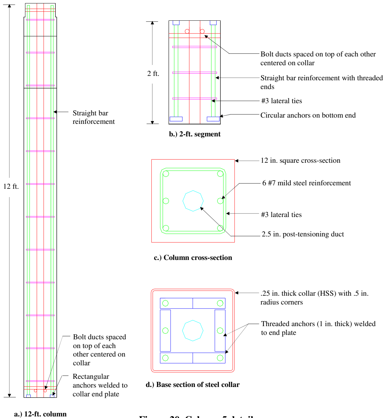
Figure 20. Column 5 details.
