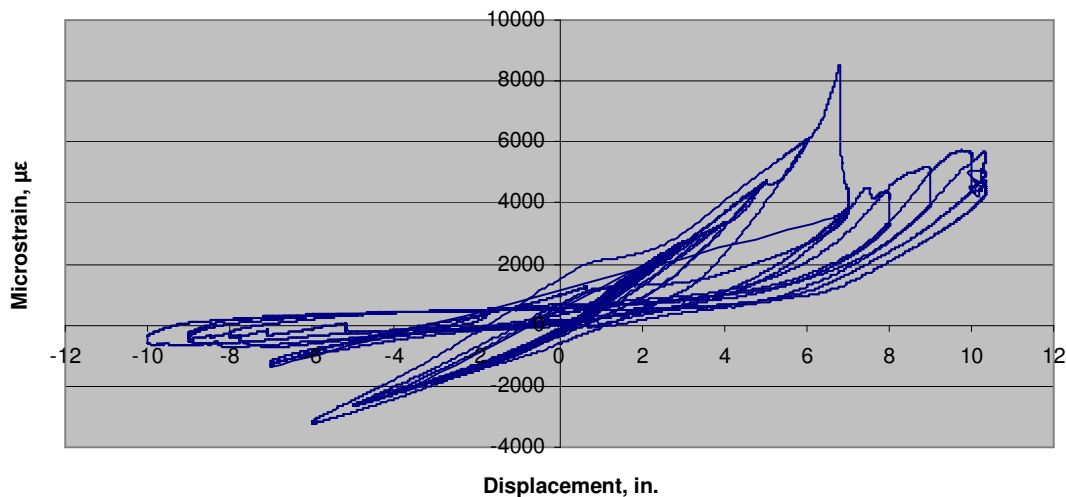
Figure 182. Column 6b lower segment longitudinal reinforcement strain.
