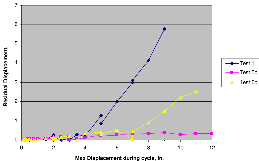
Figure 174. Test “b” residual displacements.
