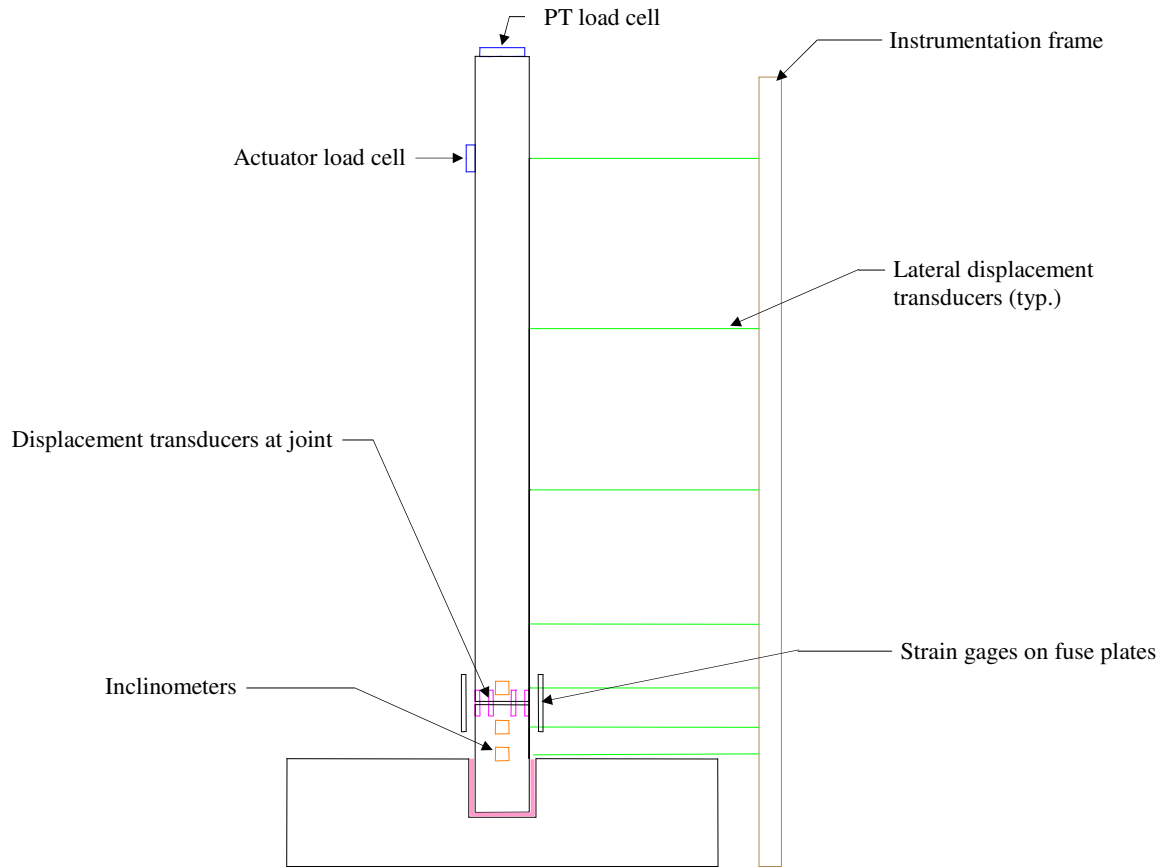
Figure 12. Instrumentation schematic.
