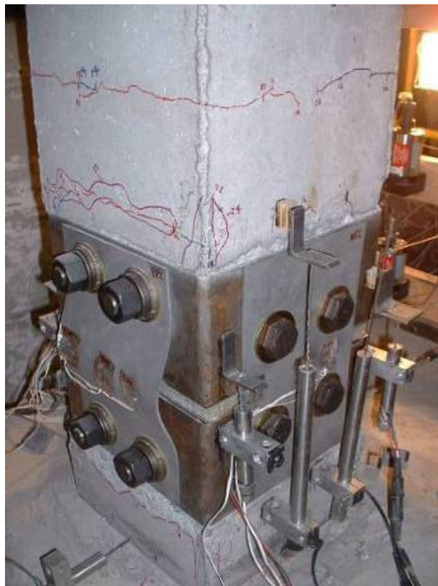
Figure 155. Photograph of Column 6 – Cycle 26b, column damage.
