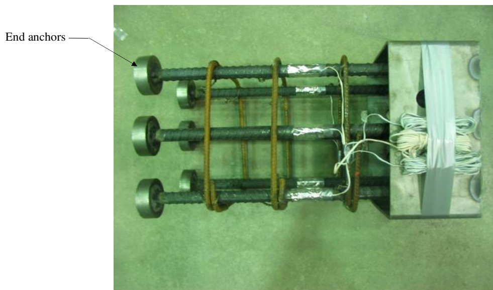
Figure 52. Photograph of Column 5, 2 ft. segment reinforcement.
