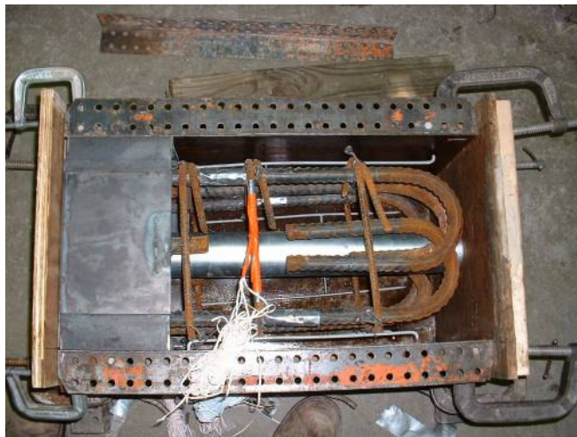
Figure 46. Photograph of Column 4, 2 ft. segment.
