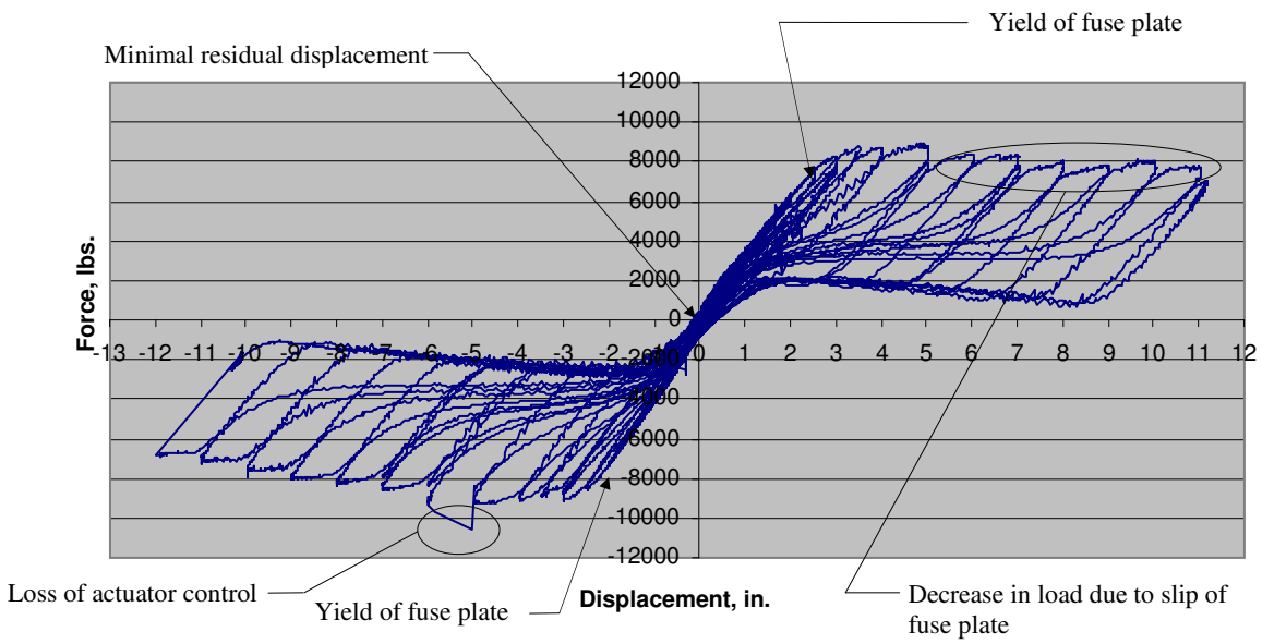
Figure 168. Test 5b load vs. displacement hysteresis.
