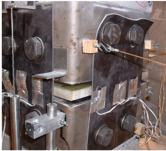
b.) West joint opening and bearing of west fuse plate on bolts
