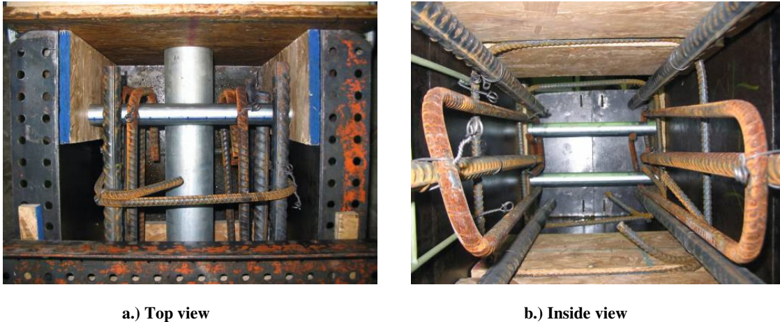
Figure 33. Photographs of lifting inserts.
