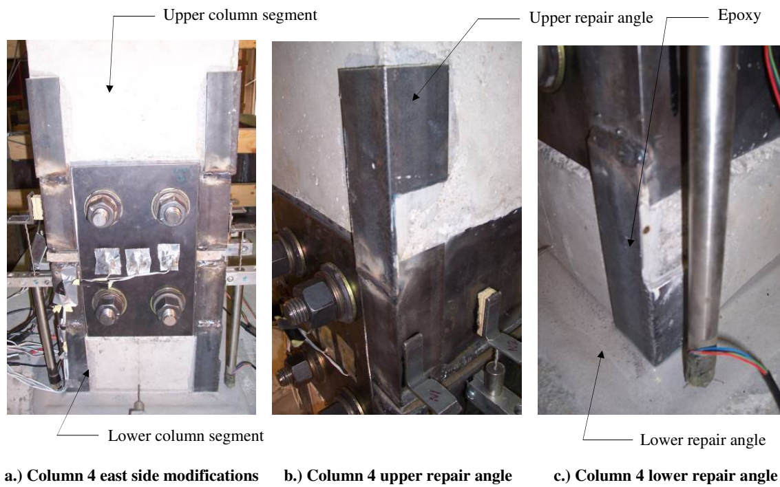
Figure 51. Photographs of Column 4 alterations.
