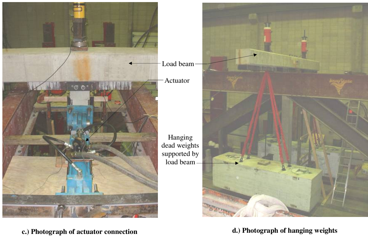
Figure 7. Test setup.
