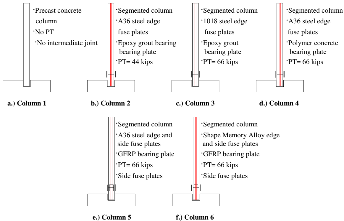
Figure 5. Test columns.
