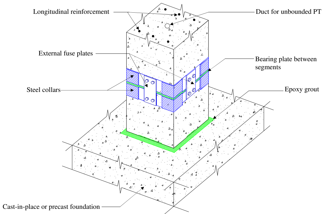
Figure 4. Close-up of typical joints.
