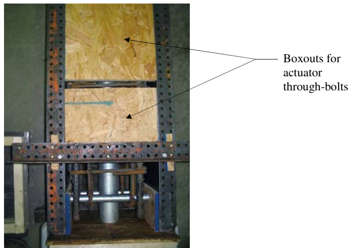
Figure 36. Photograph of top of Column 2.
