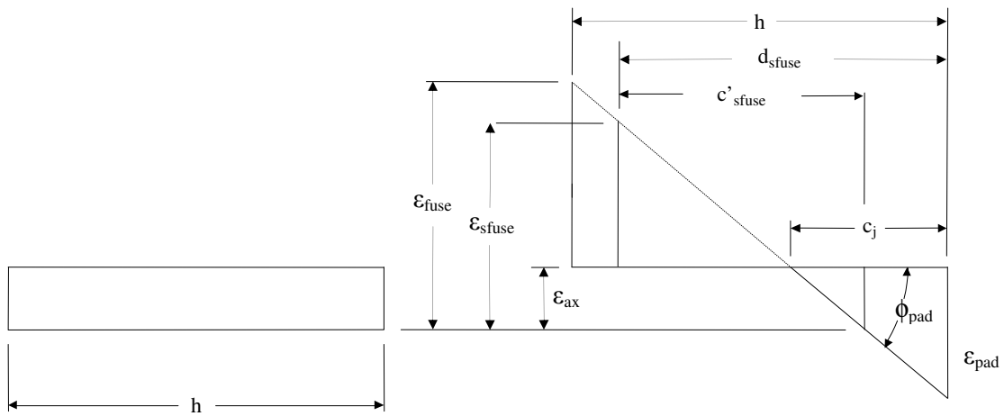
b.) Strain condition at segment joint with axial load only
