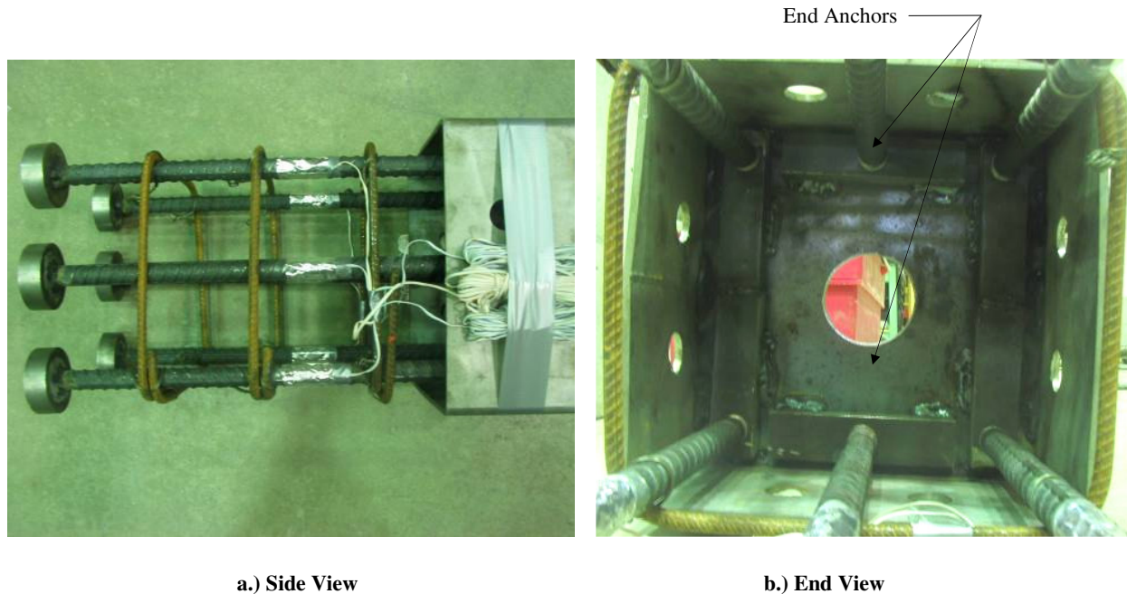
Figure 19. Column 5 mild steel reinforcement in the 2 ft. segment.
