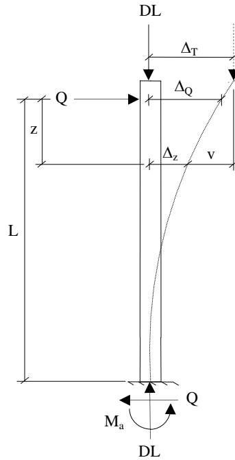
Figure 187. Free body diagram of R/C cantilever with axial and lateral loads.
