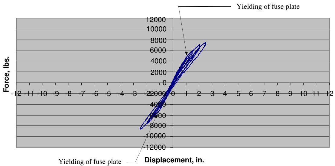
Figure 167. Test 5a load vs. displacement hysteresis.
