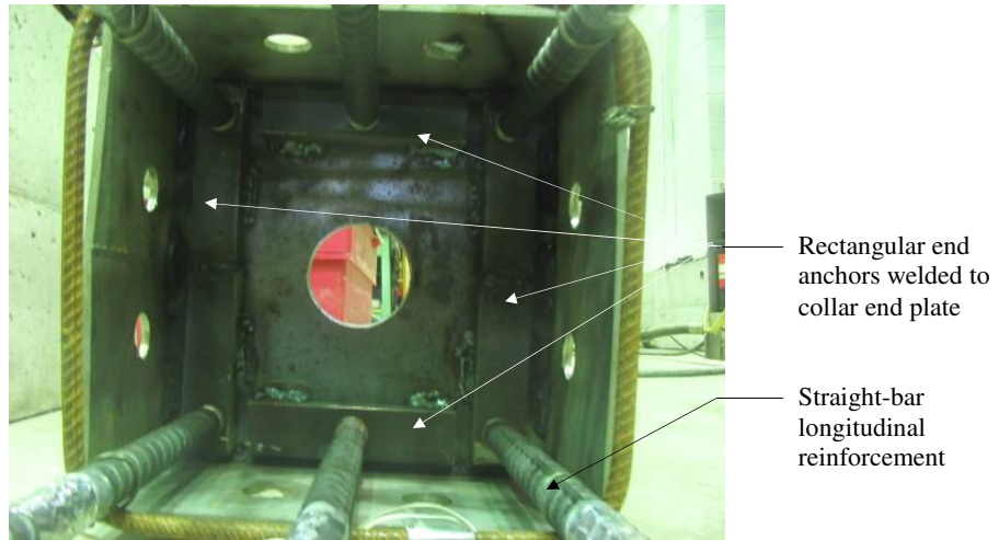
Figure 53. Photograph Column 5 collar reinforcement anchorages.
