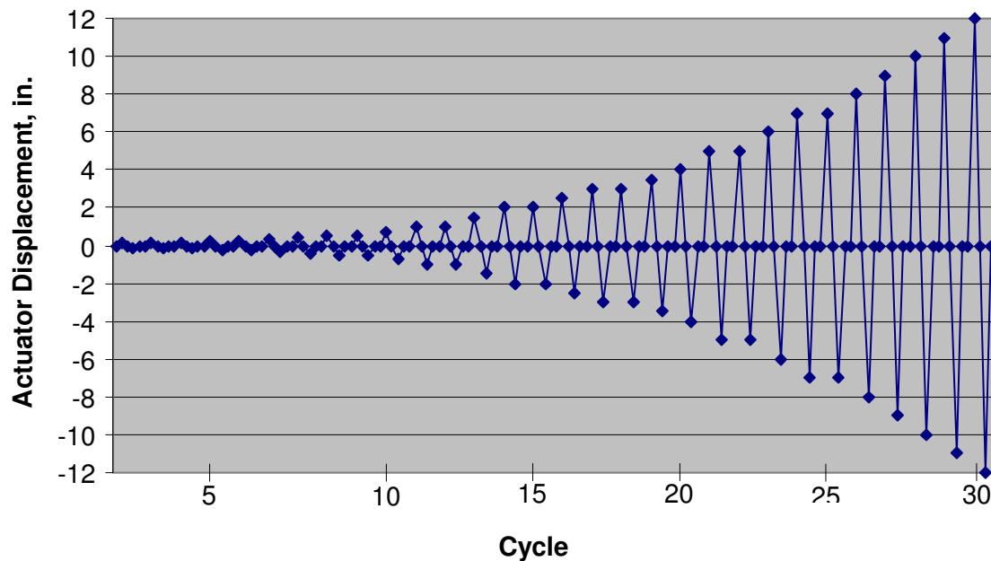
Figure 14. Displacement regimen.
