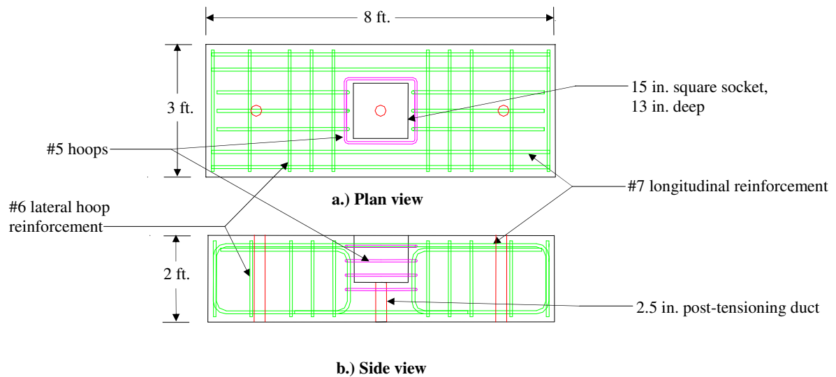
Figure 24. Foundation details.
