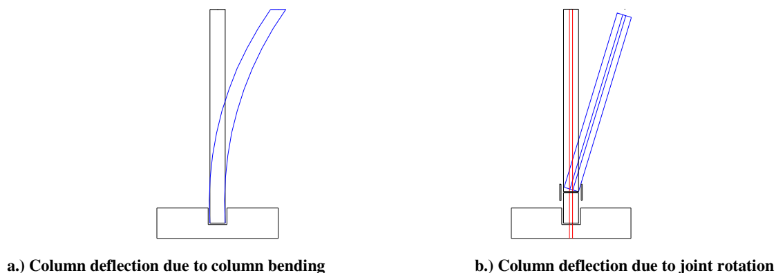
Figure 185. Components of lateral deflection of a jointed column.
