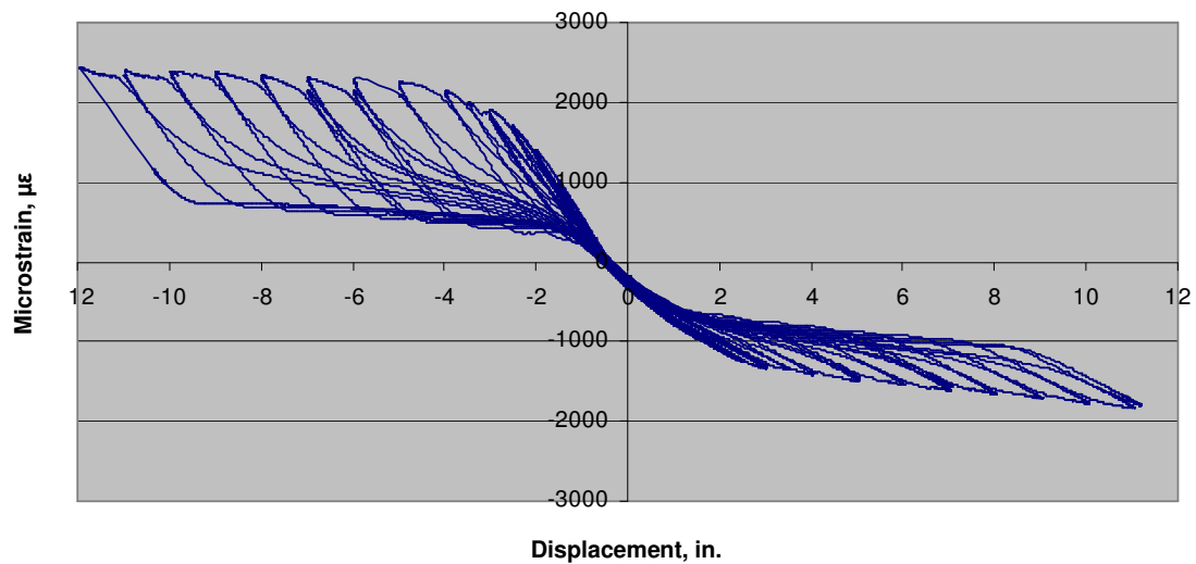
Figure 180. Column 5b upper segment longitudinal reinforcement strain.
