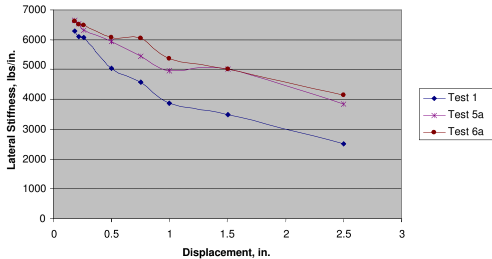
Figure 171. Test “a” lateral stiffness comparisons between Columns 1, 5, and 6.
