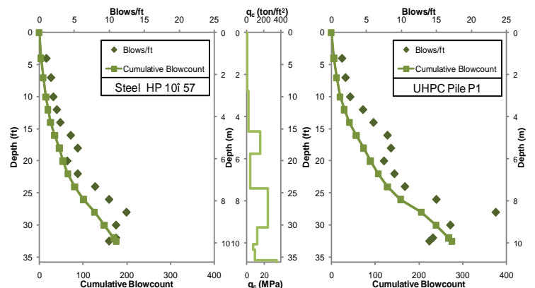
Figure 4. Driving log of blows/ft and cumulative blow count.
