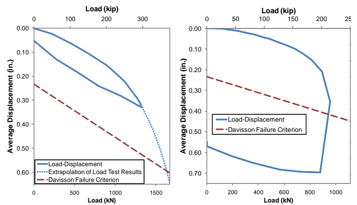
Figure 6. Vertical load-displacement behavior for UHPC pile P1 (left) and the steel pile (right). The Davisson criterion (dashed line) was used to determine the capacity of each pile.
