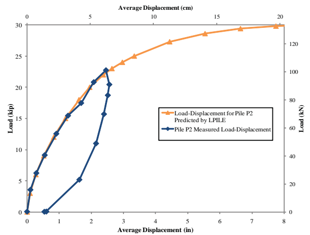
Figure 7. Measured lateral load-displacement behavior of UHPC pile P2 compared with calculated response using LPILE.
