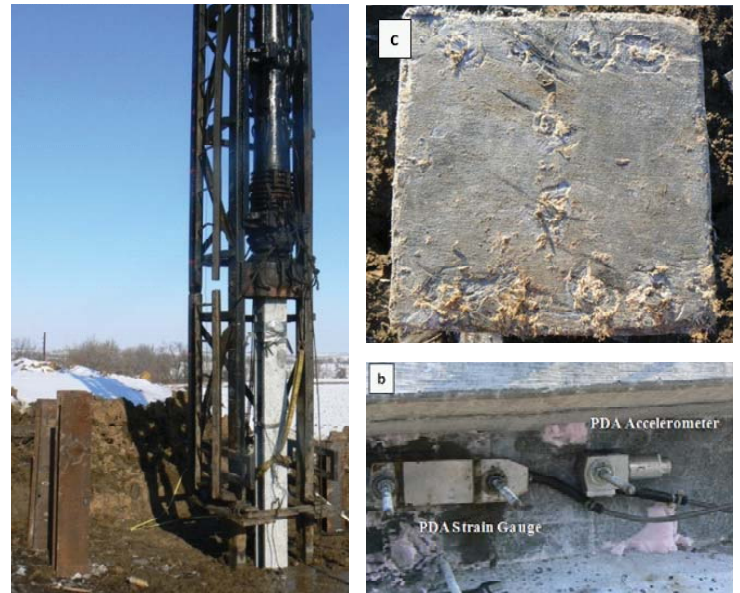
Figure 2. Pile driving hammer (left), UHPC pile head after driving (top right), strain gages and accelerometers (bottom right).
