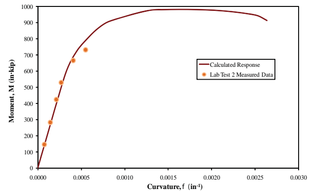
Figure 9. Calculated and measured moment-curvature response of a \frac{3}{4} -scale UHPC laboratory test unit.
