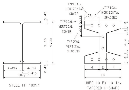
Figure 1. Steel HP 10x57 pile (left) and 10 by 10 in. tapered H-shaped section (right). The HP 10x57 section is commonly used by many states.
