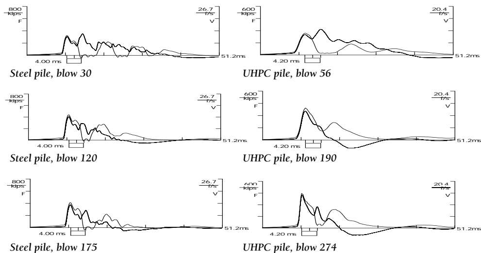
Figure 3. Force and velocity PDA diagrams for both piles during easy driving at 15 ft (top row), hard driving at 27.5 ft (middle row), and final depth at 32.5 ft (bottom row).
