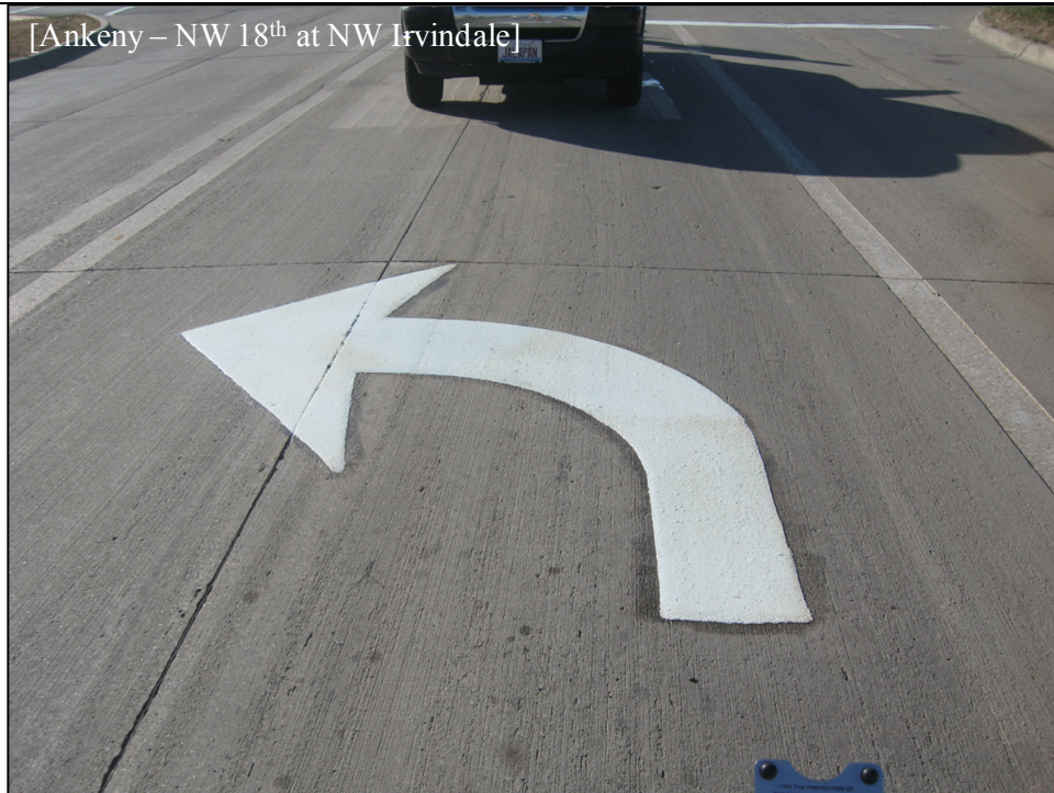
October 2008 – Urban Left Turn Arrow Installation ( R_L=429 ), on concrete.
