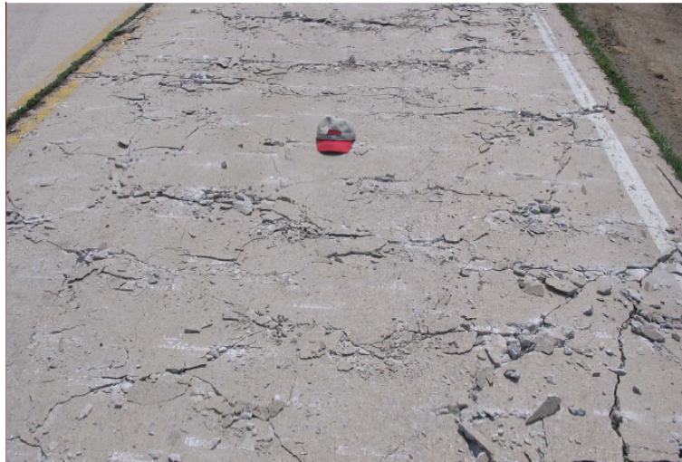
Figure 6. Modified Rubblization Method proposed by Antigo (Jansen, 2006)
